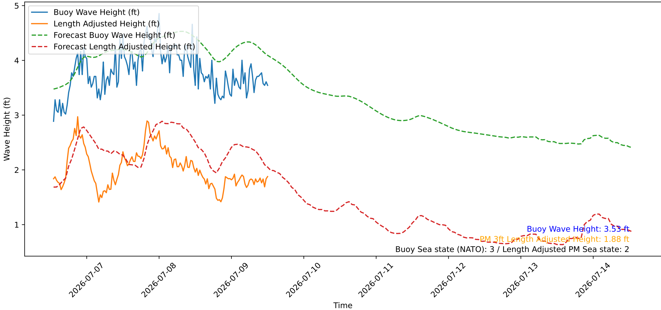
Wave Heights over Time for Red Beach at 2026-07-09 12:40:46
