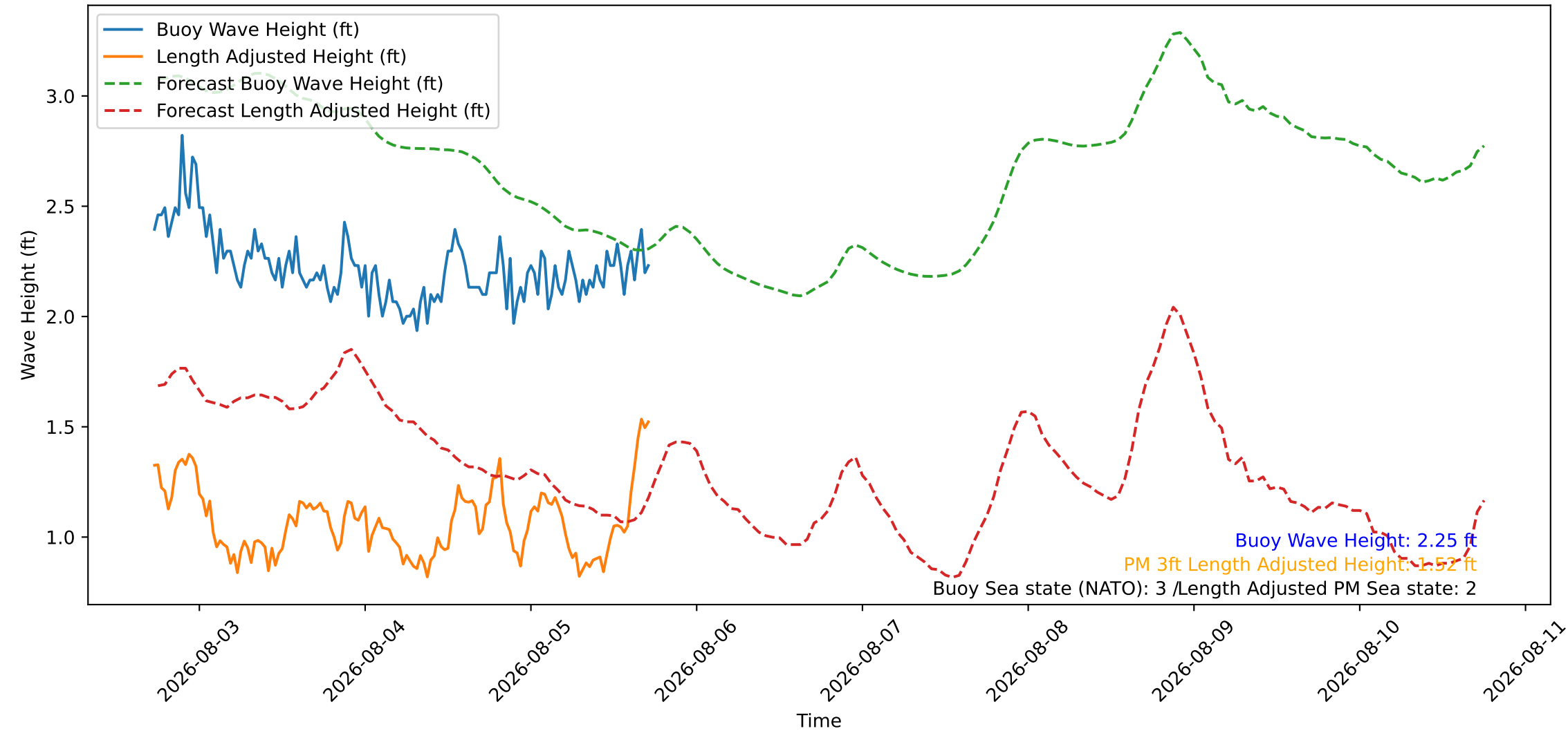
Wave Heights over Time for Green Beach at 2026-08-05 17:41:08
