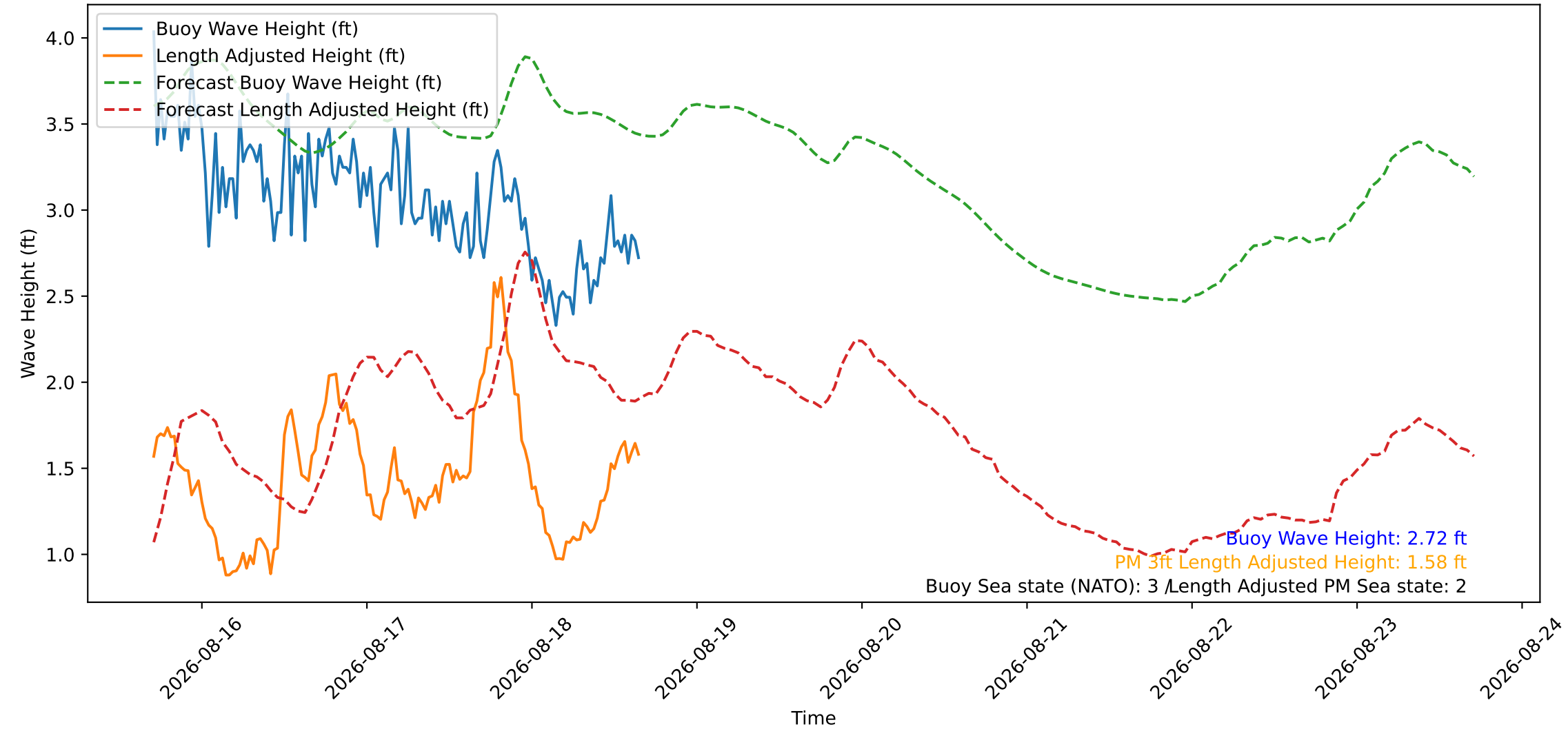
Wave Heights over Time for Red Beach at 2026-08-18 16:50:47
