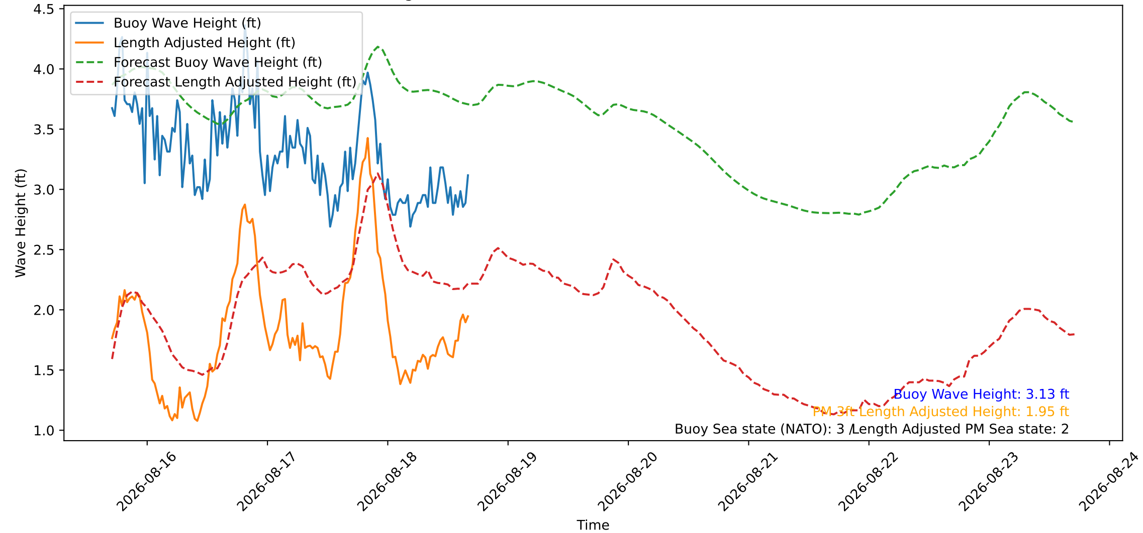
Wave Heights over Time for Green Beach at 2026-08-18 16:51:12
