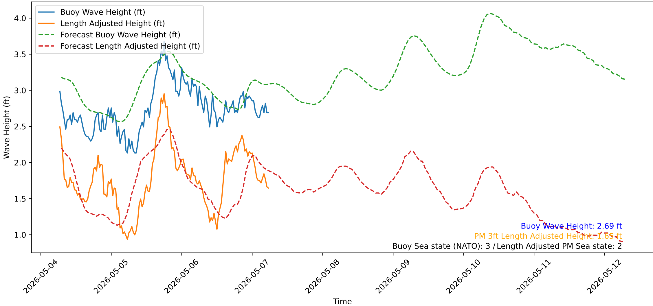
Wave Heights over Time for Green Beach at 2026-05-07 06:31:12
