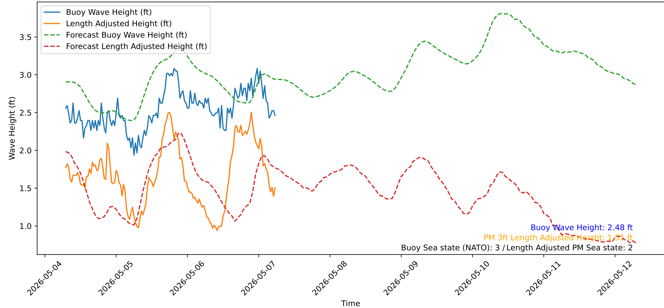
Wave Heights over Time for Red Beach at 2026-05-07 06:30:50
