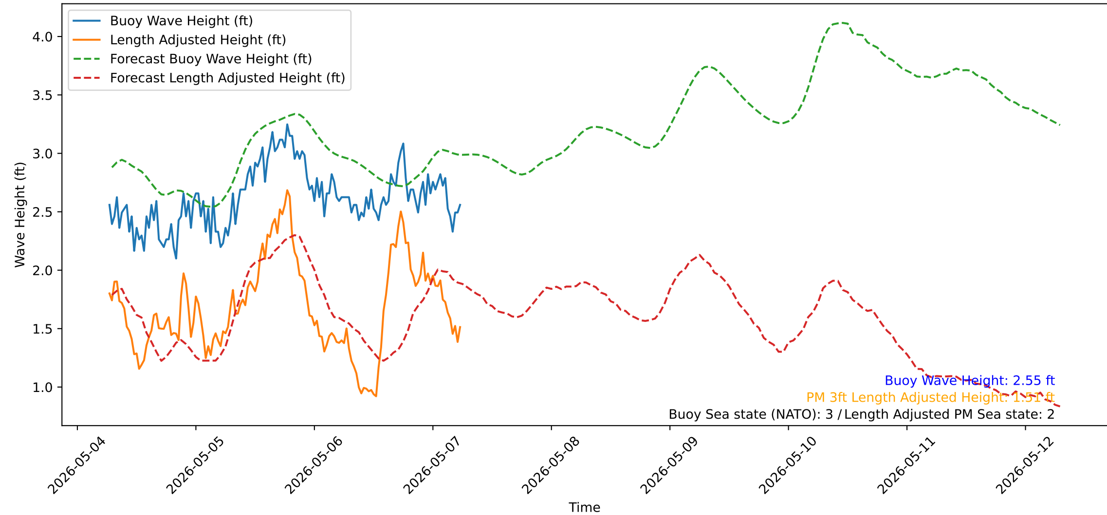
Wave Heights over Time for Oceanside Harbor at 2026-05-07 06:30:31
