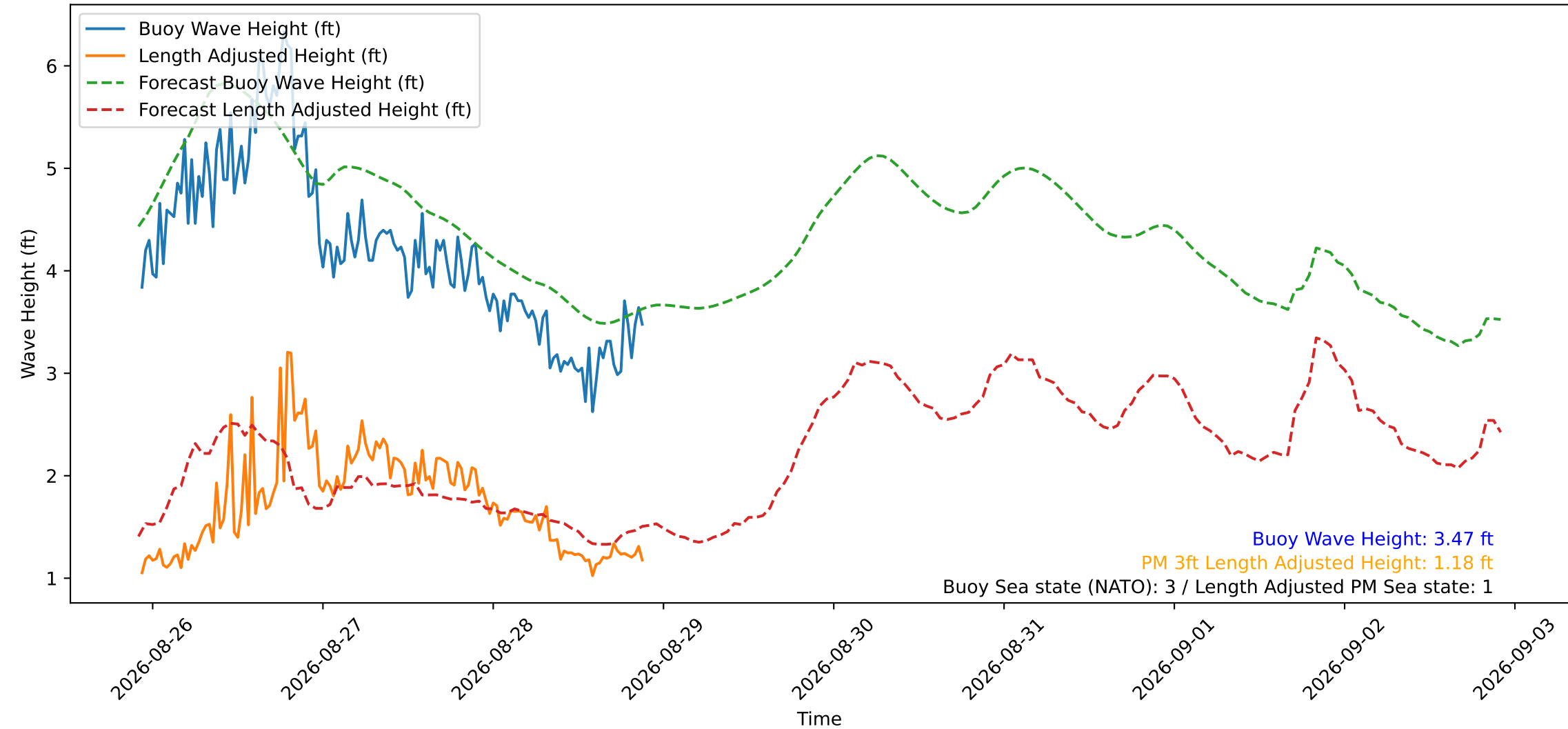
Wave Heights over Time for Green Beach at 2026-08-28 22:01:11
