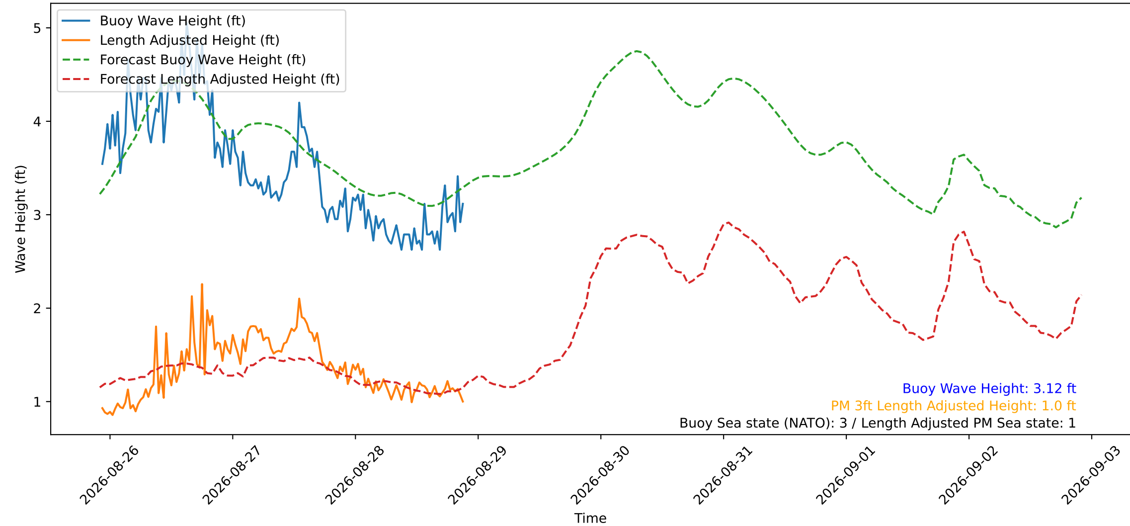
Wave Heights over Time for Red Beach at 2026-08-28 22:00:48
