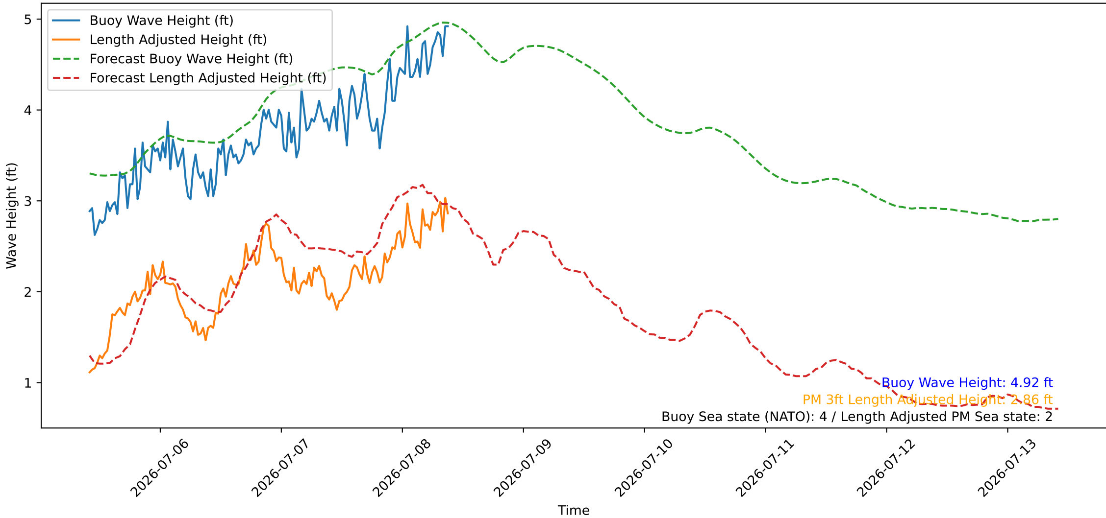
Wave Heights over Time for Oceanside Harbor at 2026-07-08 09:50:26
