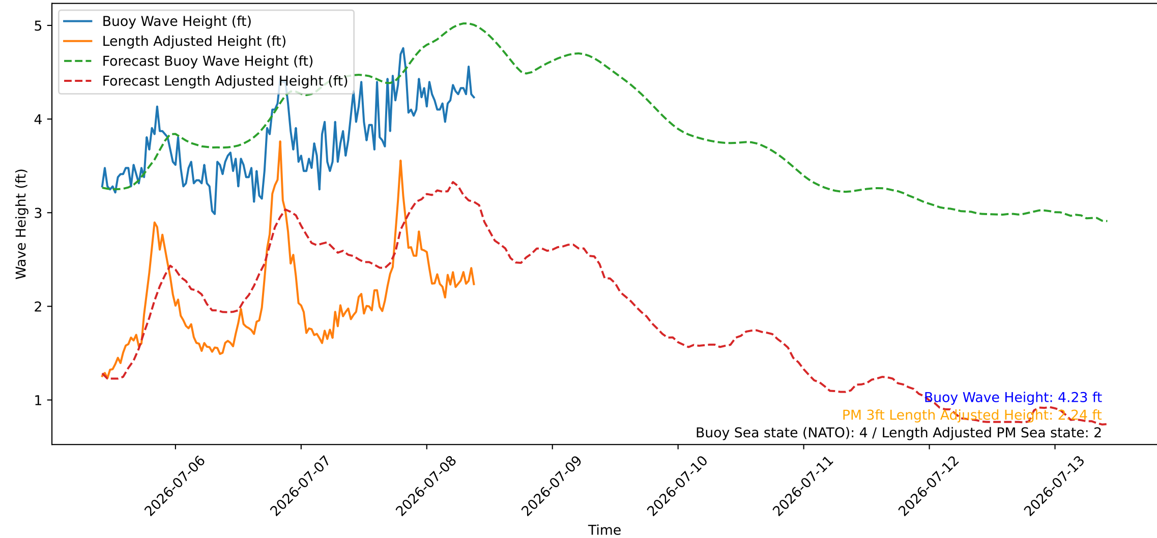
Wave Heights over Time for Green Beach at 2026-07-08 09:51:09
