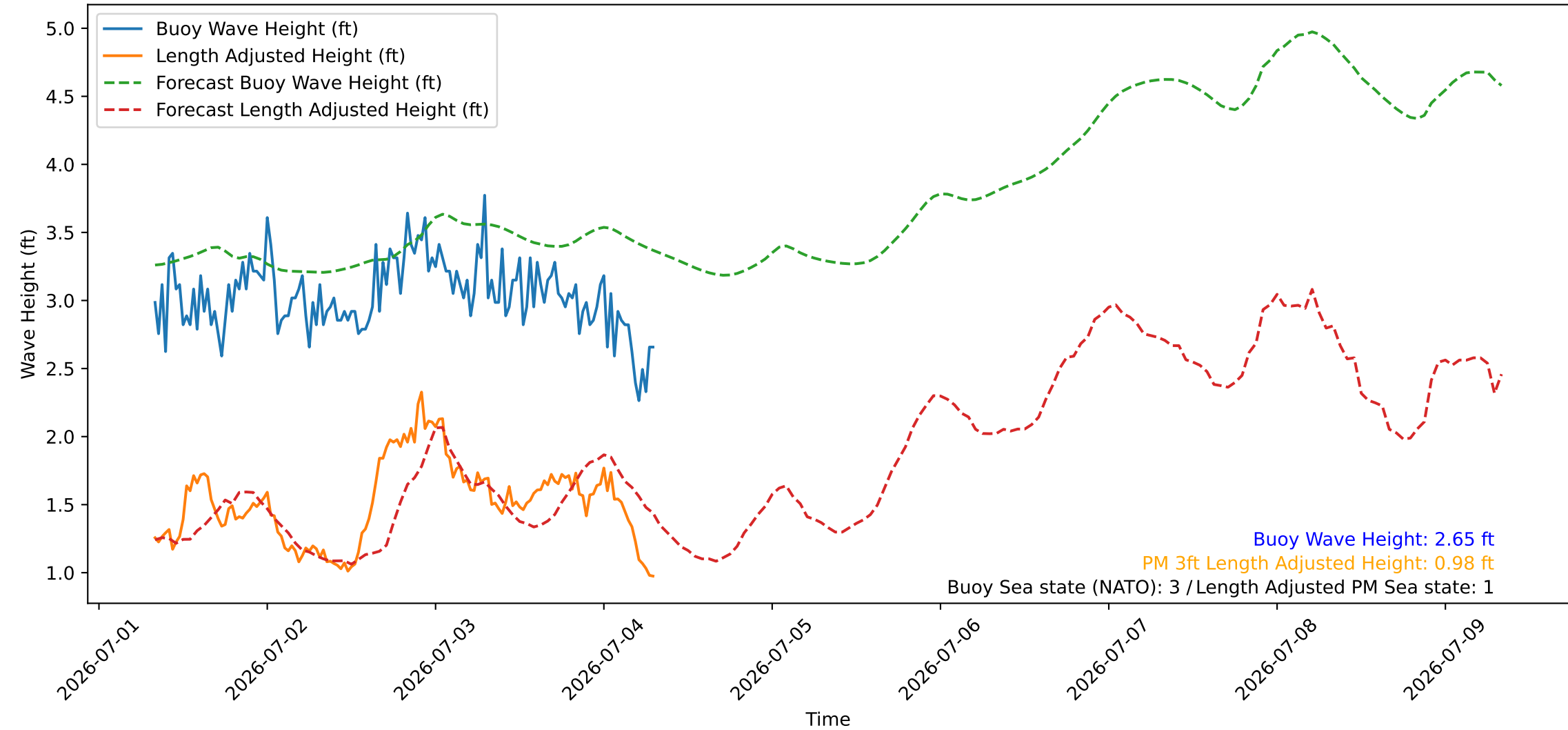
Wave Heights over Time for Oceanside Harbor at 2026-07-04 07:50:26
