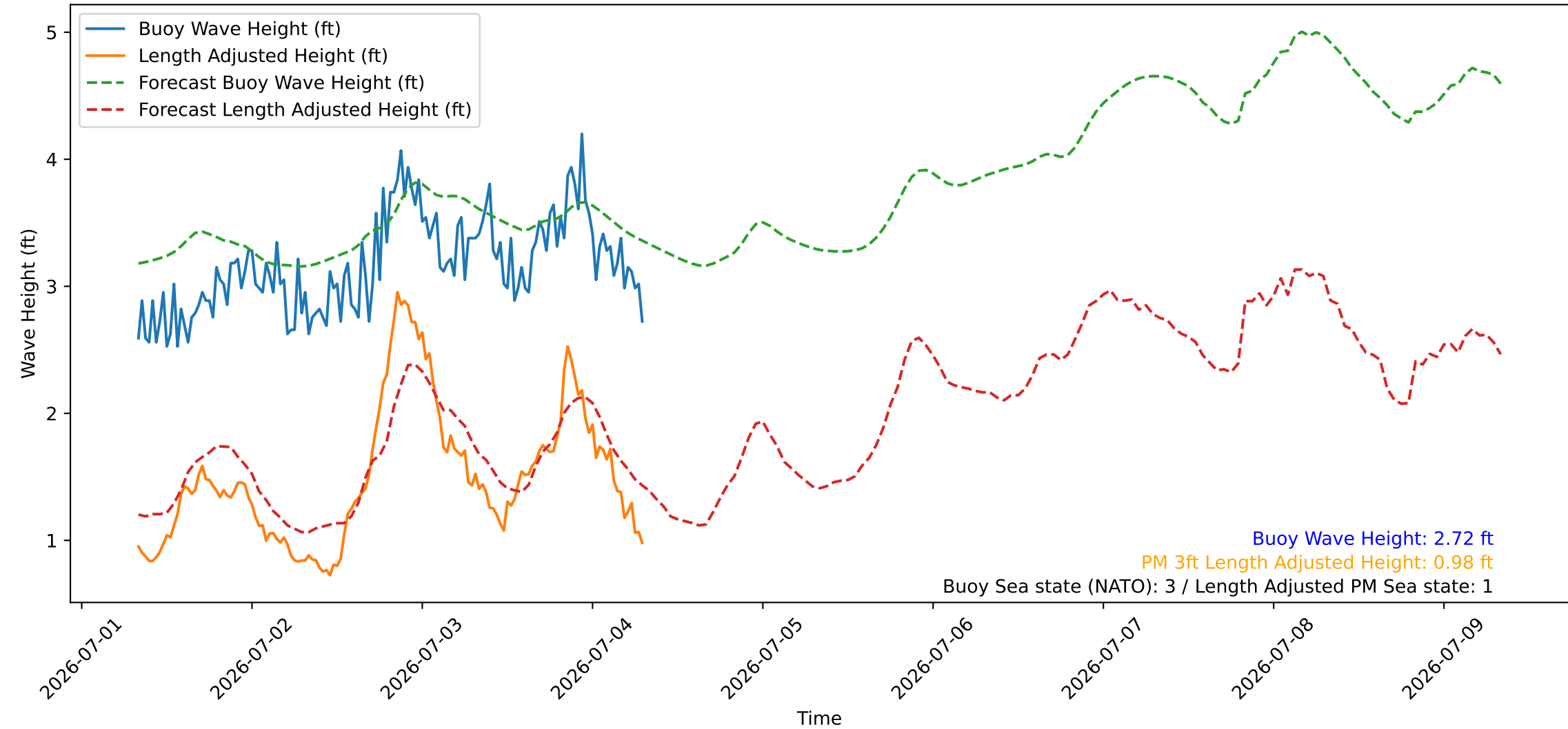
Wave Heights over Time for Green Beach at 2026-07-04 07:51:10
