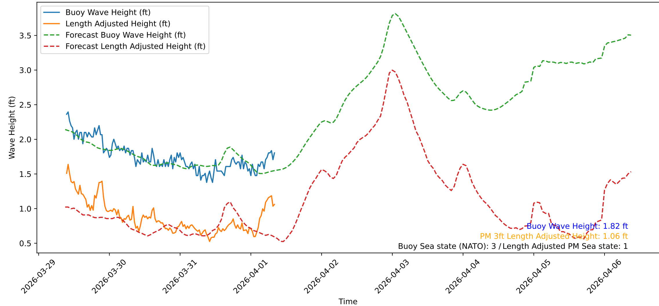
Wave Heights over Time for Red Beach at 2026-04-01 09:00:49
