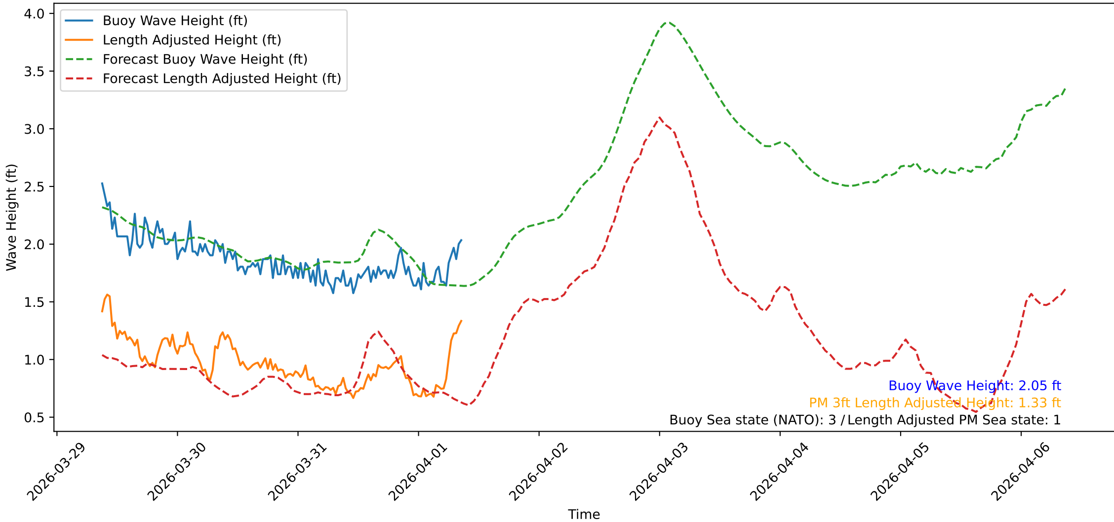
Wave Heights over Time for Oceanside Harbor at 2026-04-01 09:00:32
