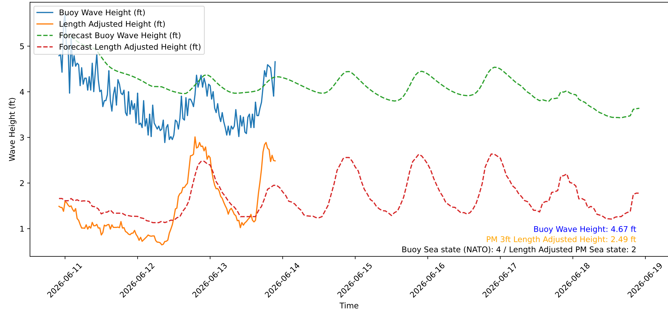
Wave Heights over Time for Green Beach at 2026-06-13 22:11:09
