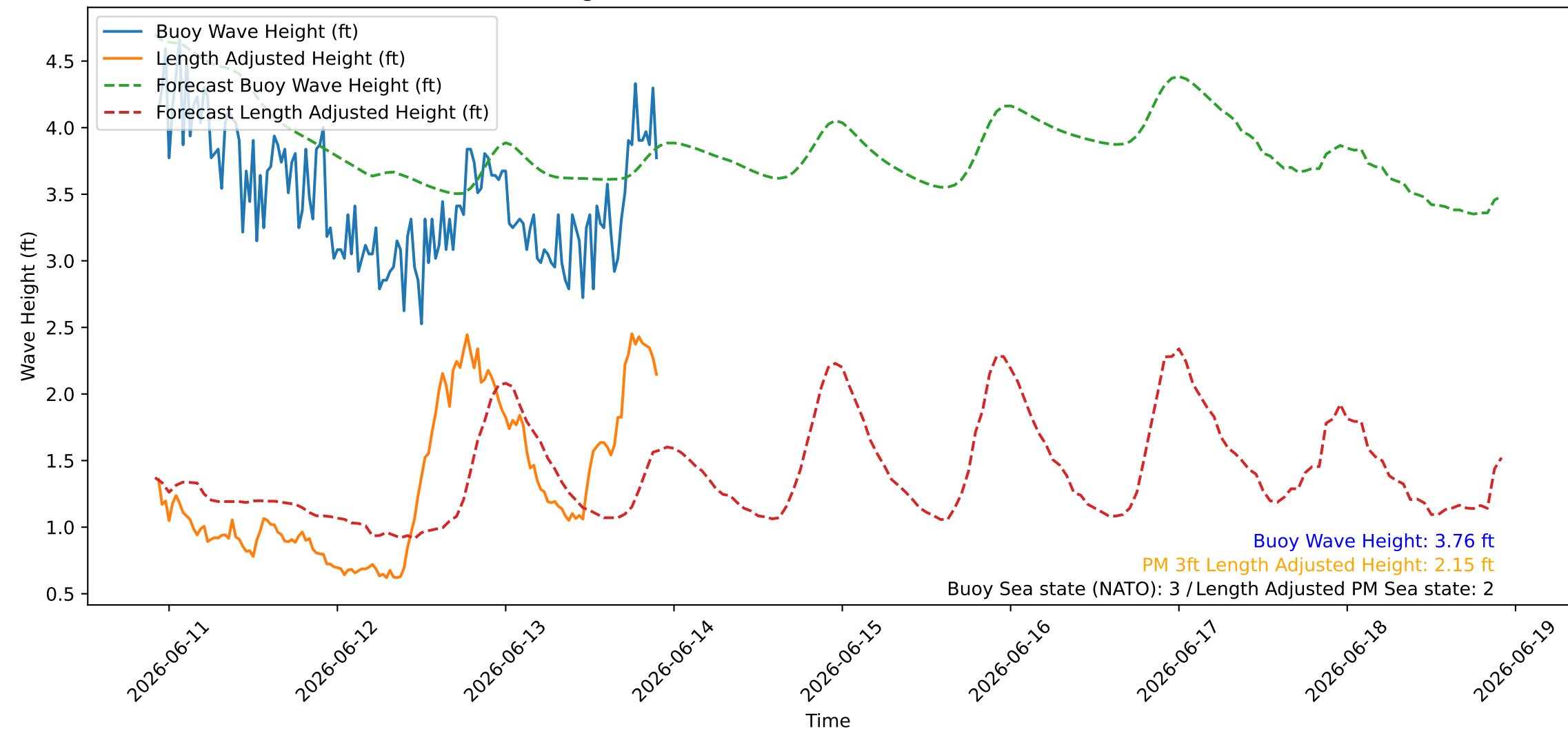
Wave Heights over Time for Red Beach at 2026-06-13 22:10:46
