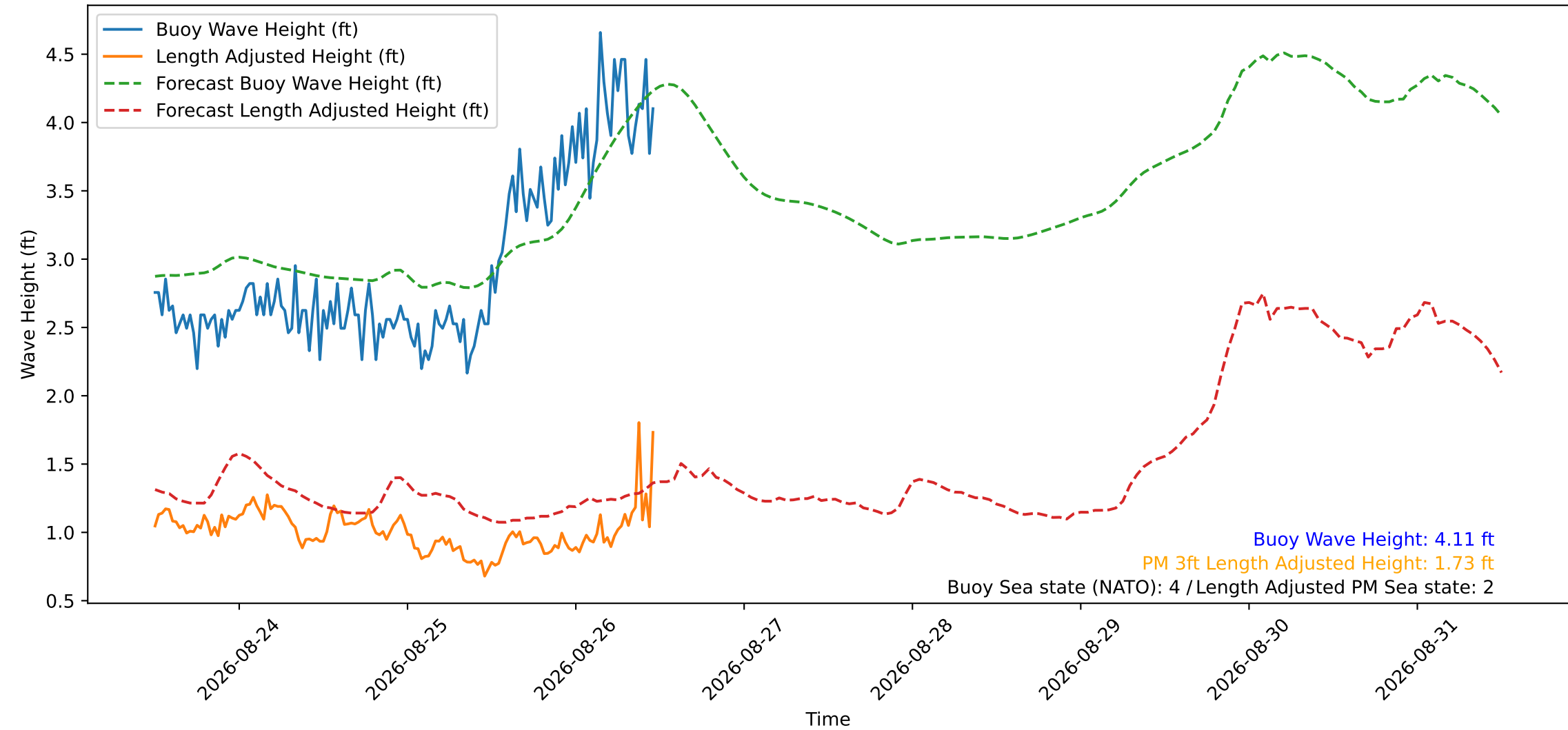
Wave Heights over Time for Red Beach at 2026-08-26 11:40:49
