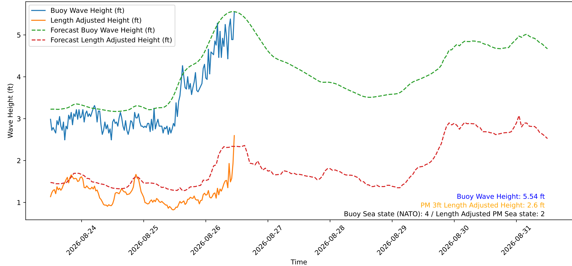
Wave Heights over Time for Green Beach at 2026-08-26 11:41:12
