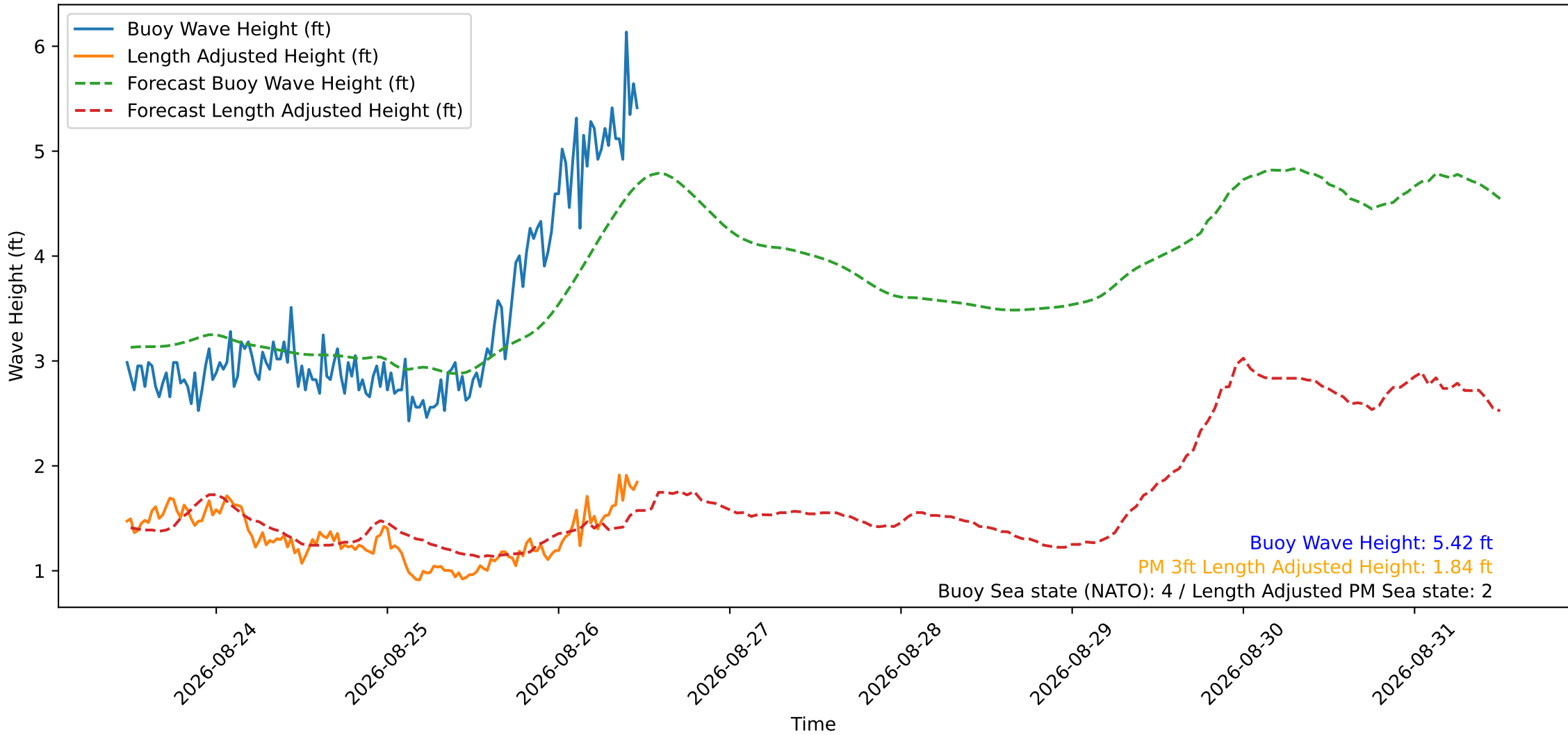
Wave Heights over Time for Oceanside Harbor at 2026-08-26 11:40:29
