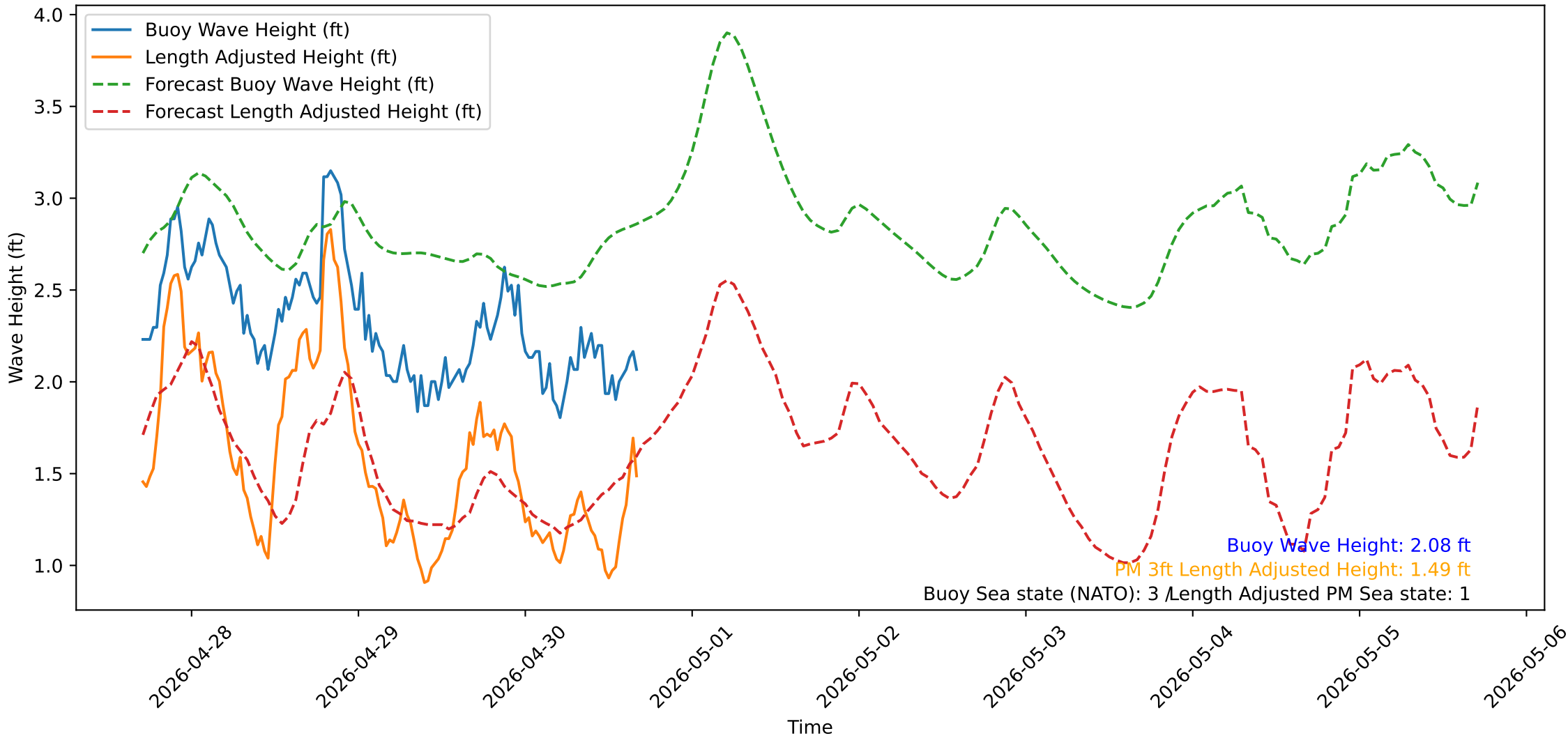
Wave Heights over Time for Green Beach at 2026-04-30 16:51:14
