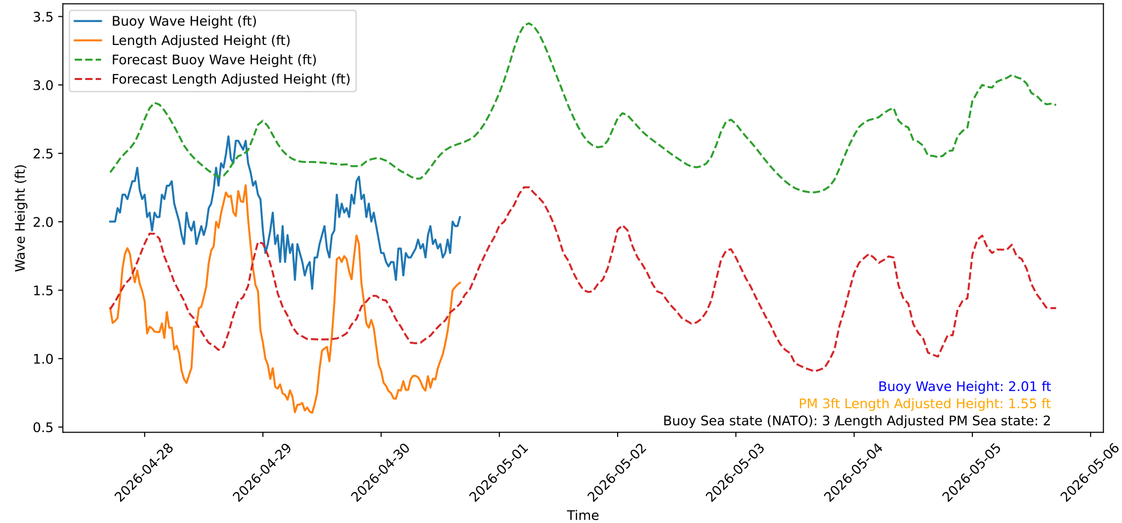
Wave Heights over Time for Red Beach at 2026-04-30 16:50:52
