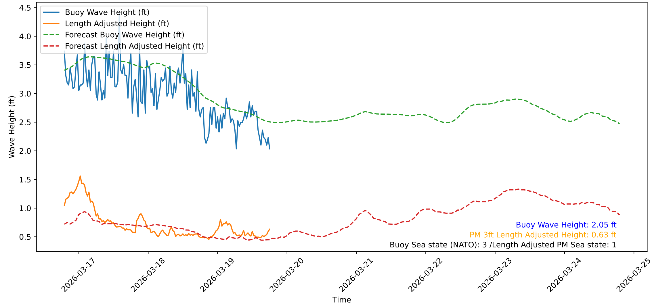
Wave Heights over Time for Oceanside Harbor at 2026-03-19 18:50:32
