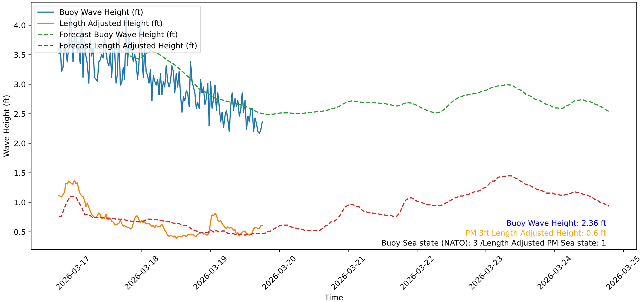
Wave Heights over Time for Green Beach at 2026-03-19 18:51:10
