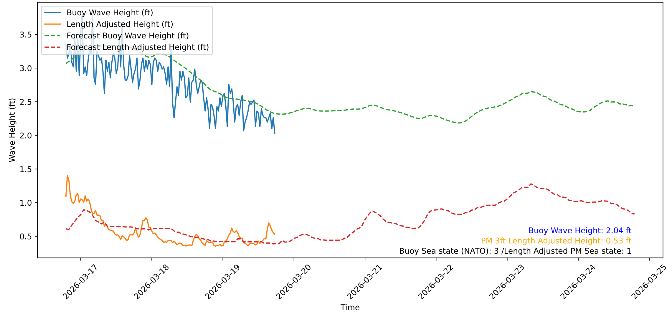
Wave Heights over Time for Red Beach at 2026-03-19 18:50:48
