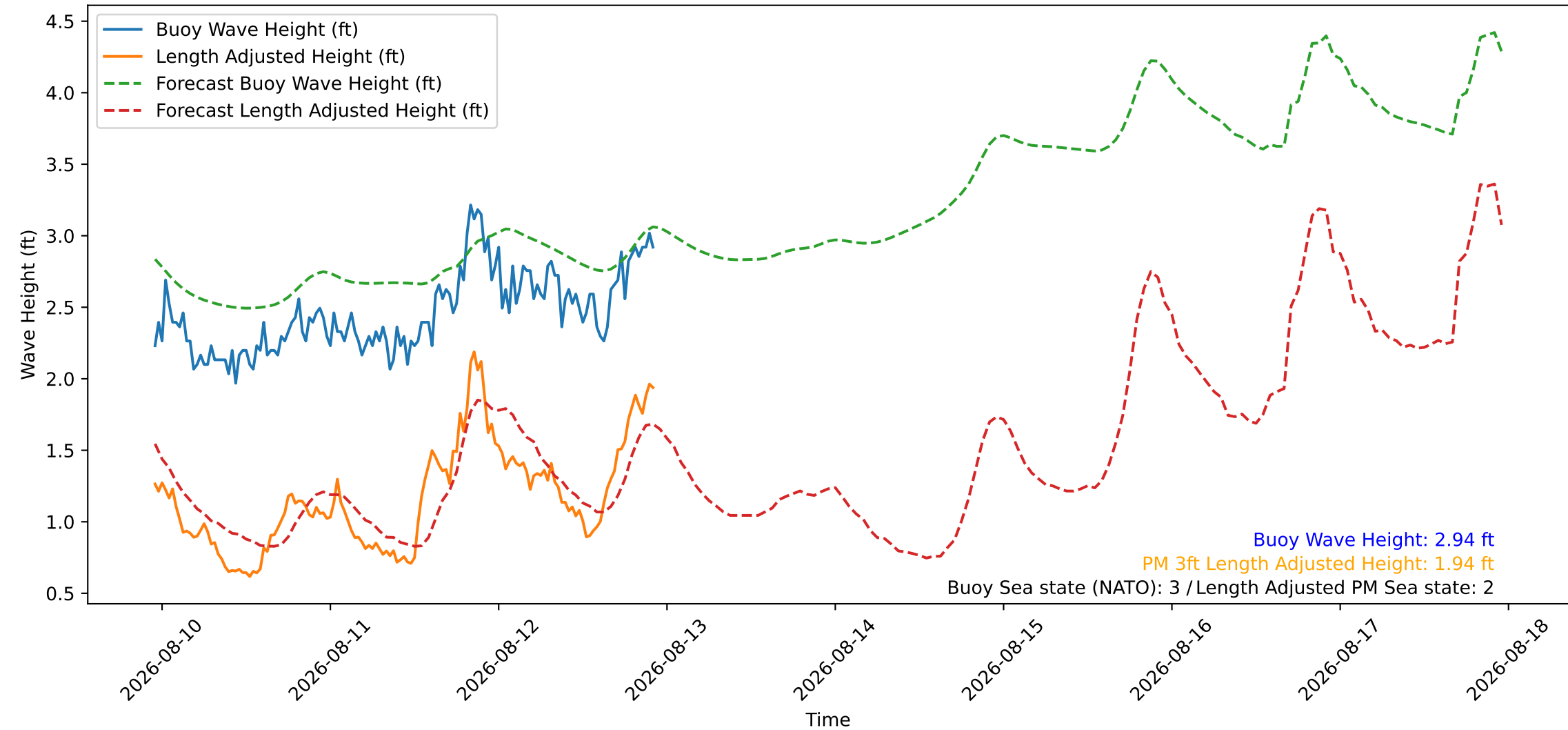
Wave Heights over Time for Green Beach at 2026-08-12 23:01:07
