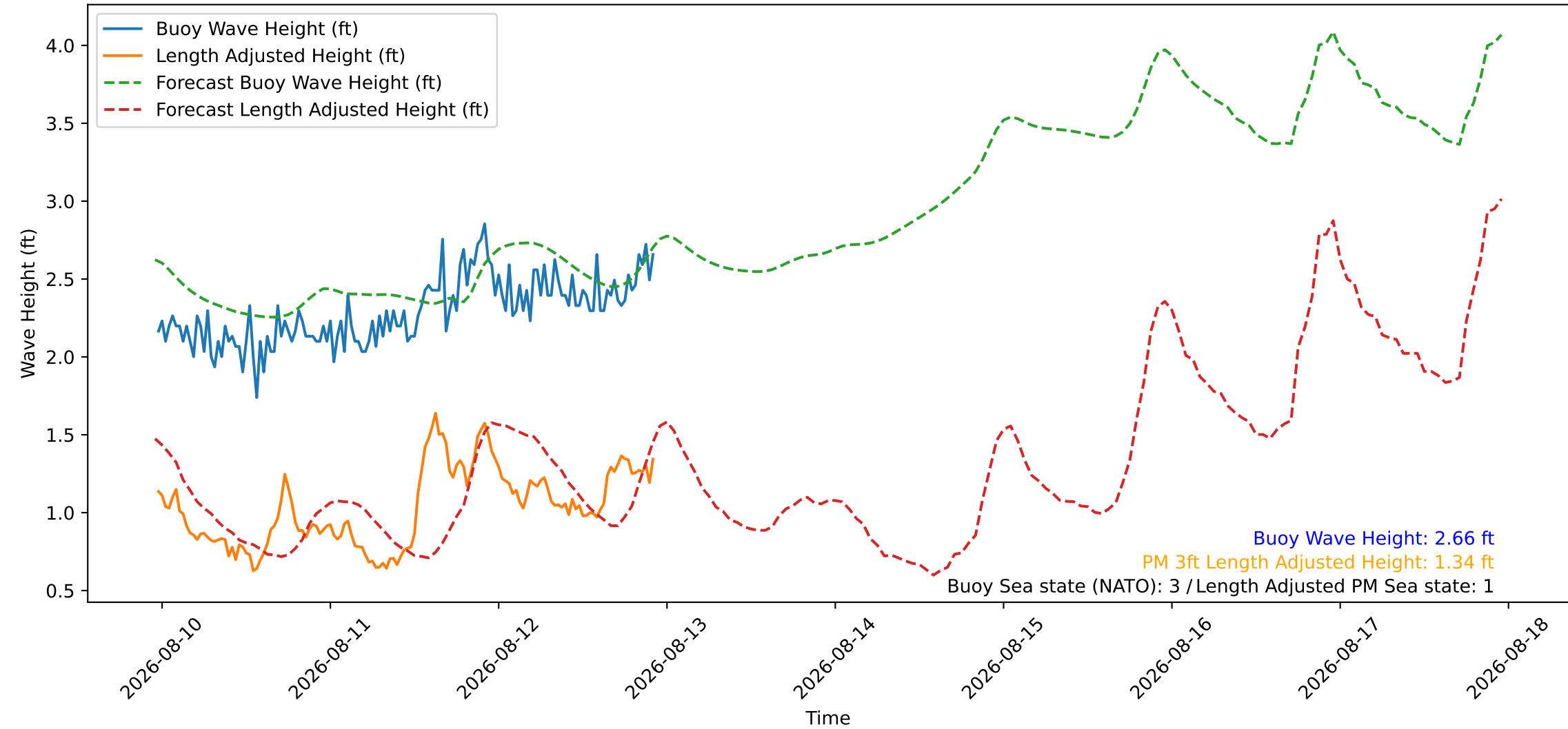
Wave Heights over Time for Red Beach at 2026-08-12 23:00:45
