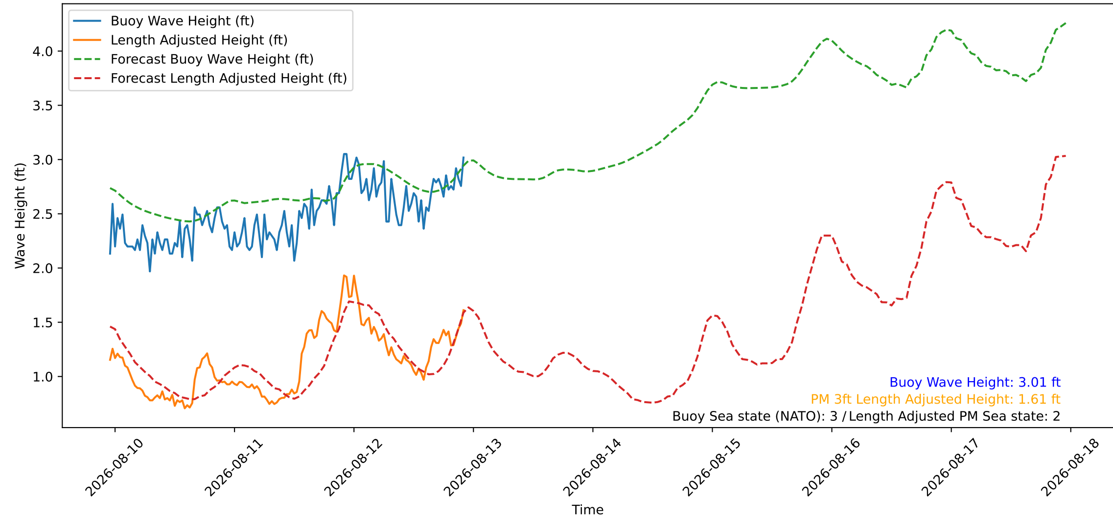
Wave Heights over Time for Oceanside Harbor at 2026-08-12 23:00:26
