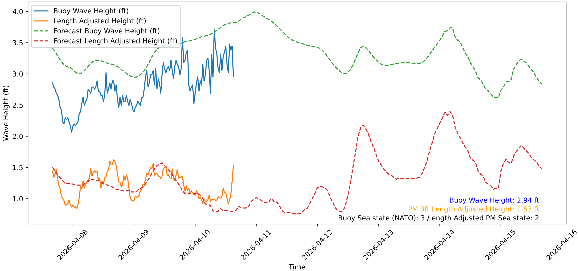
Wave Heights over Time for Red Beach at 2026-04-10 15:40:51
