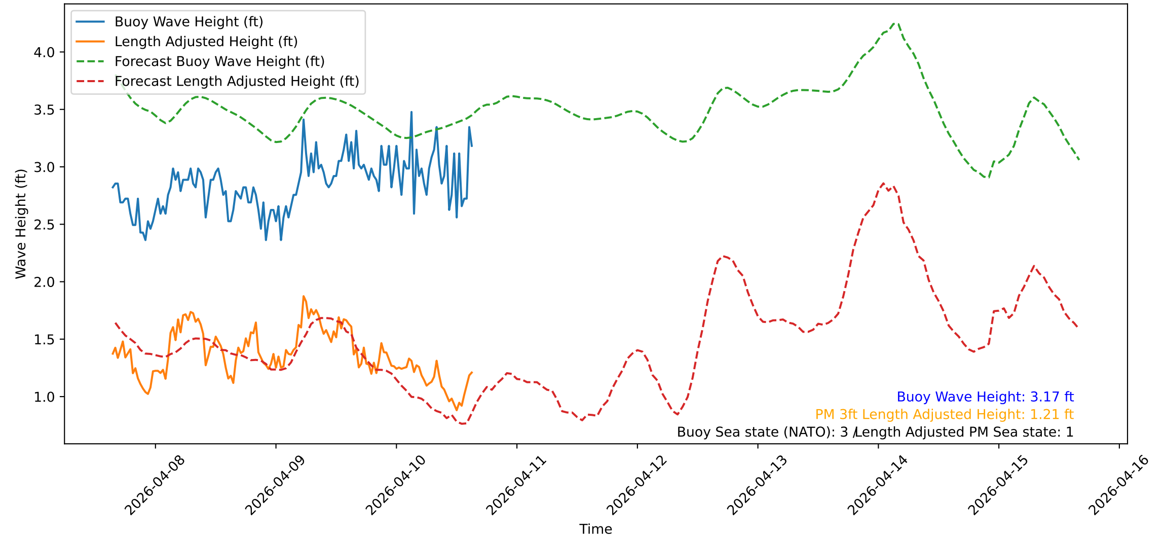
Wave Heights over Time for Green Beach at 2026-04-10 15:41:13
