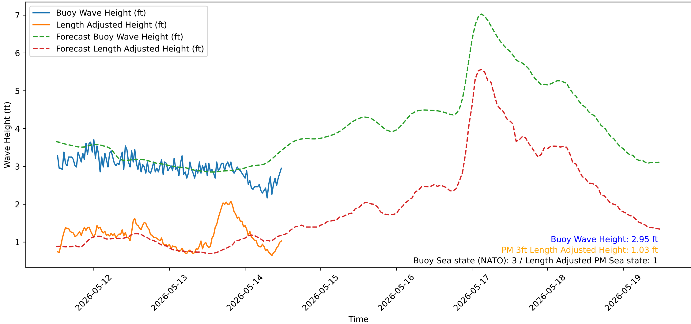
Wave Heights over Time for Oceanside Harbor at 2026-05-14 12:20:32
