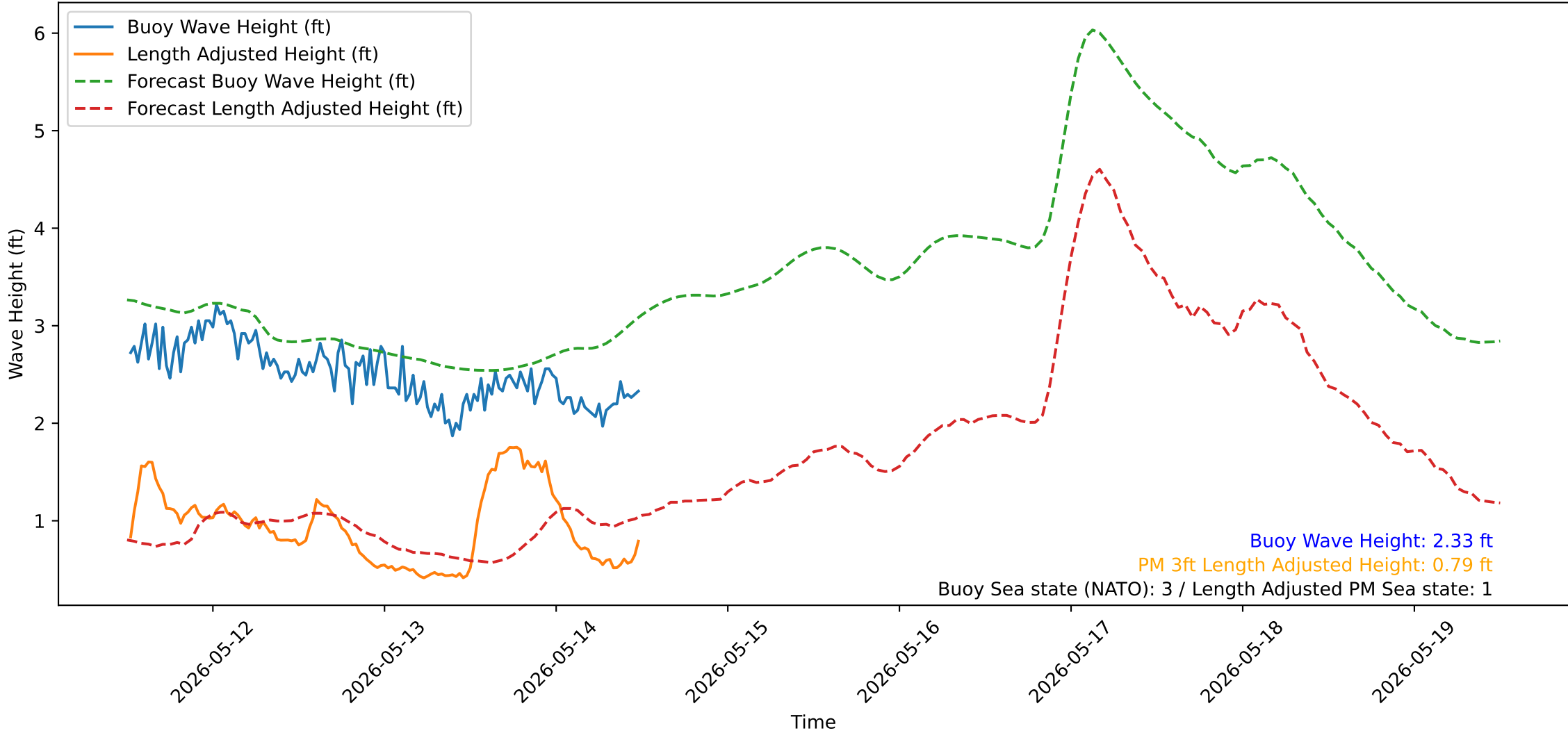
Wave Heights over Time for Red Beach at 2026-05-14 12:20:52
