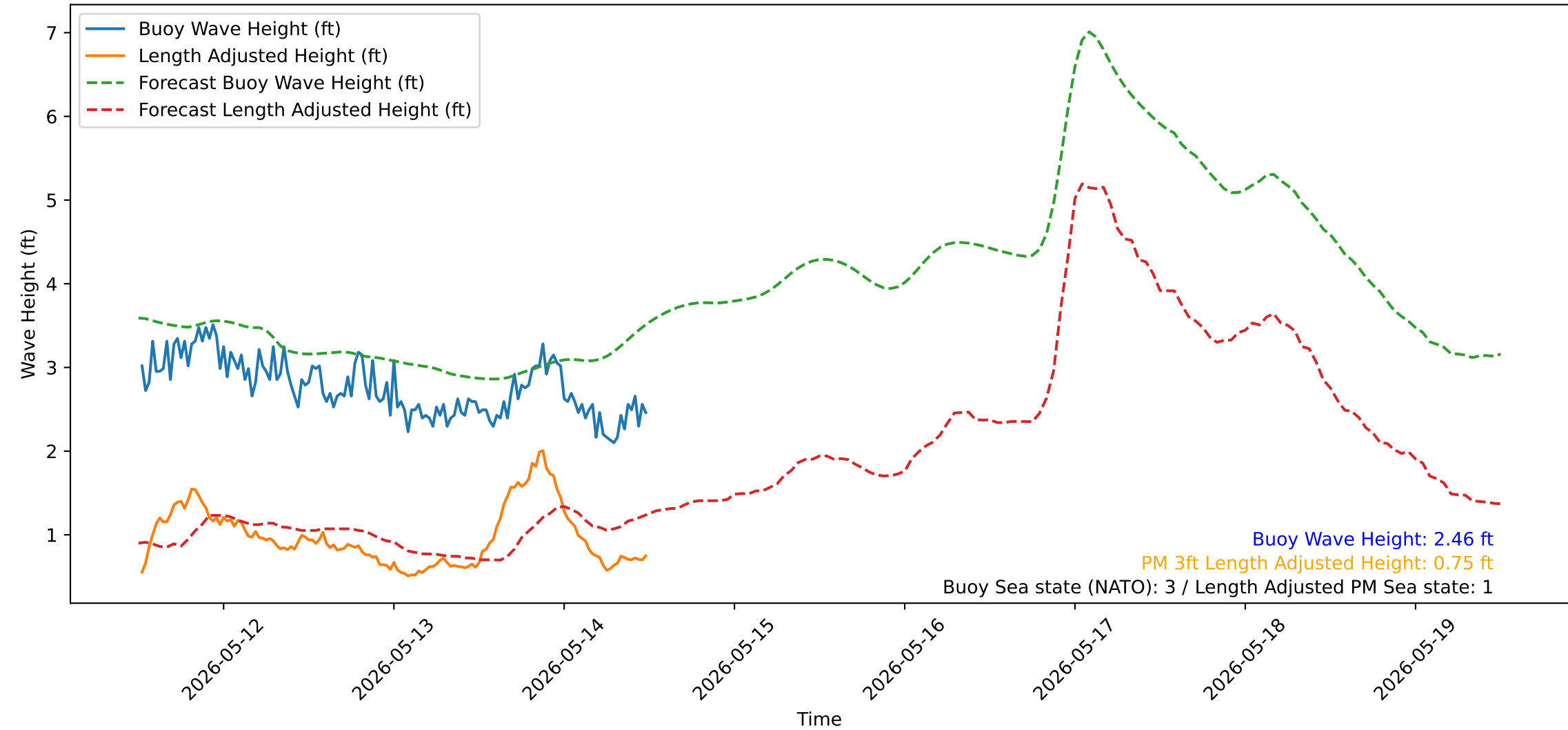
Wave Heights over Time for Green Beach at 2026-05-14 12:21:16
