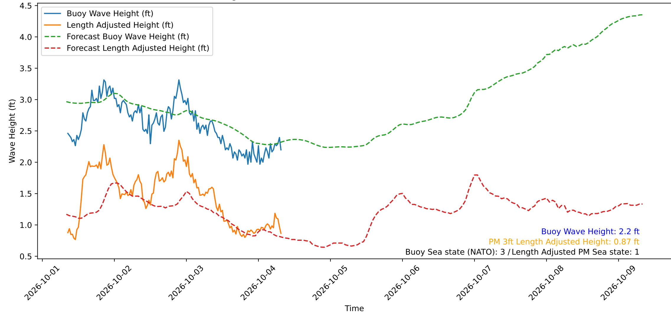
Wave Heights over Time for Oceanside Harbor at 2026-10-04 08:20:29
