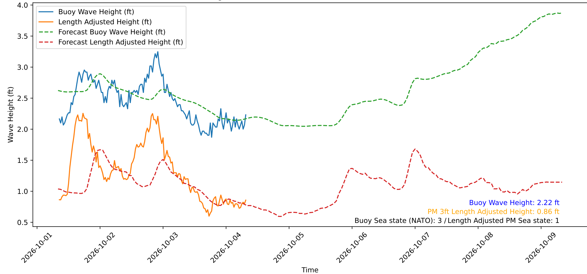
Wave Heights over Time for Red Beach at 2026-10-04 08:20:50
