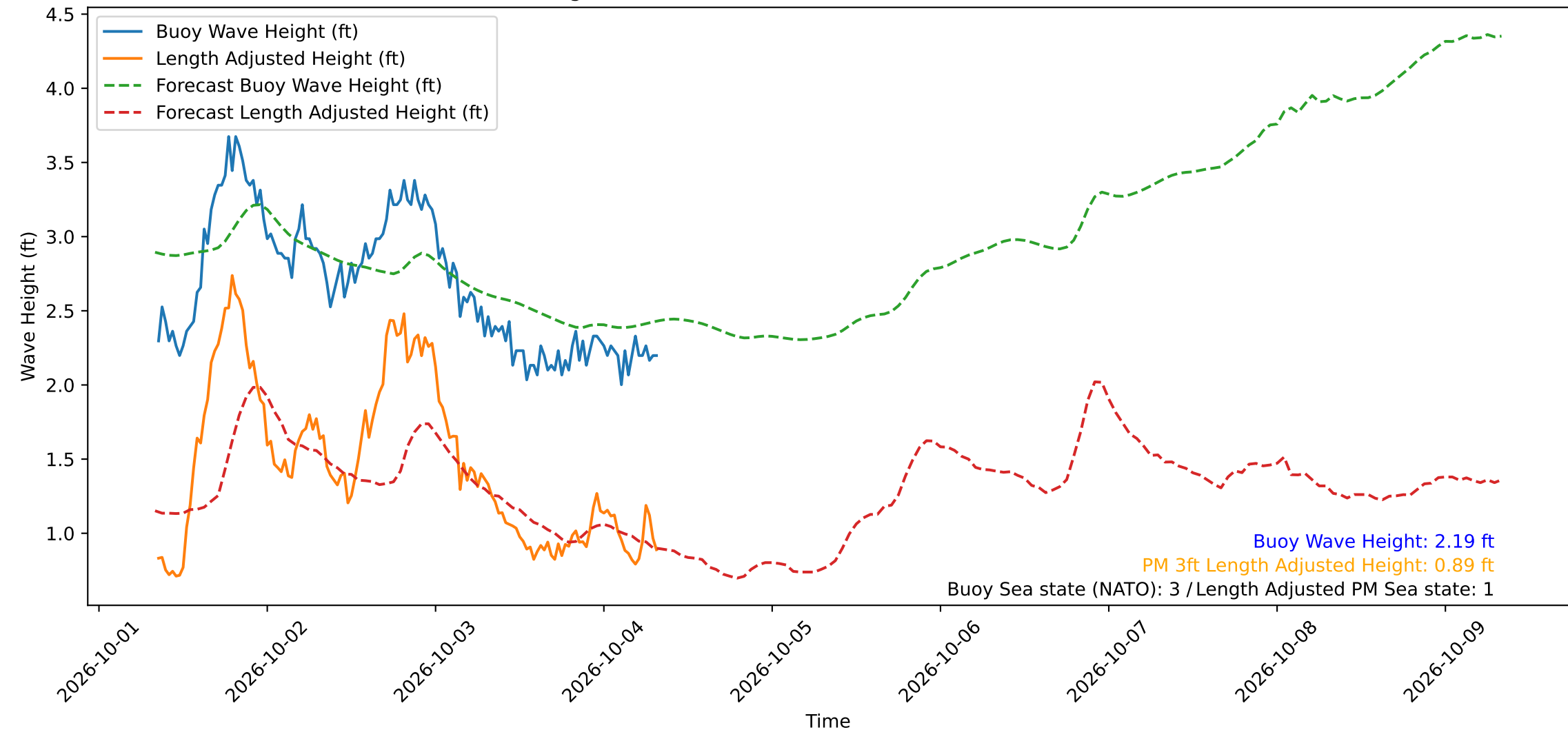
Wave Heights over Time for Green Beach at 2026-10-04 08:21:15
