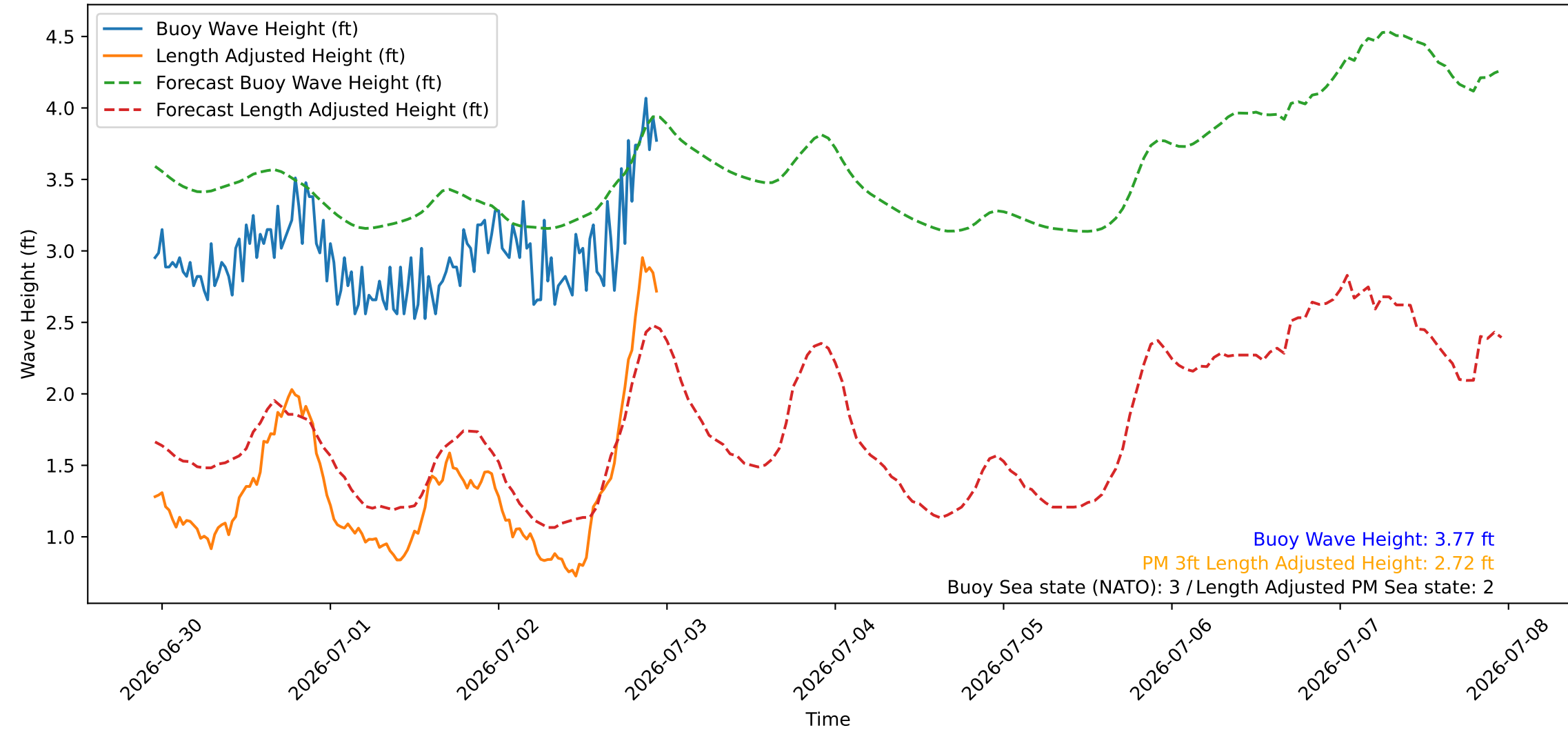
Wave Heights over Time for Green Beach at 2026-07-02 23:11:07
