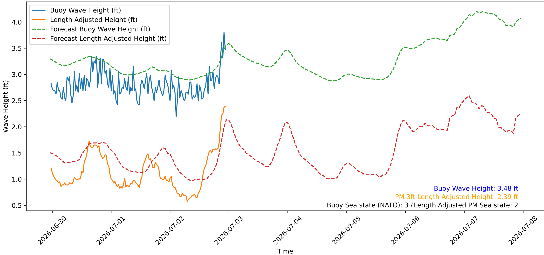
Wave Heights over Time for Red Beach at 2026-07-02 23:10:45
