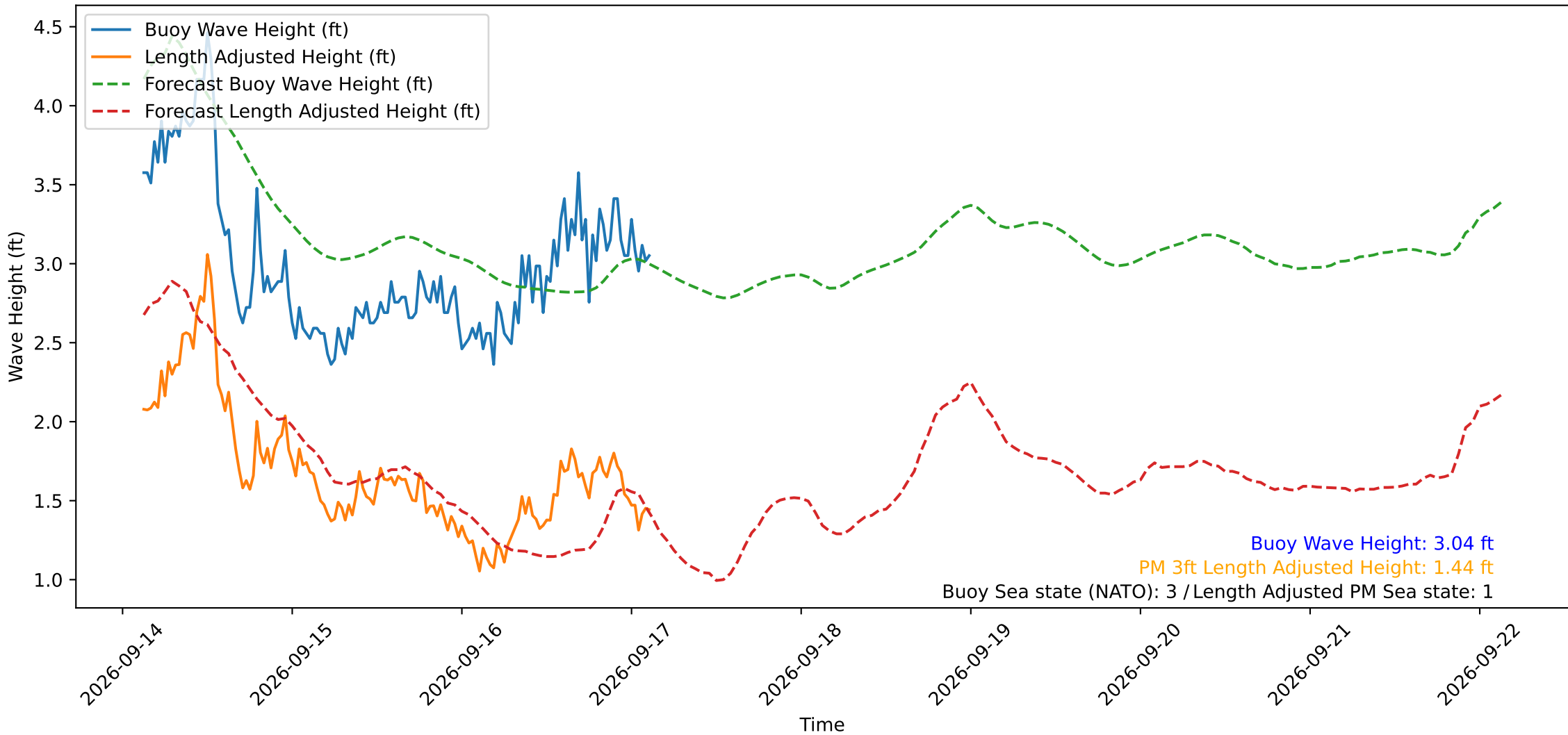
Wave Heights over Time for Oceanside Harbor at 2026-09-17 03:10:29
