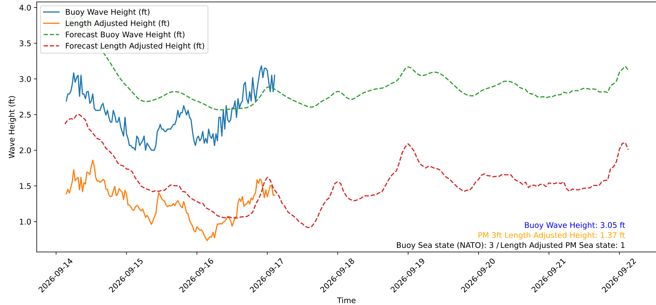
Wave Heights over Time for Red Beach at 2026-09-17 03:10:48
