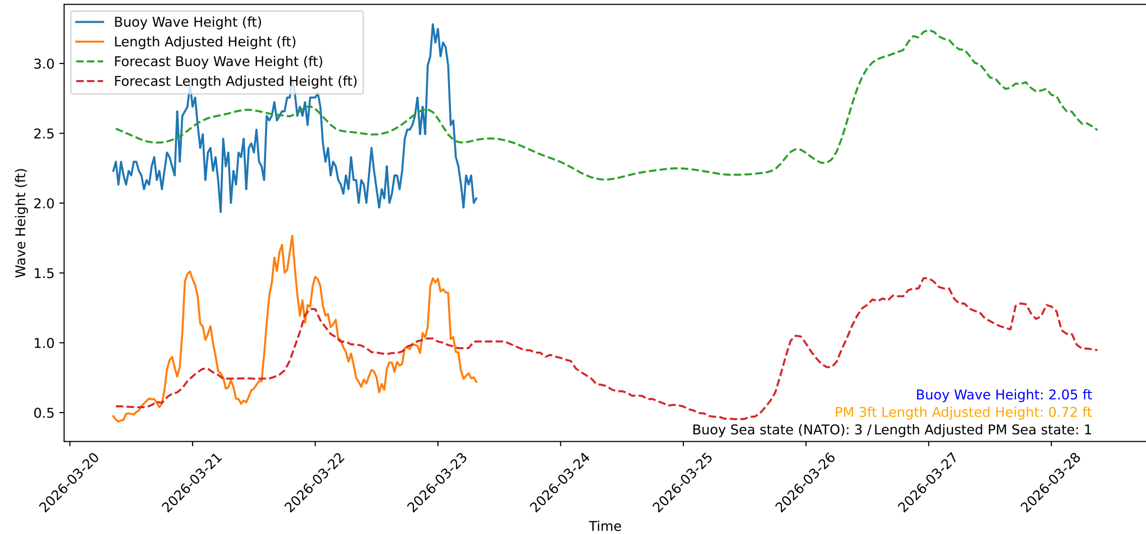
Wave Heights over Time for Green Beach at 2026-03-23 08:31:09
