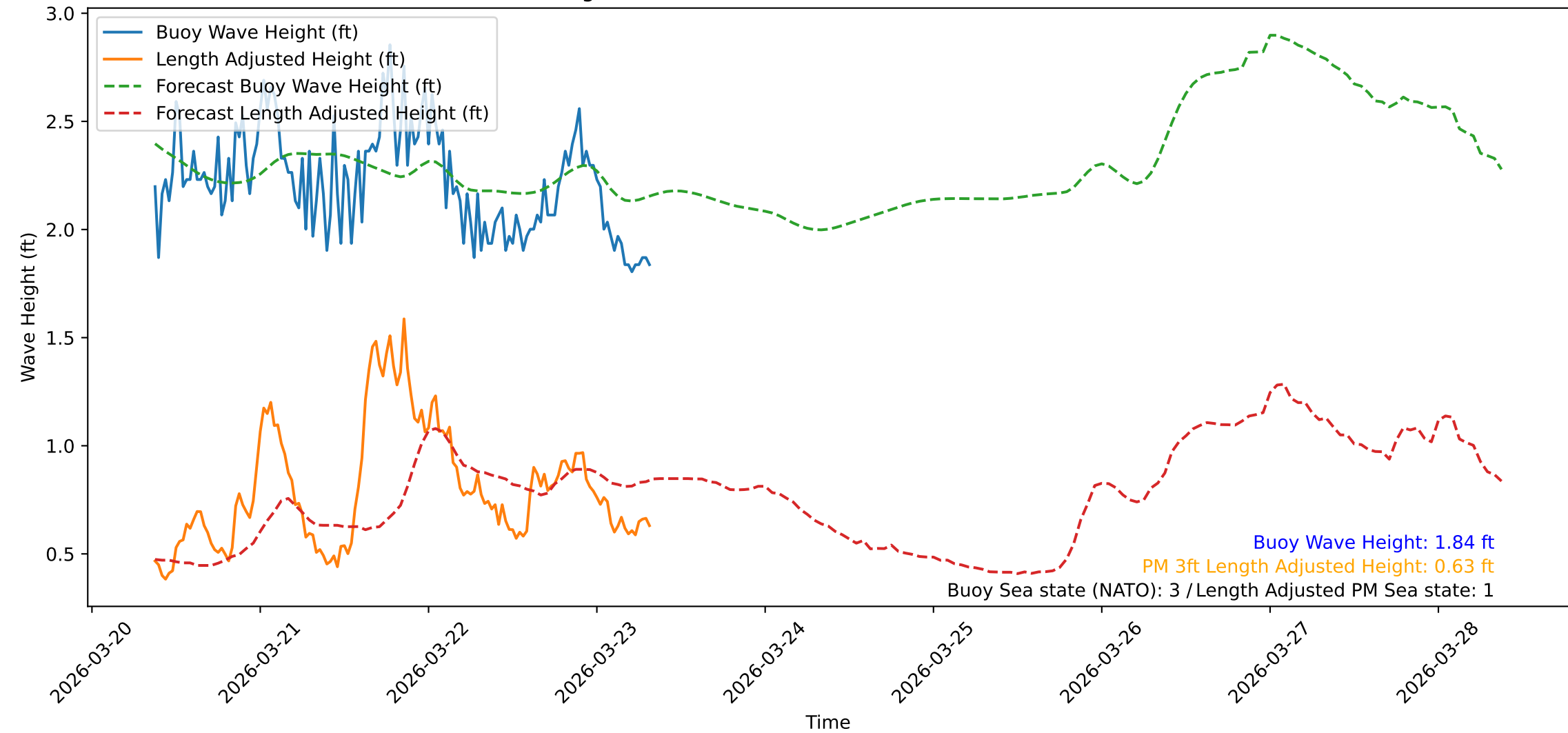
Wave Heights over Time for Red Beach at 2026-03-23 08:30:47
