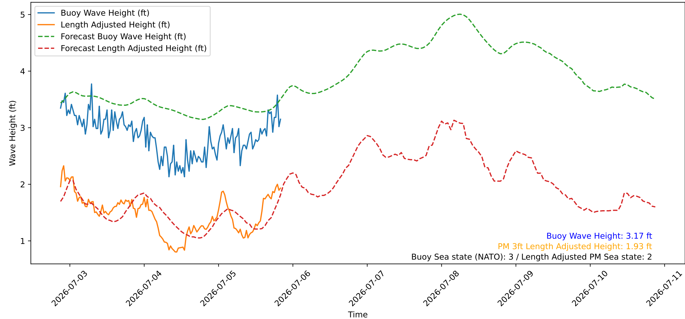
Wave Heights over Time for Oceanside Harbor at 2026-07-05 20:50:26
