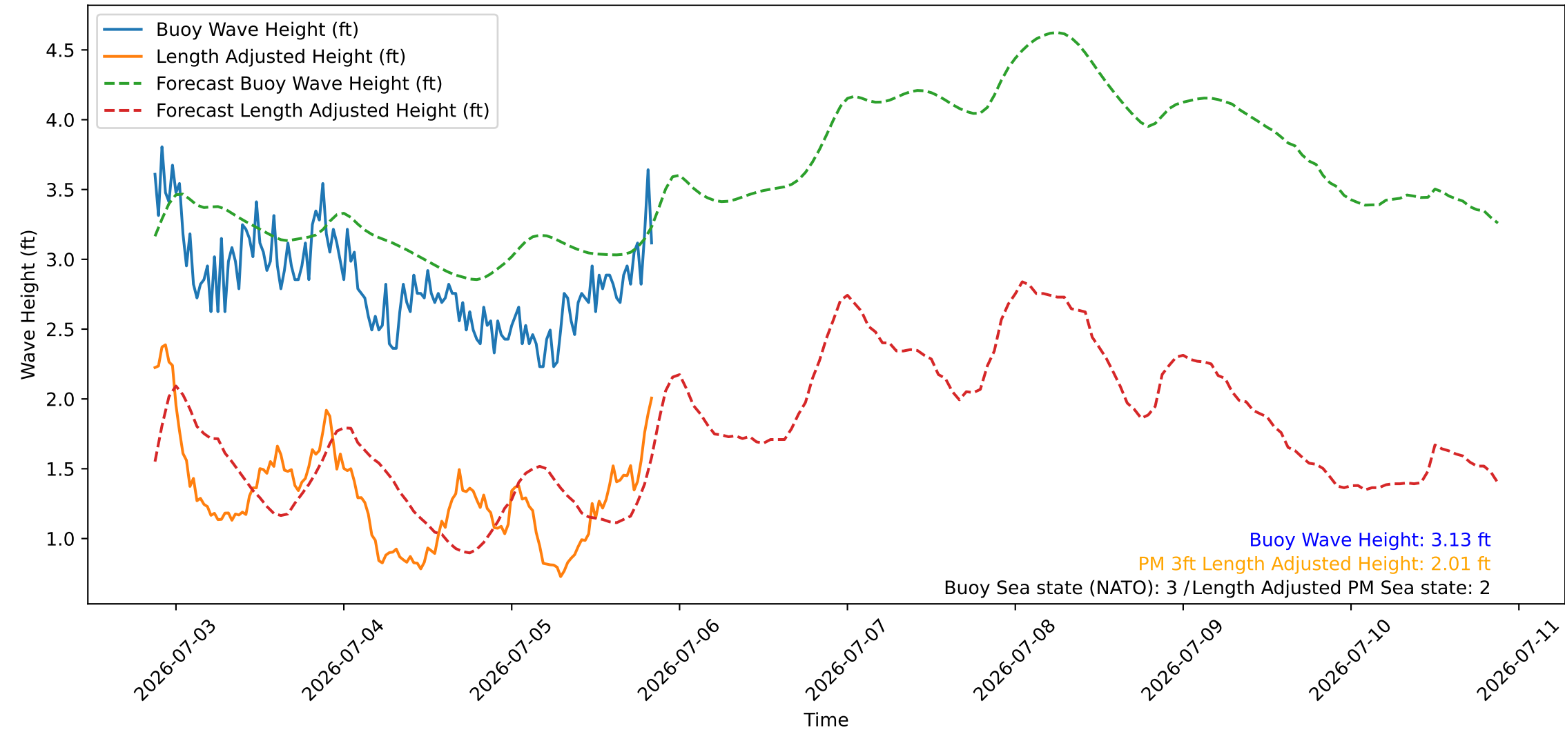
Wave Heights over Time for Red Beach at 2026-07-05 20:50:48
