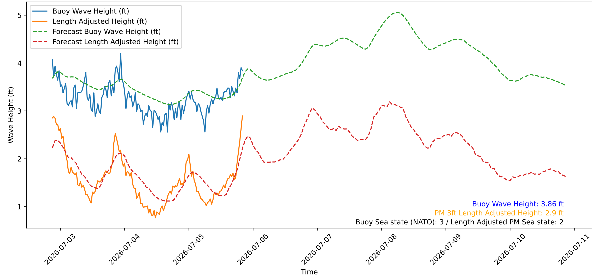
Wave Heights over Time for Green Beach at 2026-07-05 20:51:11
