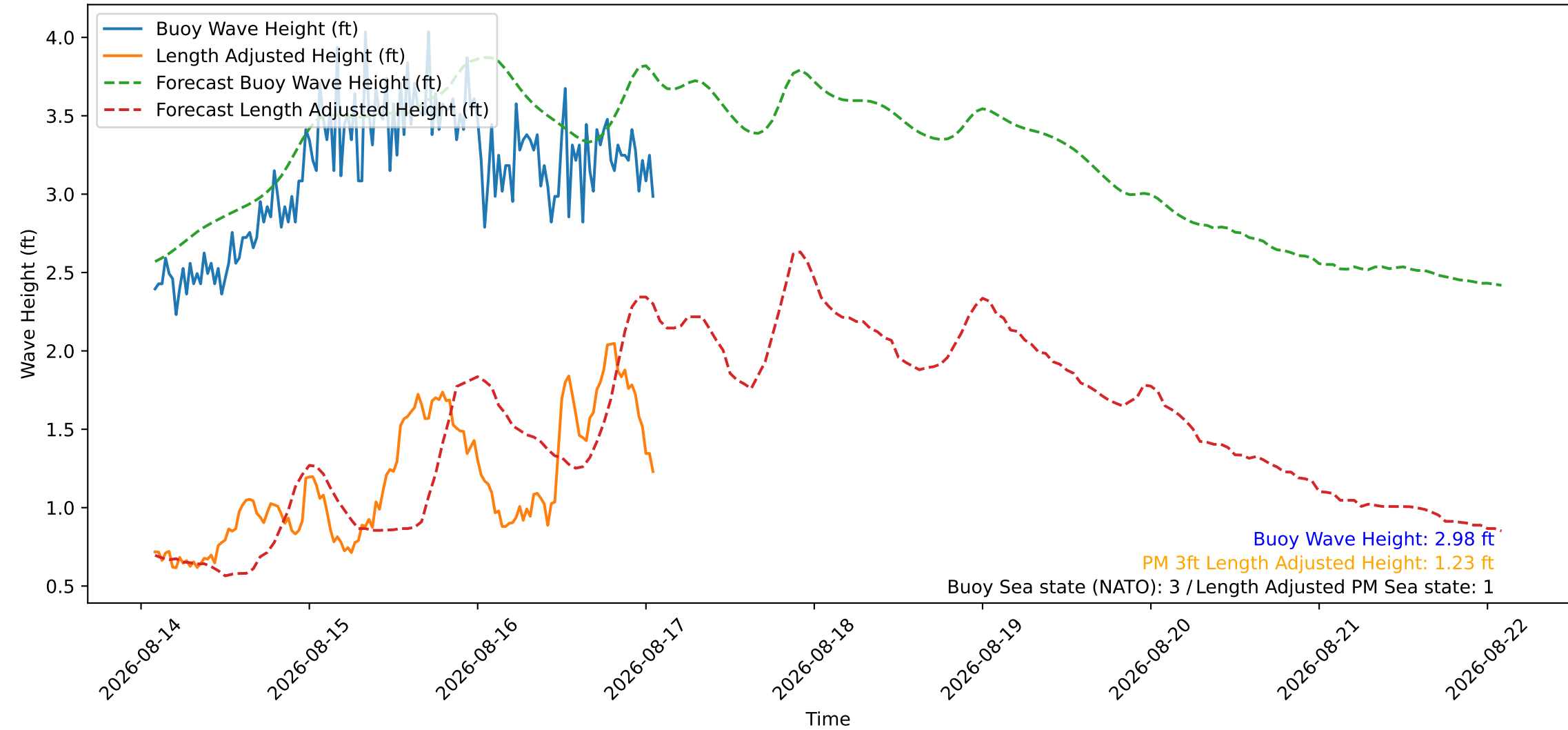
Wave Heights over Time for Red Beach at 2026-08-17 01:50:46
