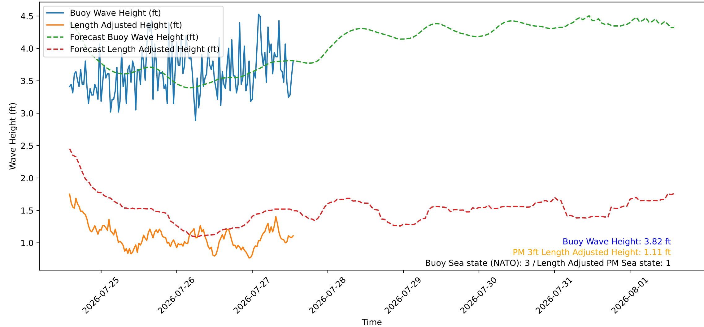
Wave Heights over Time for Red Beach at 2026-07-27 13:50:47
