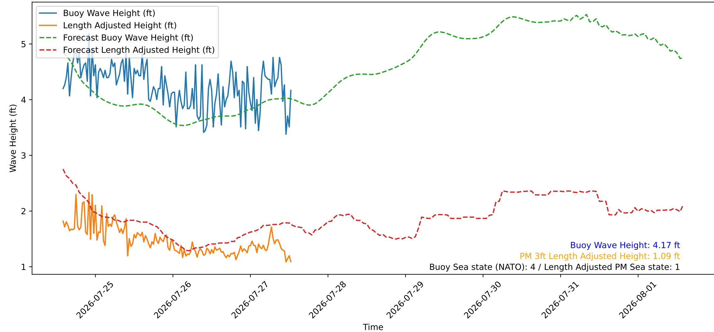
Wave Heights over Time for Green Beach at 2026-07-27 13:51:09
