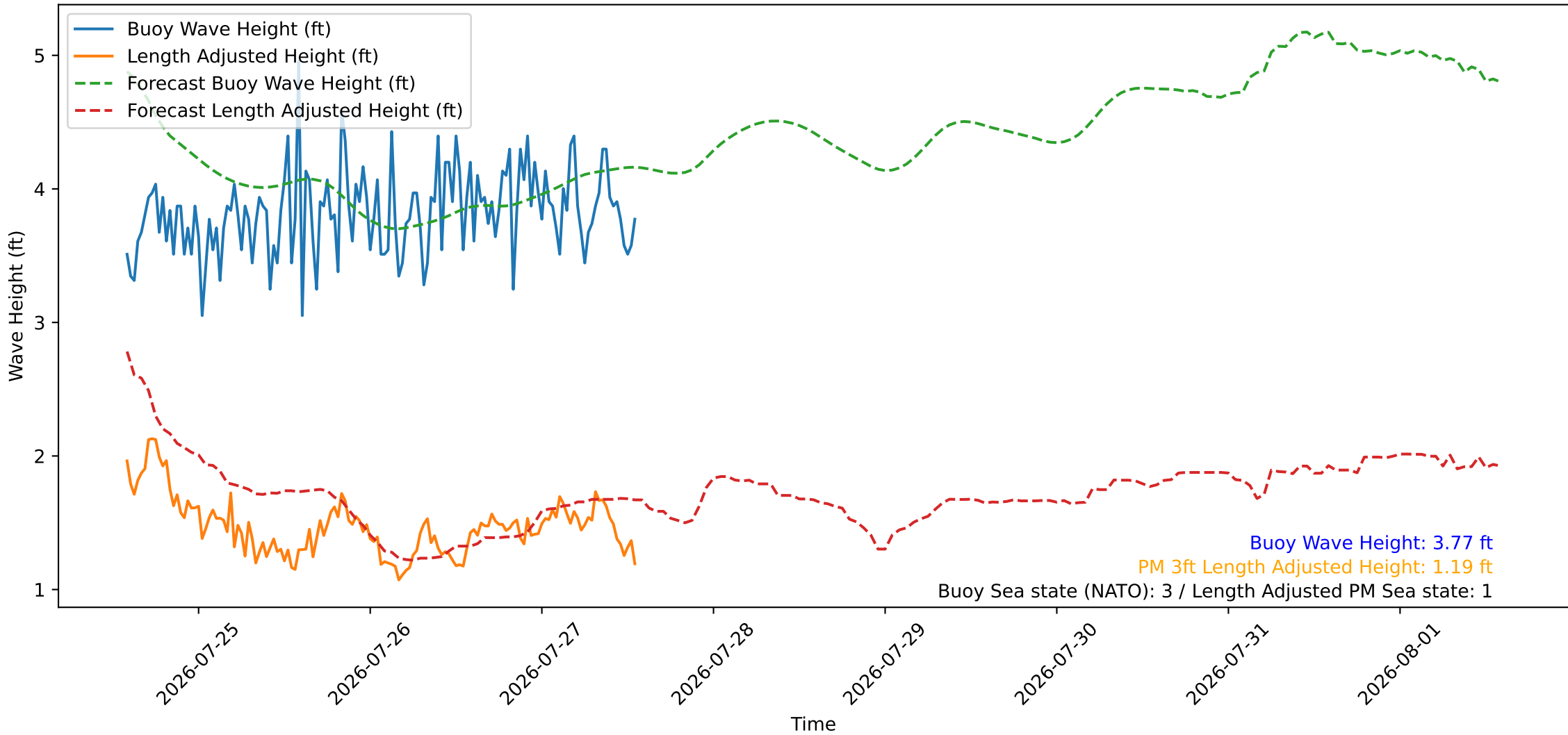
Wave Heights over Time for Oceanside Harbor at 2026-07-27 13:50:26
