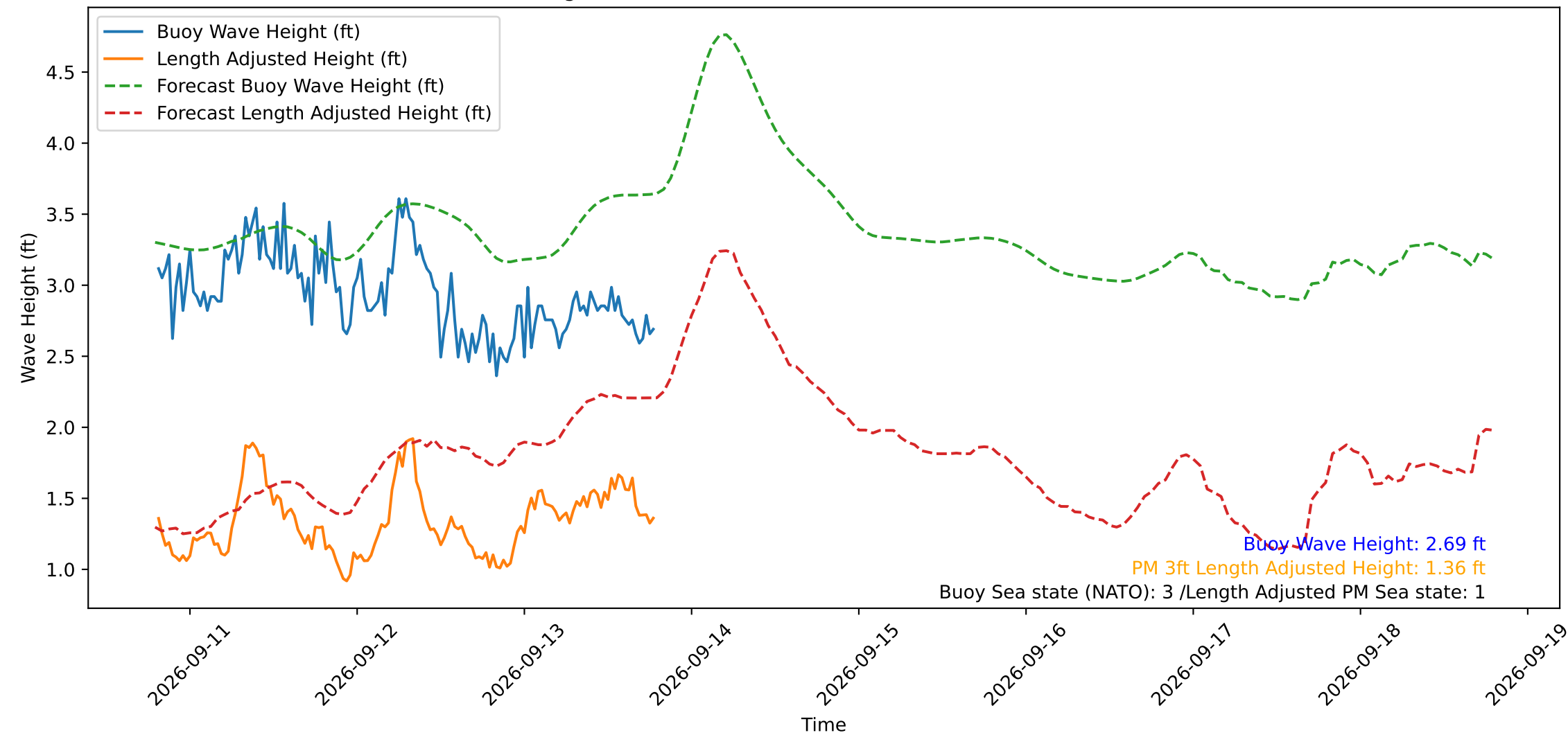
Wave Heights over Time for Green Beach at 2026-09-13 19:11:12
