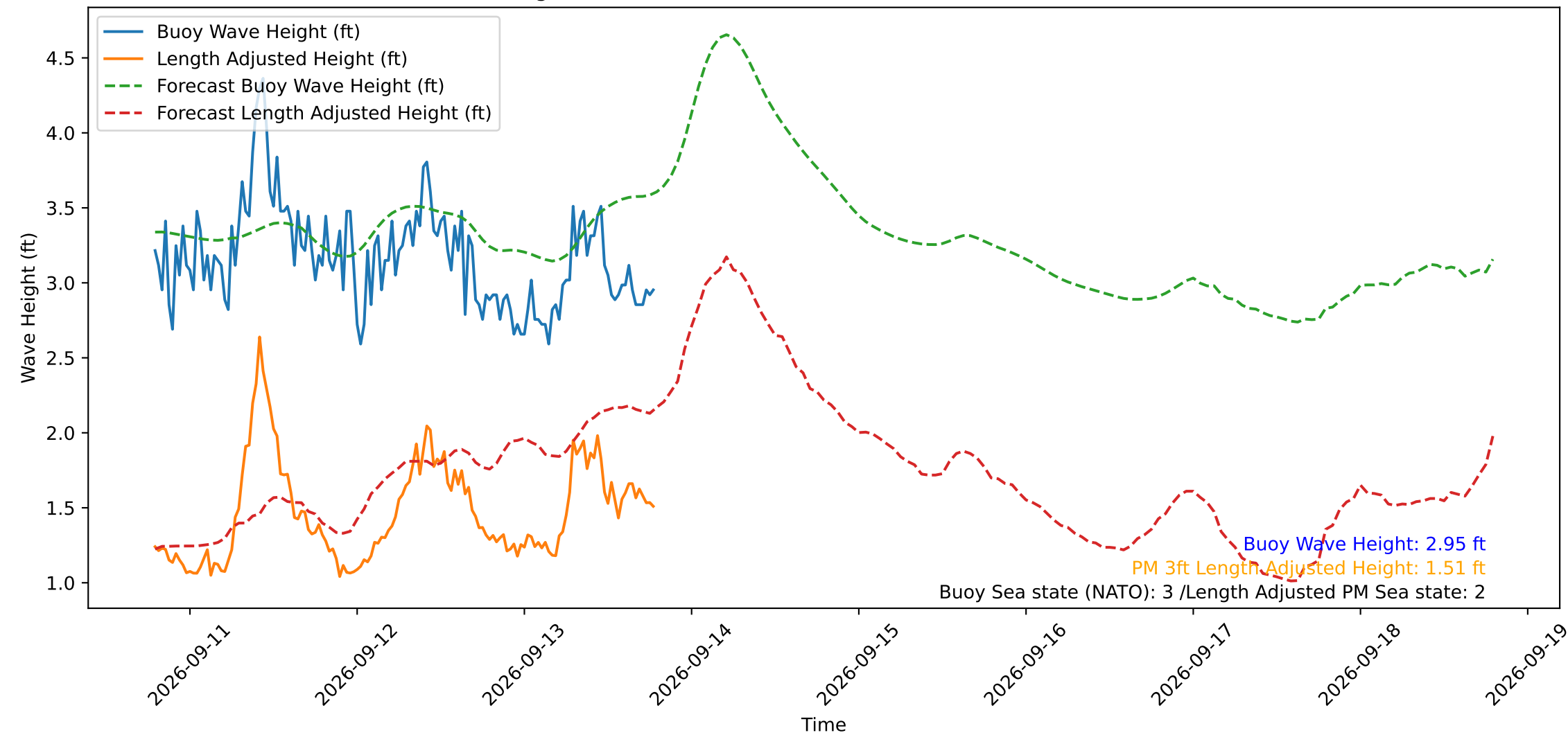
Wave Heights over Time for Oceanside Harbor at 2026-09-13 19:10:30
