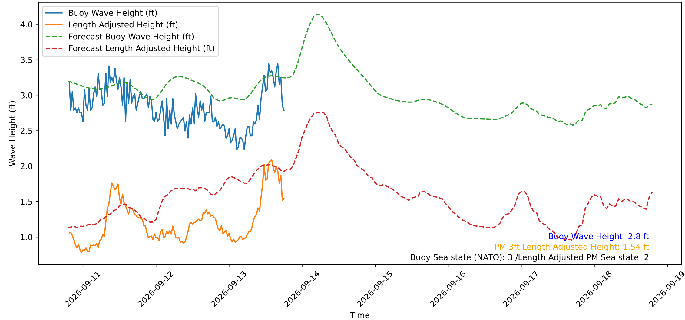
Wave Heights over Time for Red Beach at 2026-09-13 19:10:50
