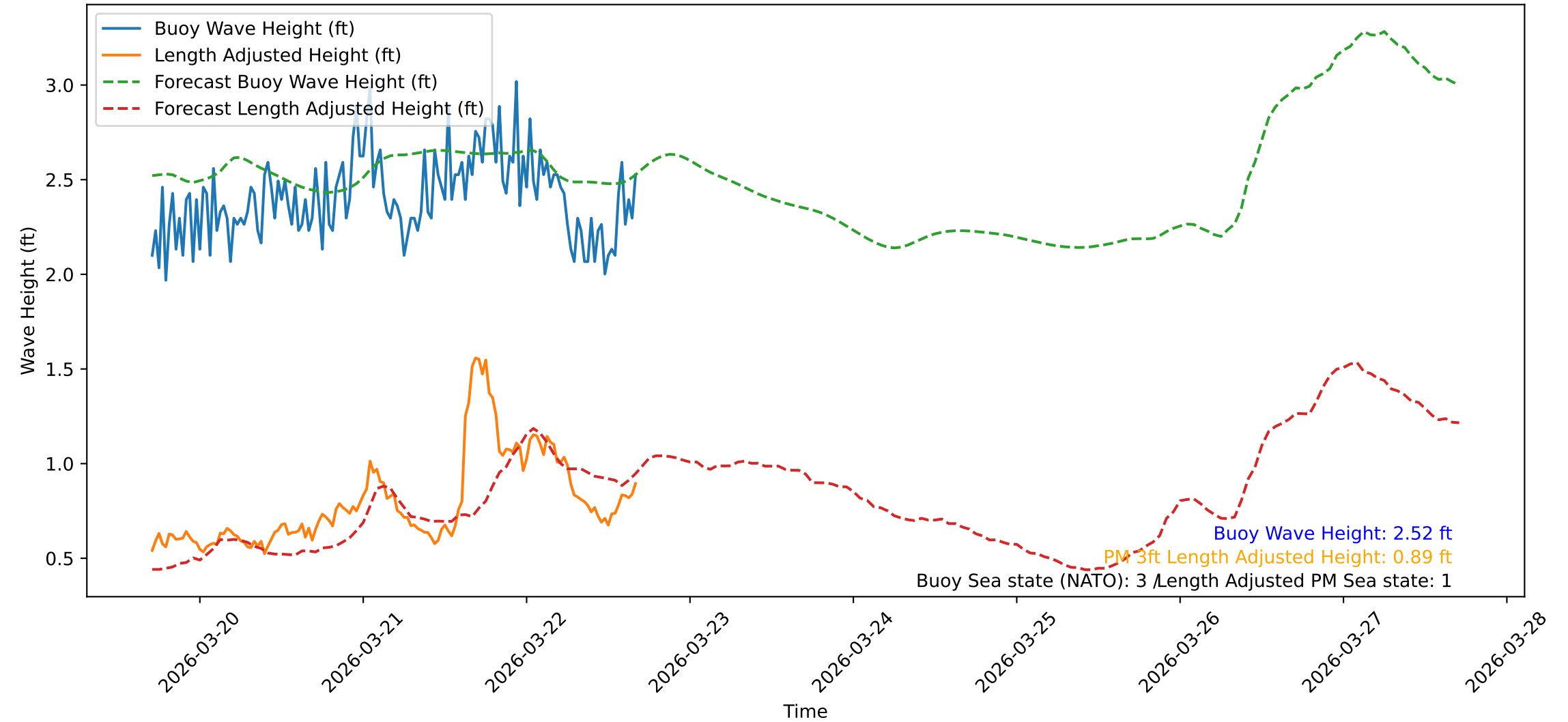
Wave Heights over Time for Oceanside Harbor at 2026-03-22 16:50:31
