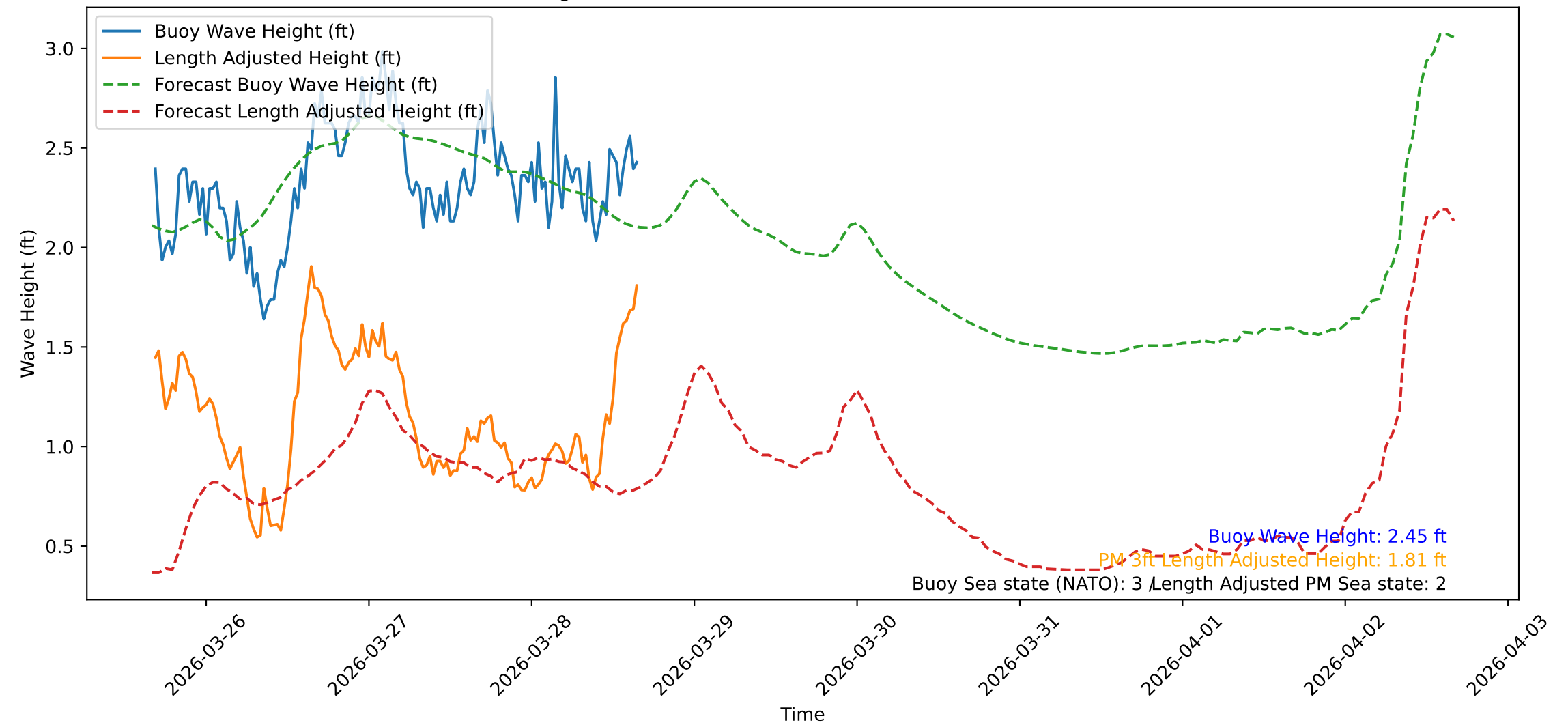
Wave Heights over Time for Red Beach at 2026-03-28 16:20:46
