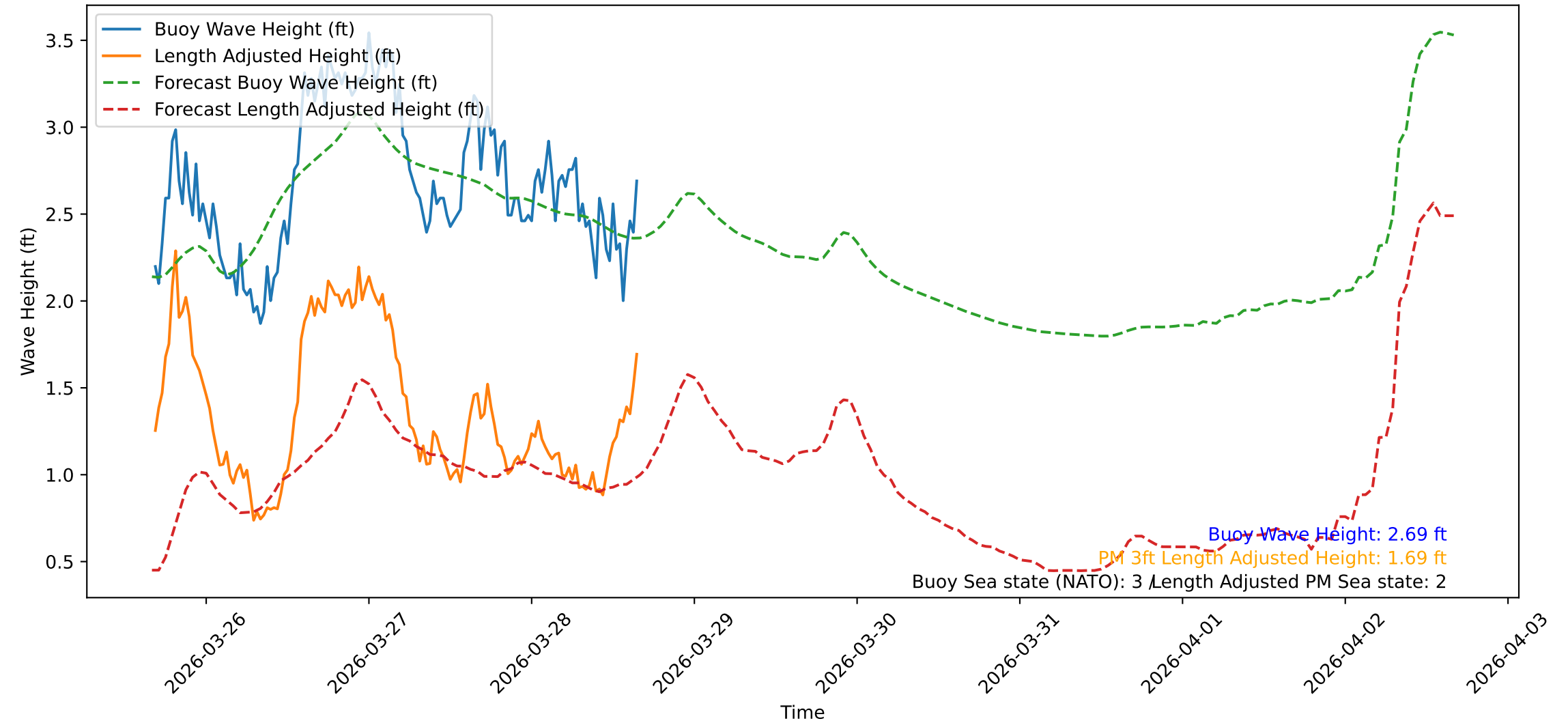
Wave Heights over Time for Green Beach at 2026-03-28 16:21:09
