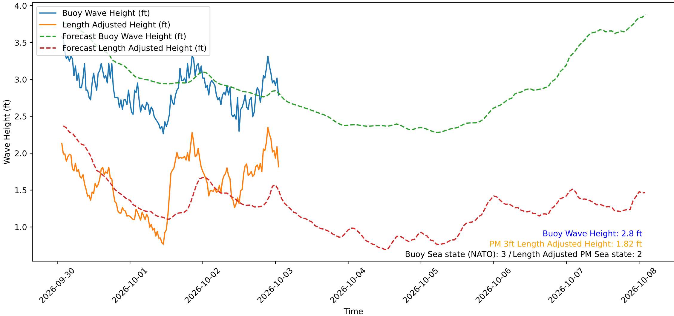
Wave Heights over Time for Oceanside Harbor at 2026-10-03 01:40:29
