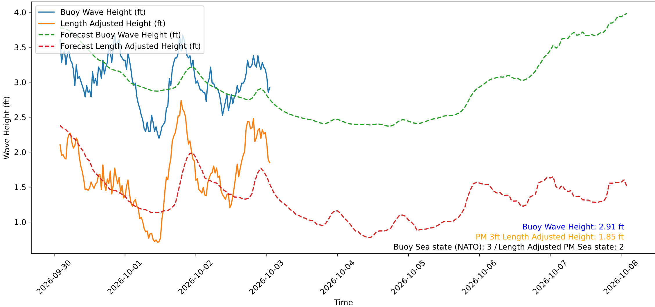
Wave Heights over Time for Green Beach at 2026-10-03 01:41:14
