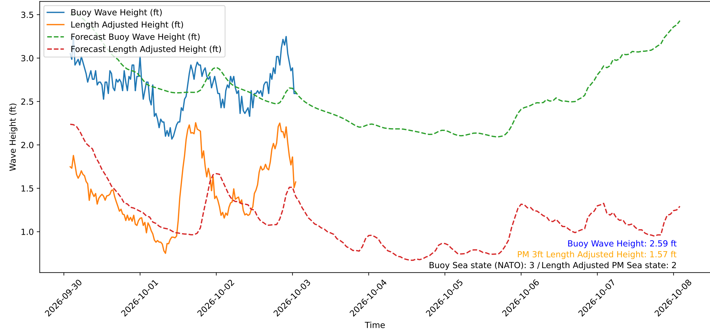
Wave Heights over Time for Red Beach at 2026-10-03 01:40:50
