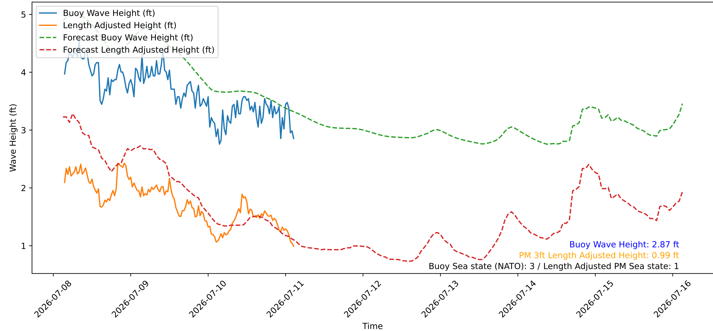
Wave Heights over Time for Green Beach at 2026-07-11 03:21:09
