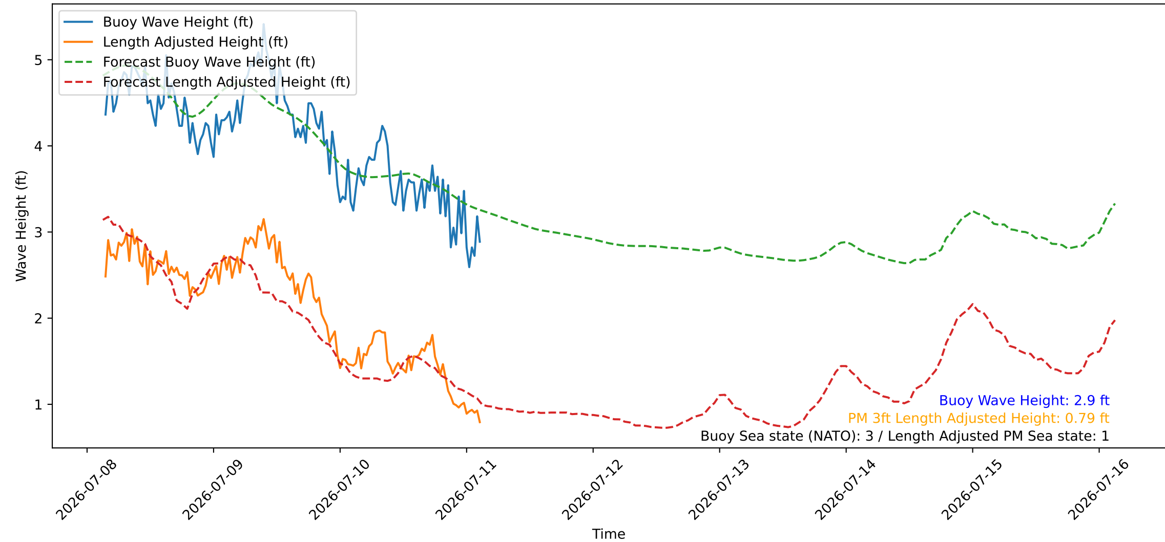
Wave Heights over Time for Oceanside Harbor at 2026-07-11 03:20:26
