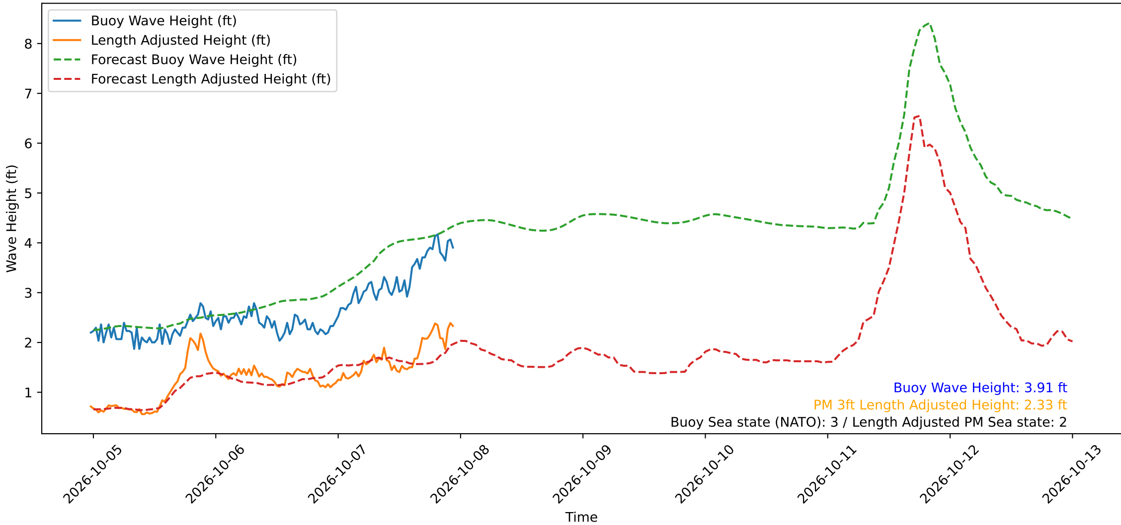
Wave Heights over Time for Oceanside Harbor at 2026-10-07 23:30:30
