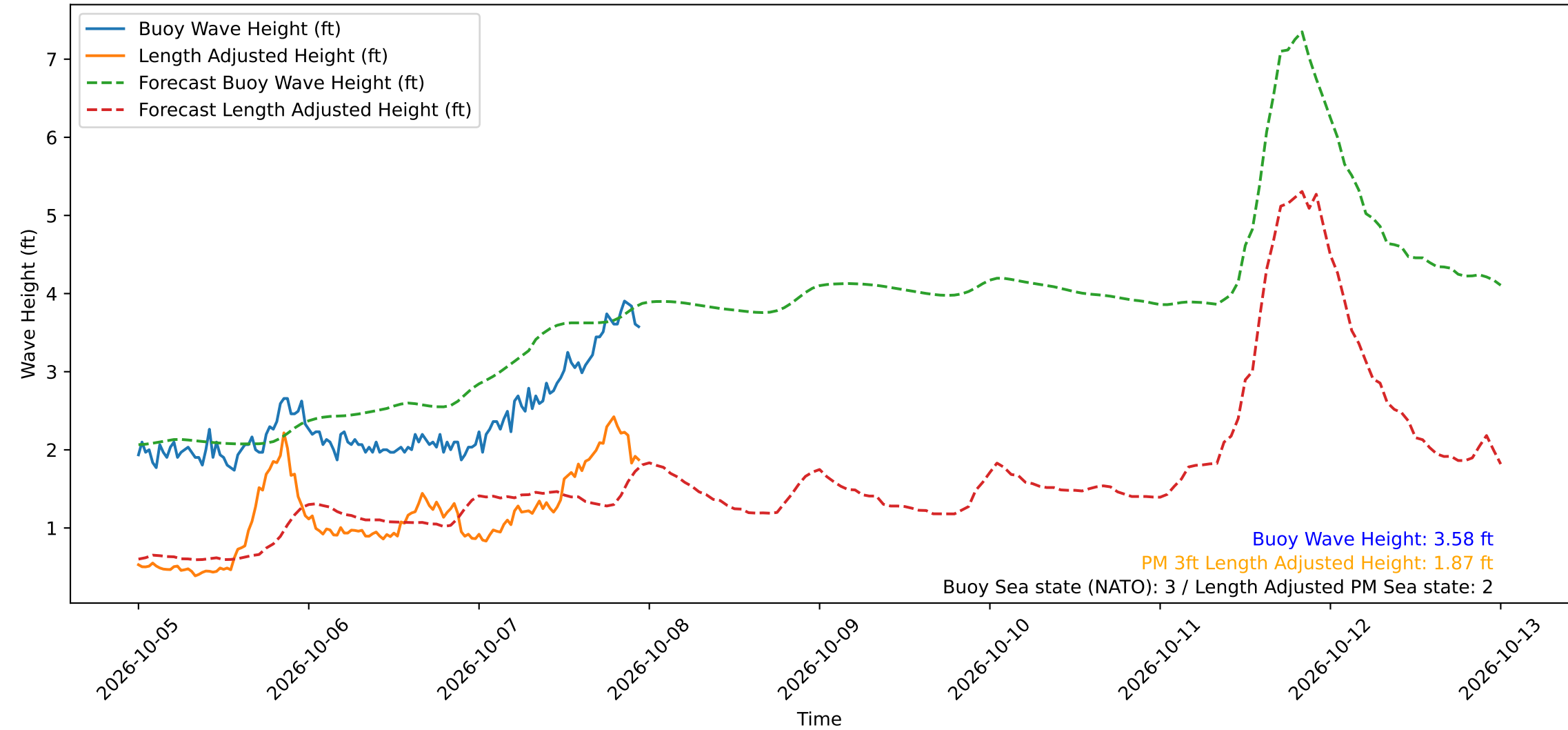
Wave Heights over Time for Red Beach at 2026-10-07 23:30:50
