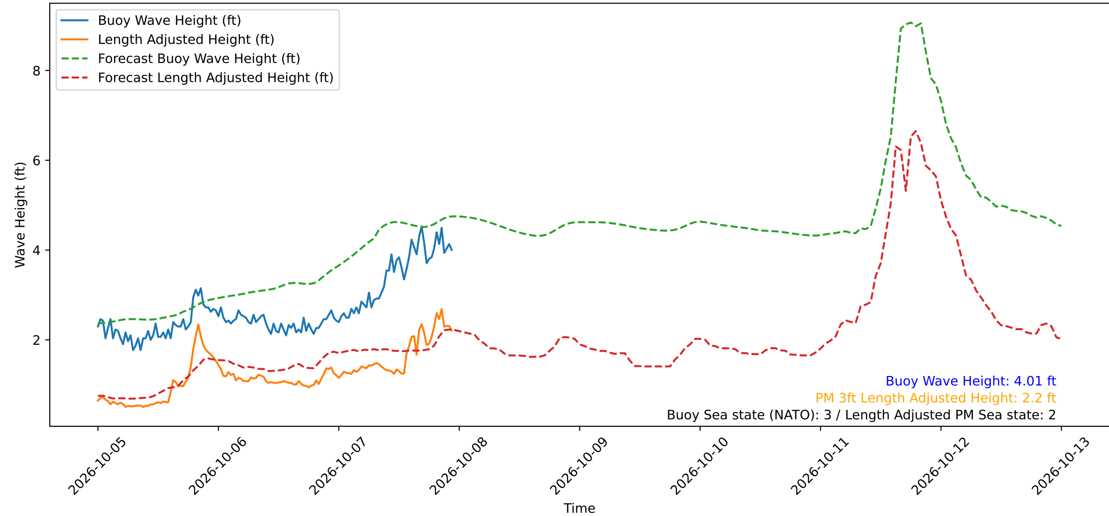
Wave Heights over Time for Green Beach at 2026-10-07 23:31:12
