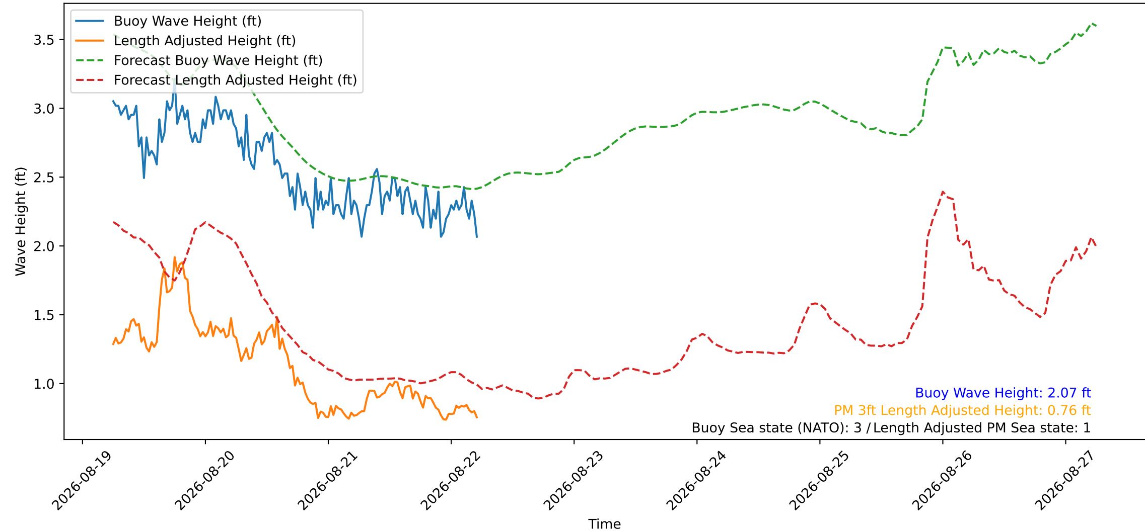
Wave Heights over Time for Red Beach at 2026-08-22 05:50:51
