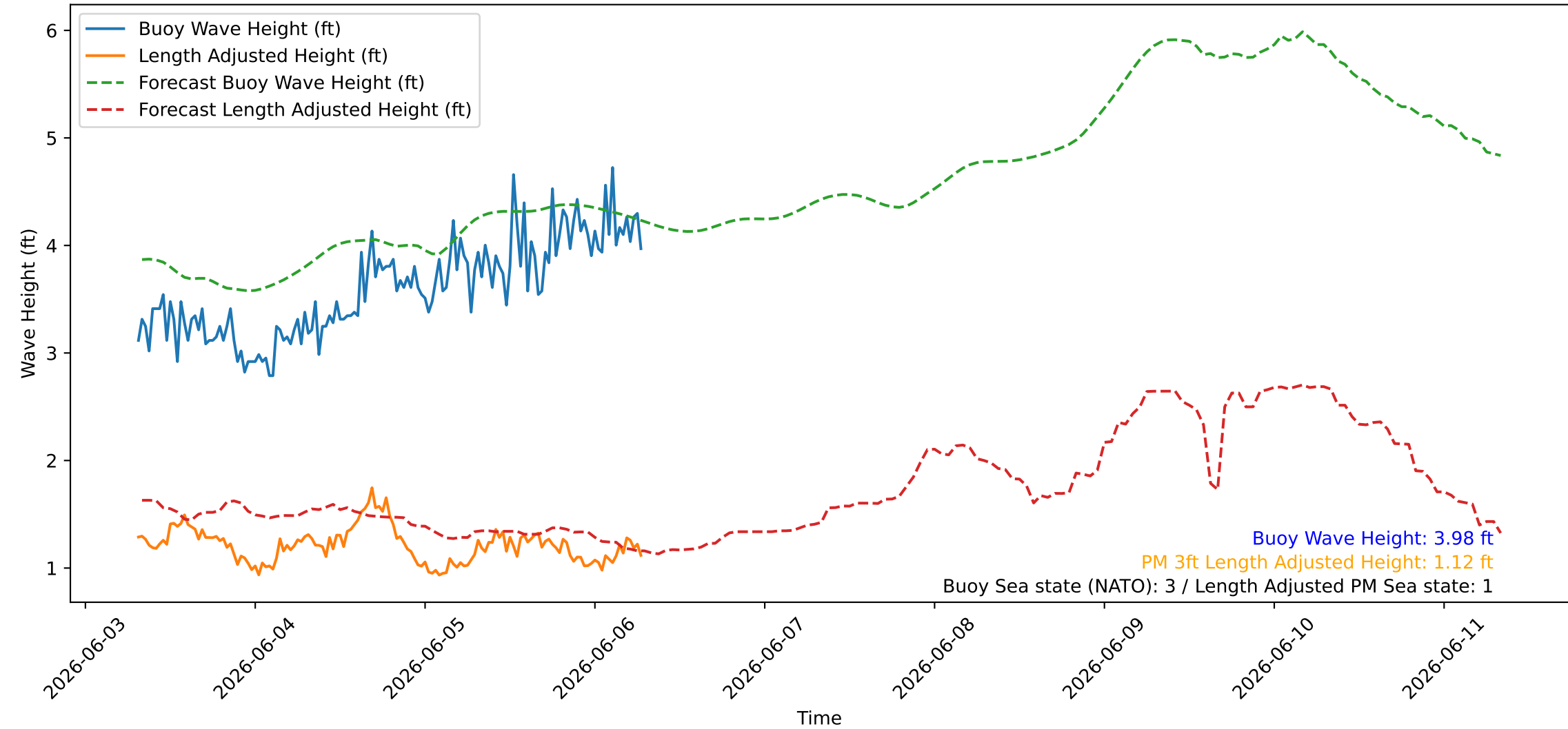
Wave Heights over Time for Green Beach at 2026-06-06 07:31:09
