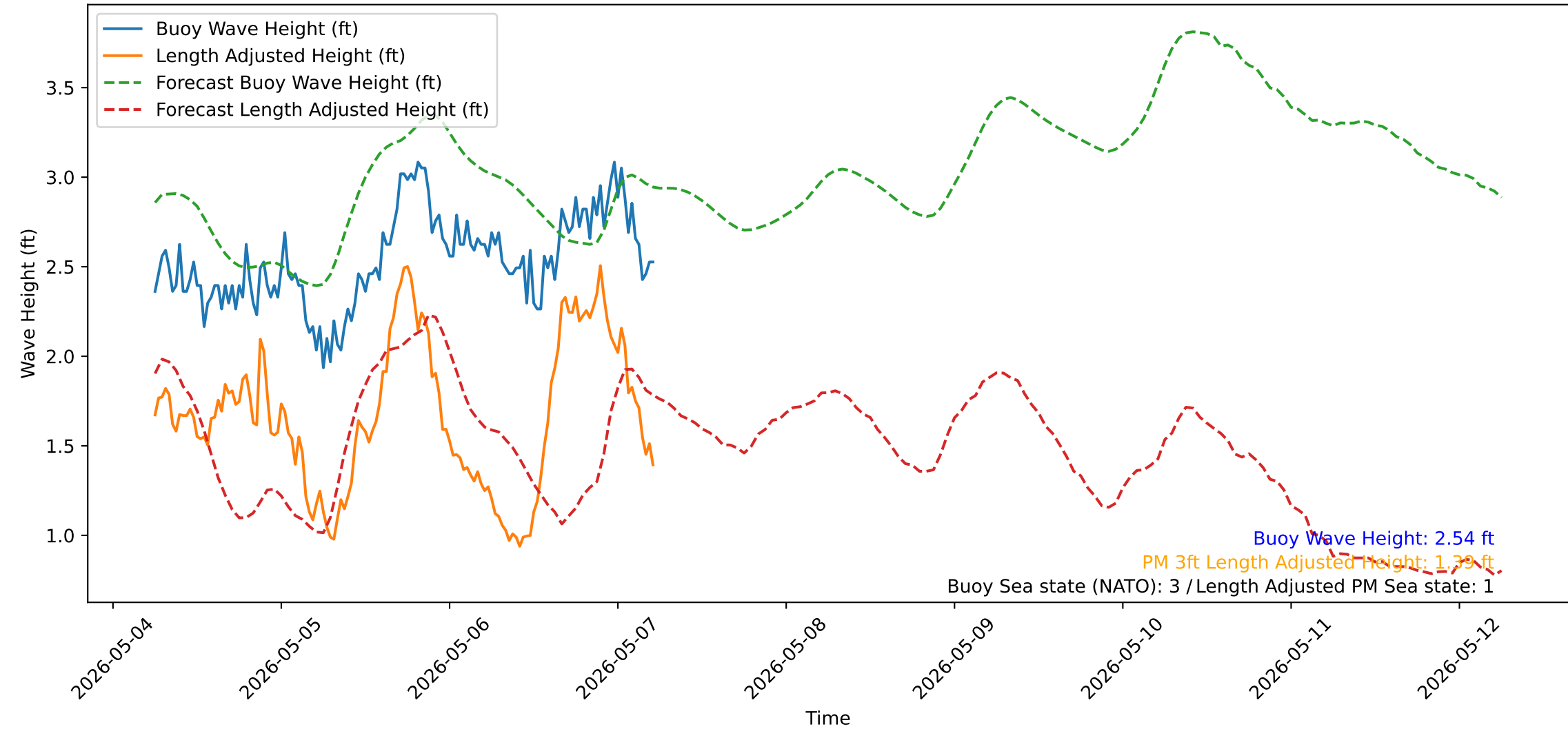
Wave Heights over Time for Red Beach at 2026-05-07 05:50:51
