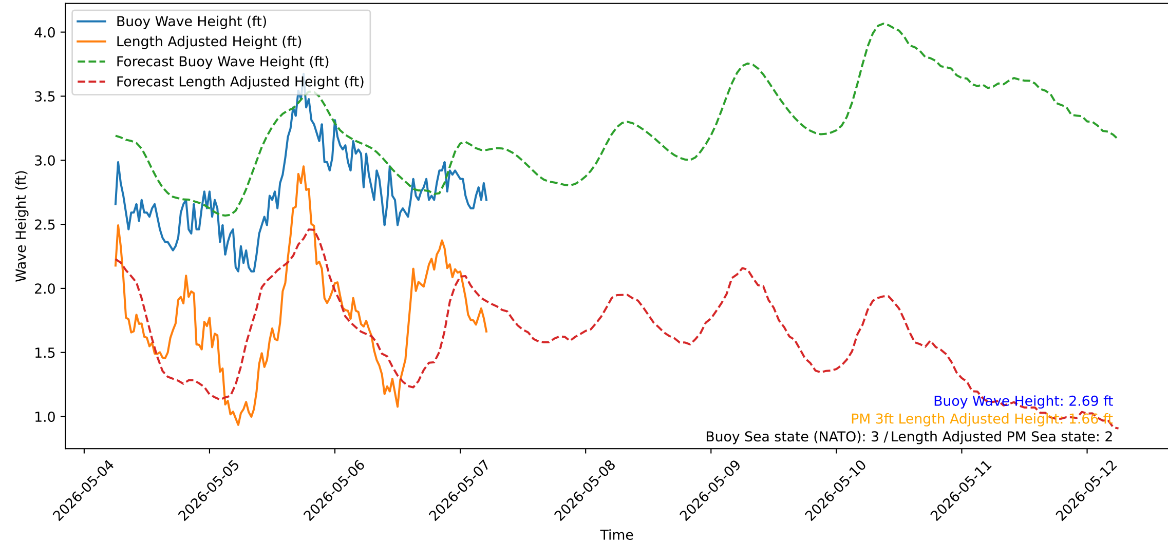
Wave Heights over Time for Green Beach at 2026-05-07 05:51:14
