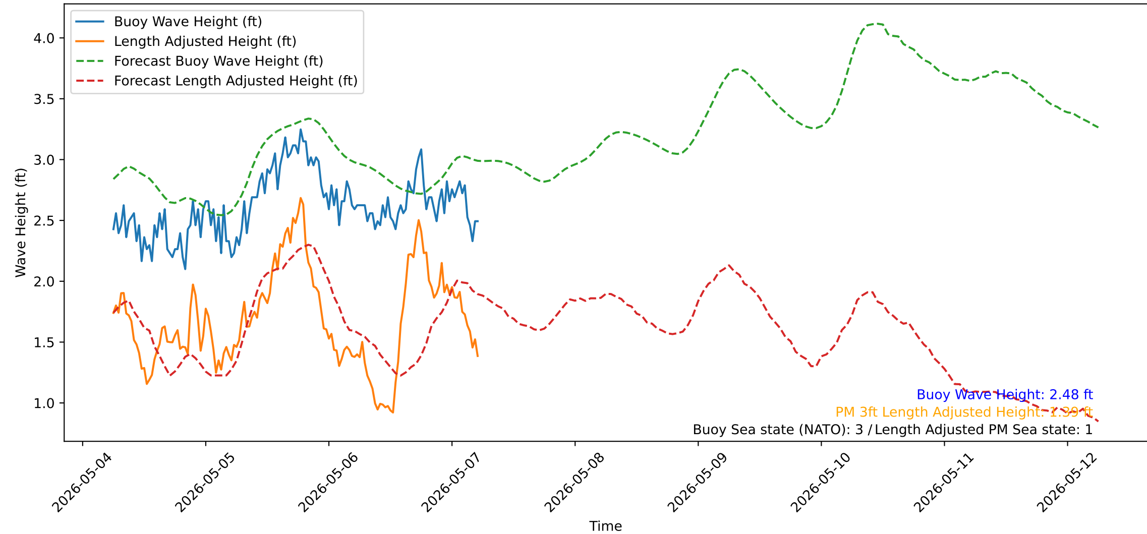
Wave Heights over Time for Oceanside Harbor at 2026-05-07 05:50:31
