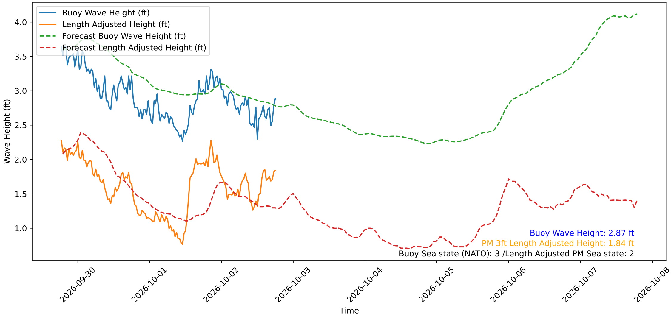
Wave Heights over Time for Oceanside Harbor at 2026-10-02 18:40:29
