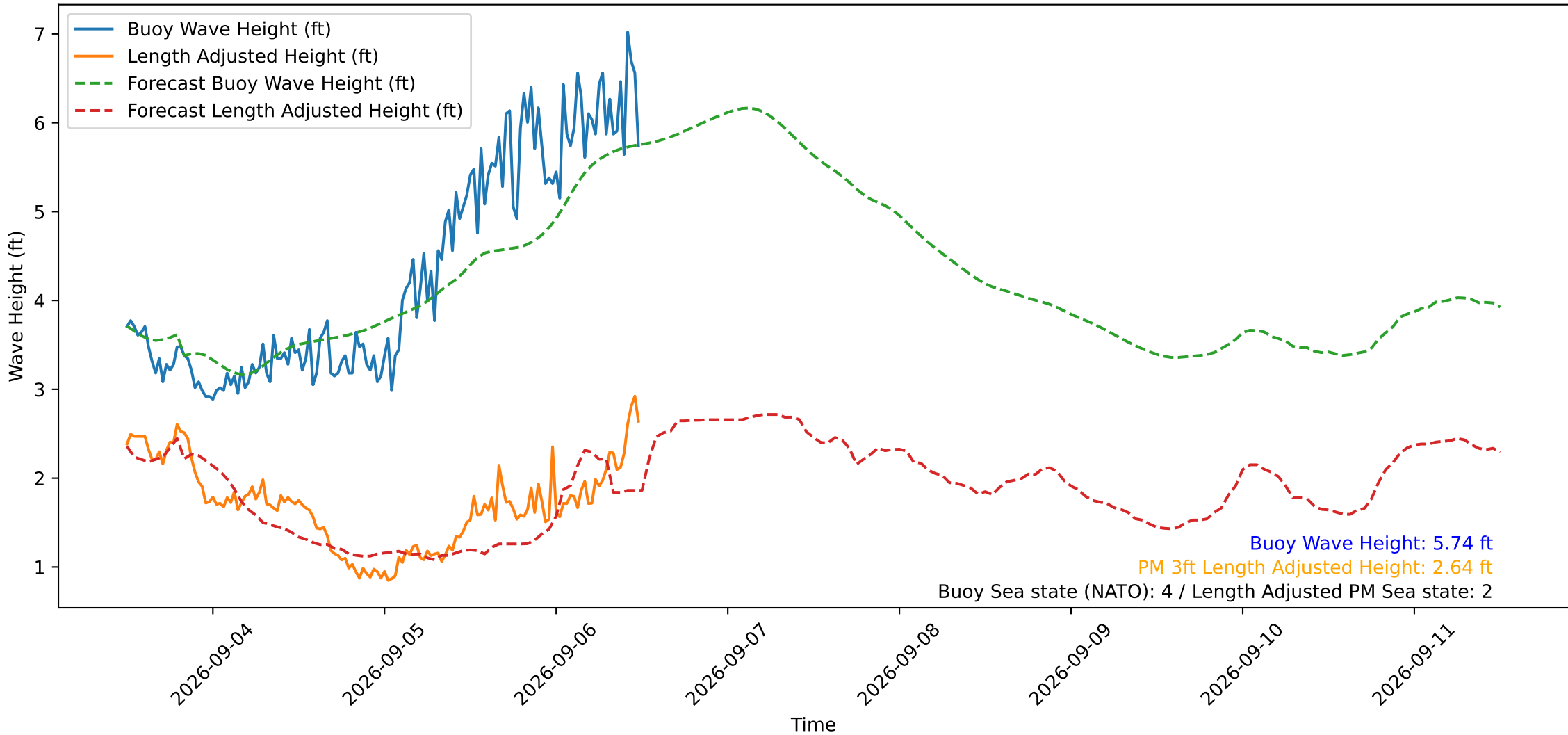
Wave Heights over Time for Oceanside Harbor at 2026-09-06 12:10:30
