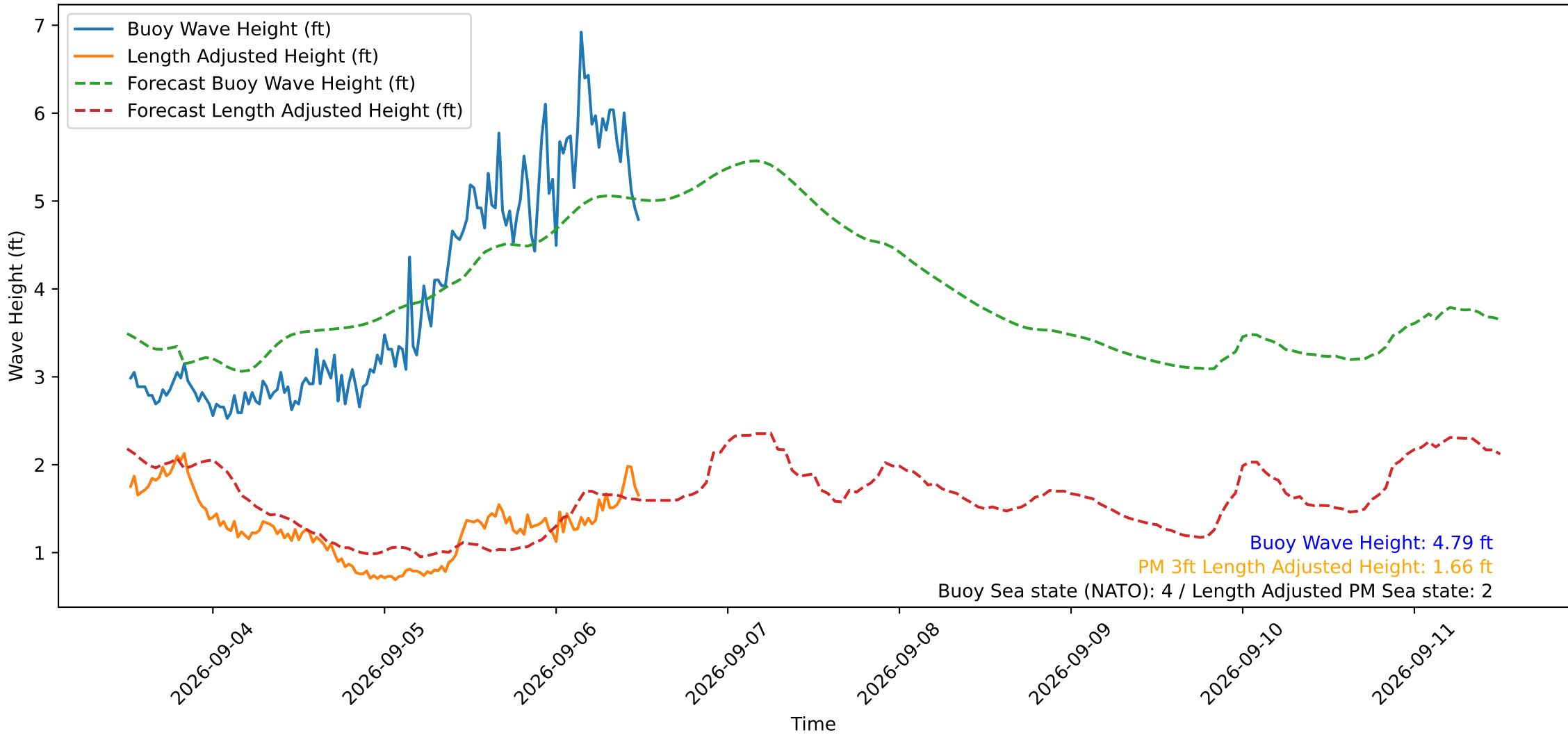
Wave Heights over Time for Red Beach at 2026-09-06 12:10:49
