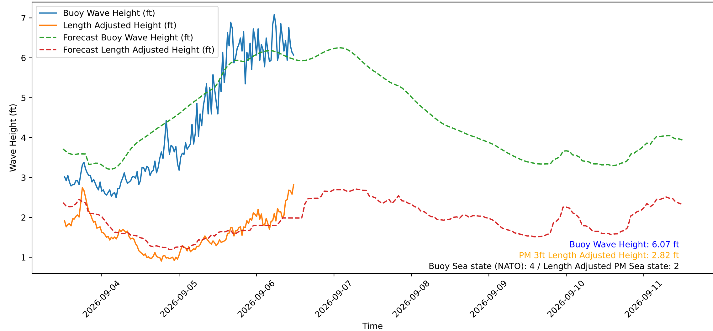
Wave Heights over Time for Green Beach at 2026-09-06 12:11:11
