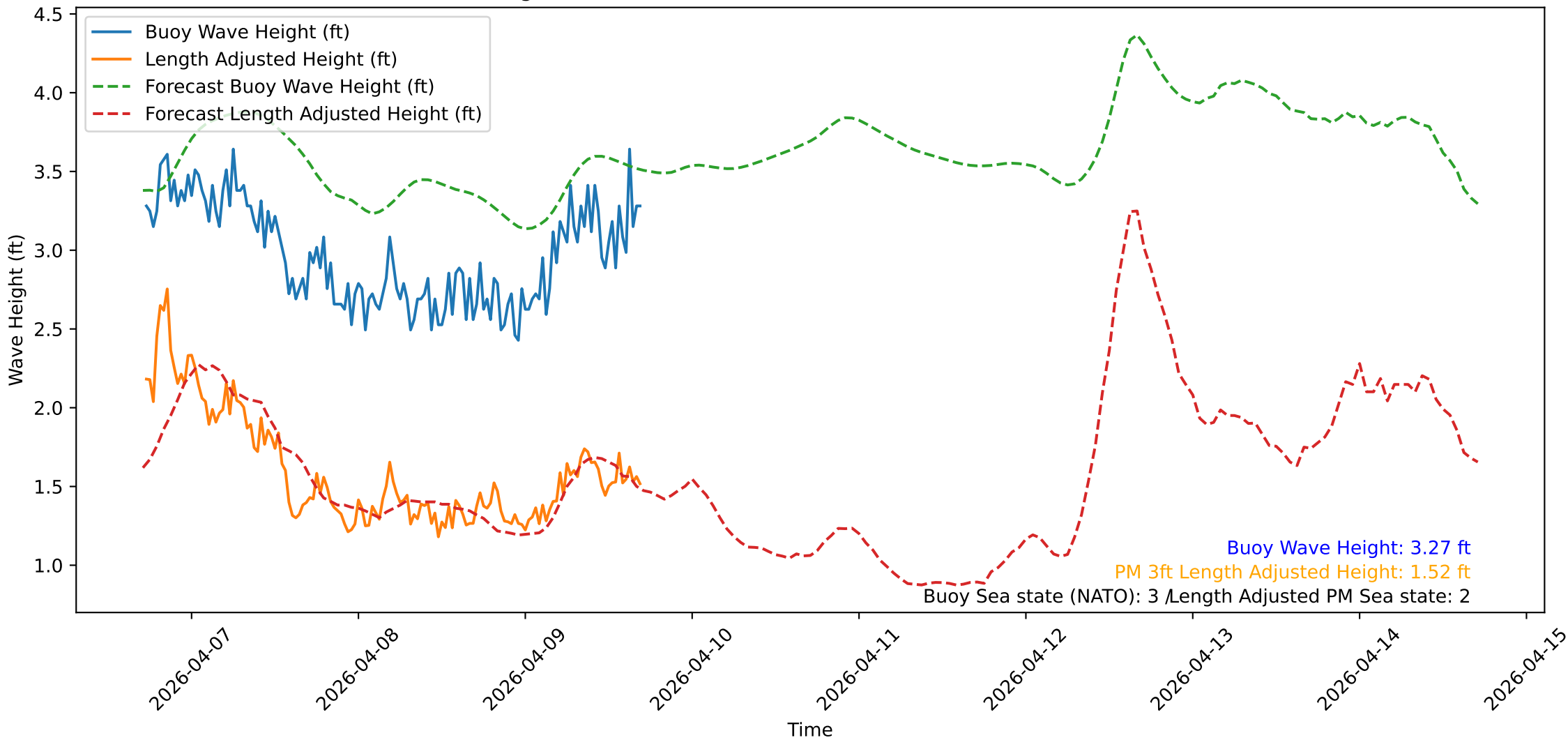
Wave Heights over Time for Oceanside Harbor at 2026-04-09 17:20:32
