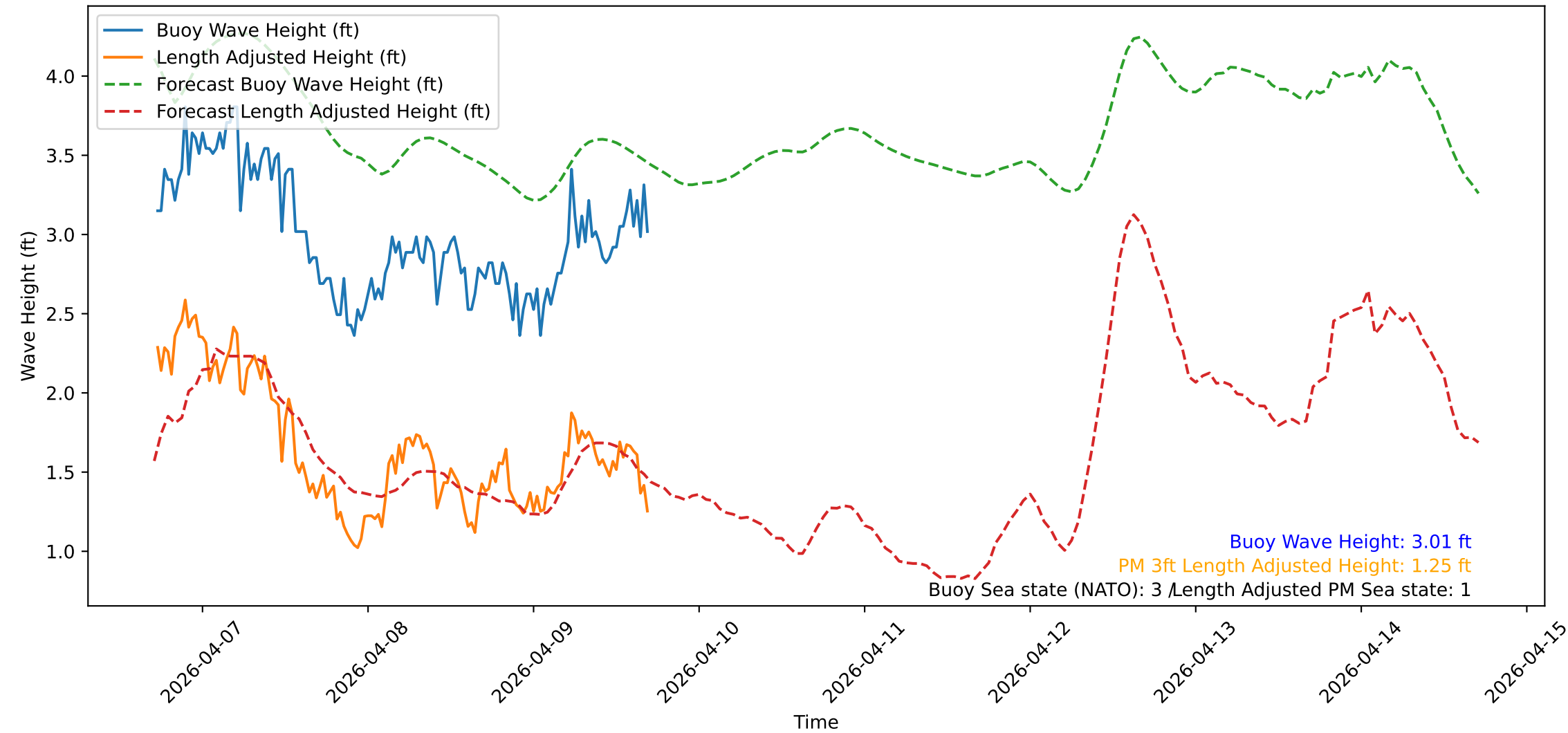
Wave Heights over Time for Green Beach at 2026-04-09 17:21:10
