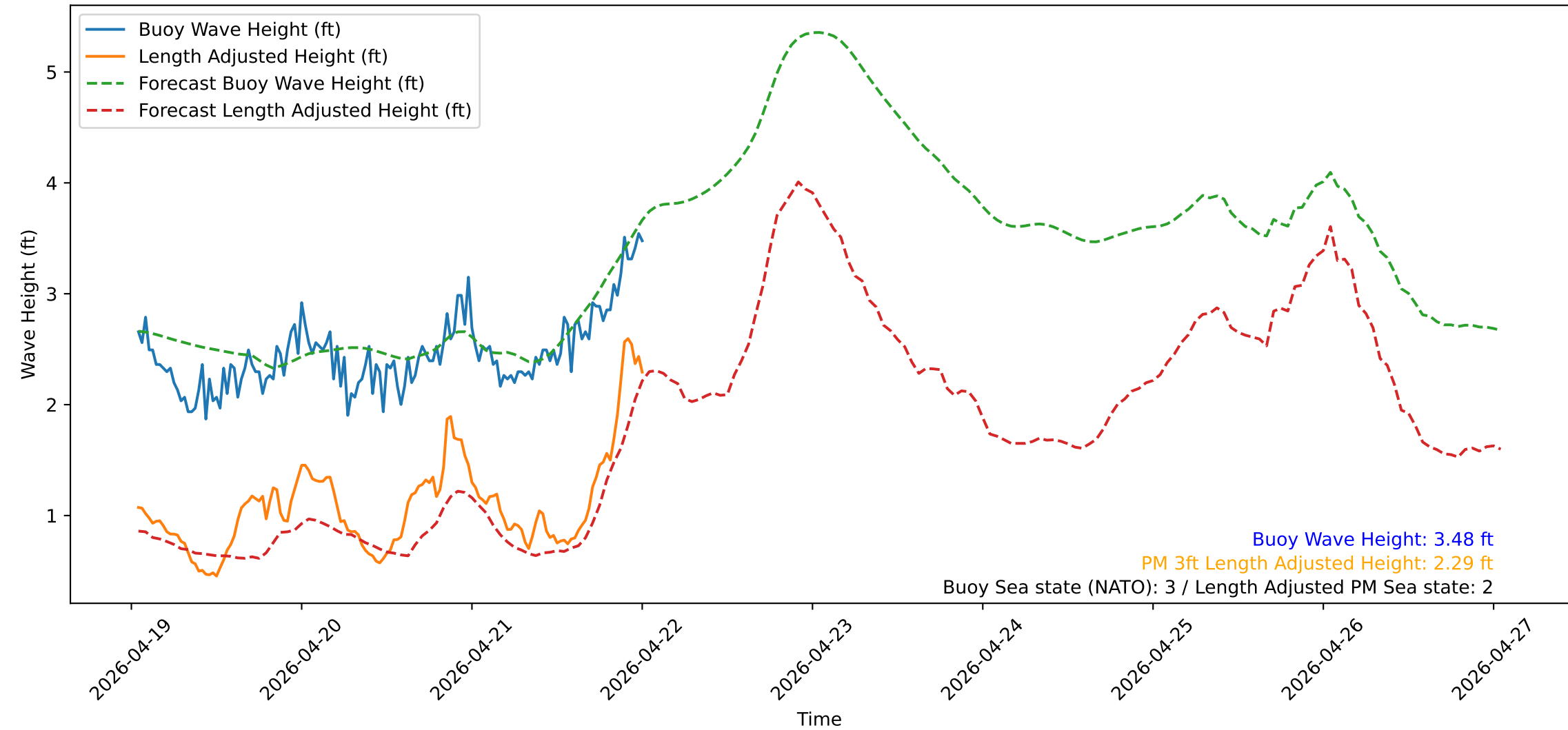
Wave Heights over Time for Green Beach at 2026-04-22 01:01:13
