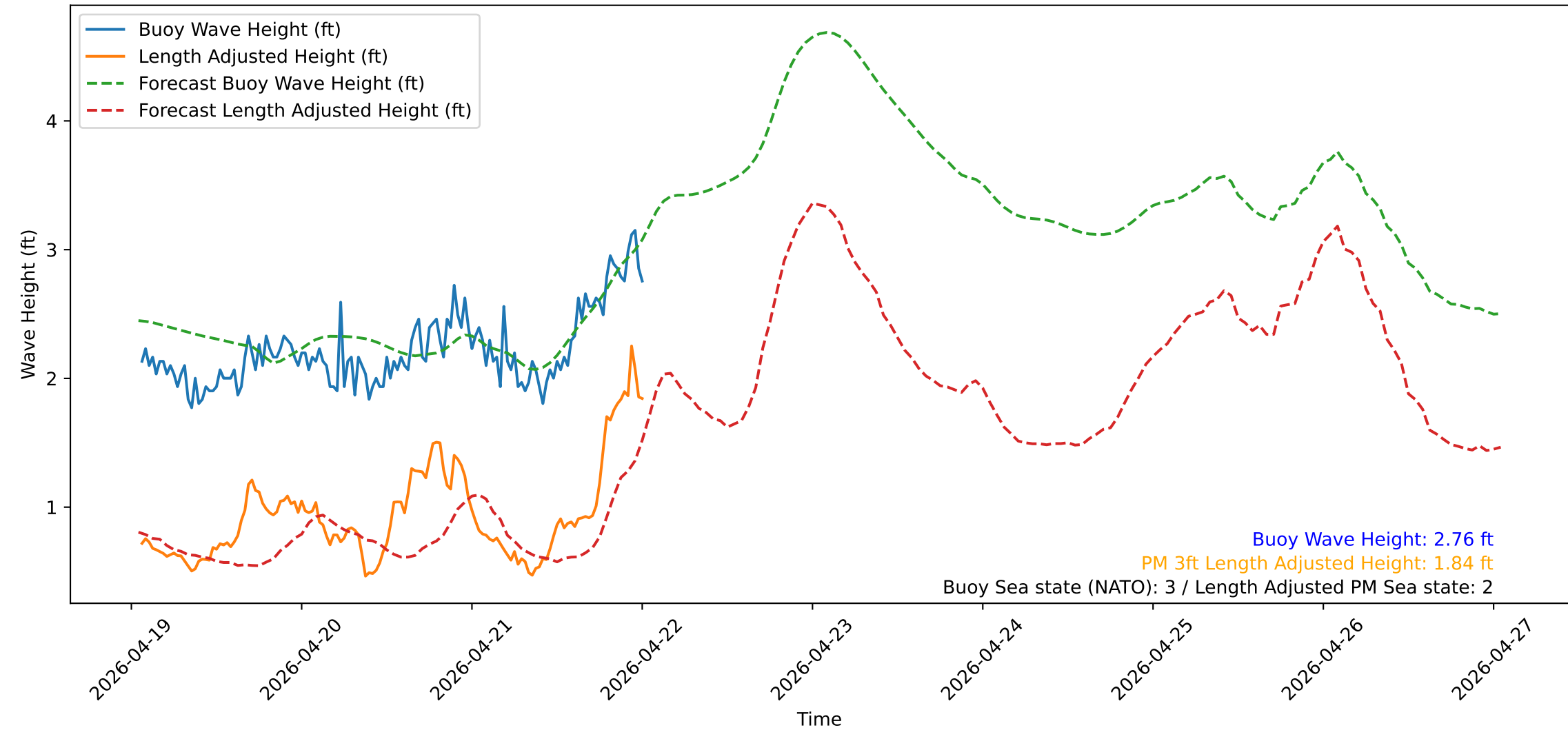
Wave Heights over Time for Red Beach at 2026-04-22 01:00:51
