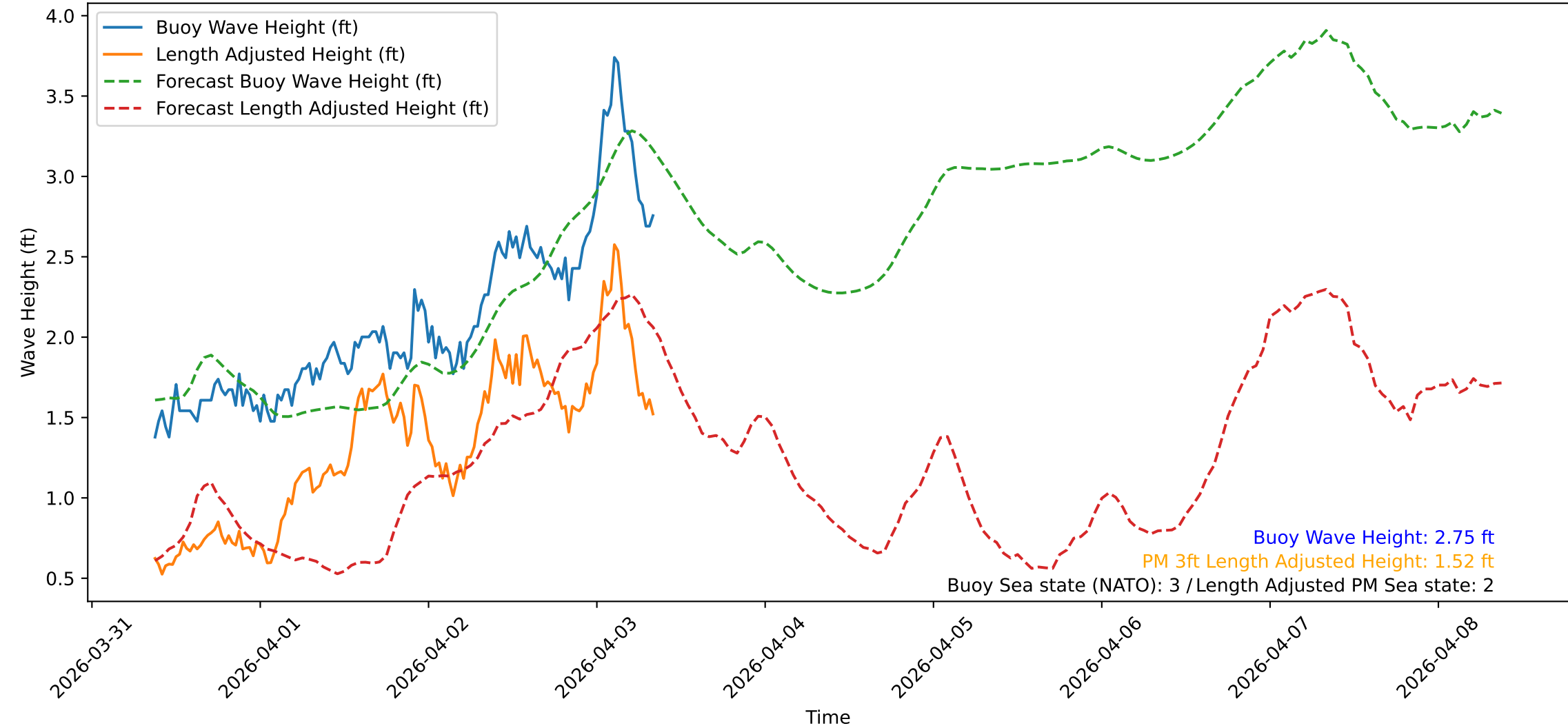
Wave Heights over Time for Red Beach at 2026-04-03 08:50:47
