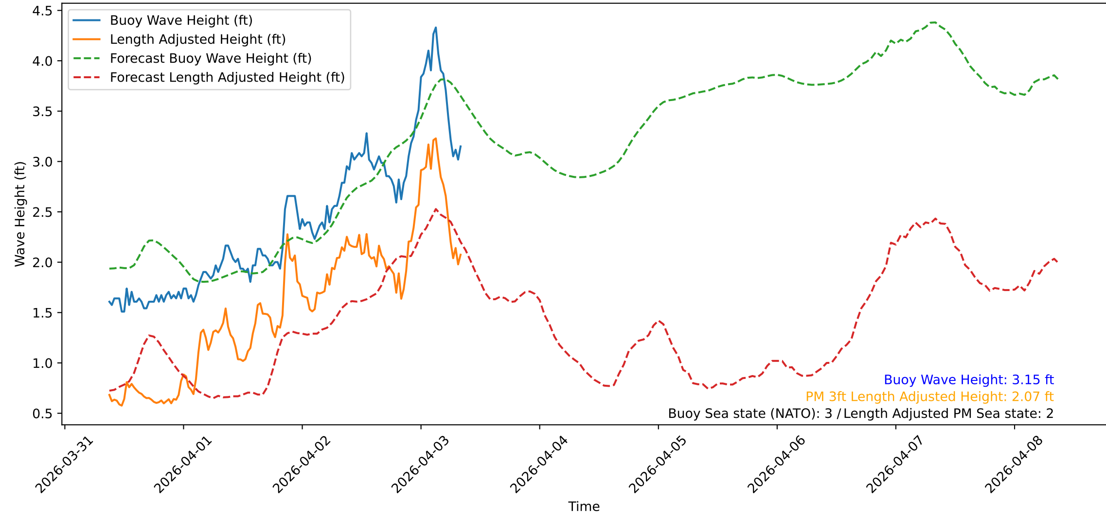
Wave Heights over Time for Green Beach at 2026-04-03 08:51:09
