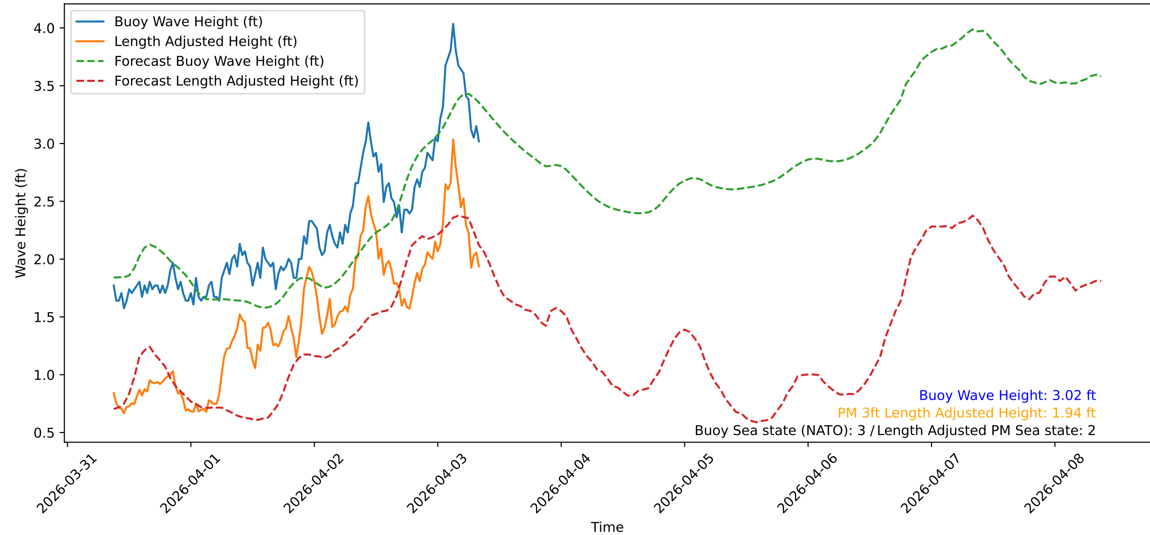
Wave Heights over Time for Oceanside Harbor at 2026-04-03 08:50:32
