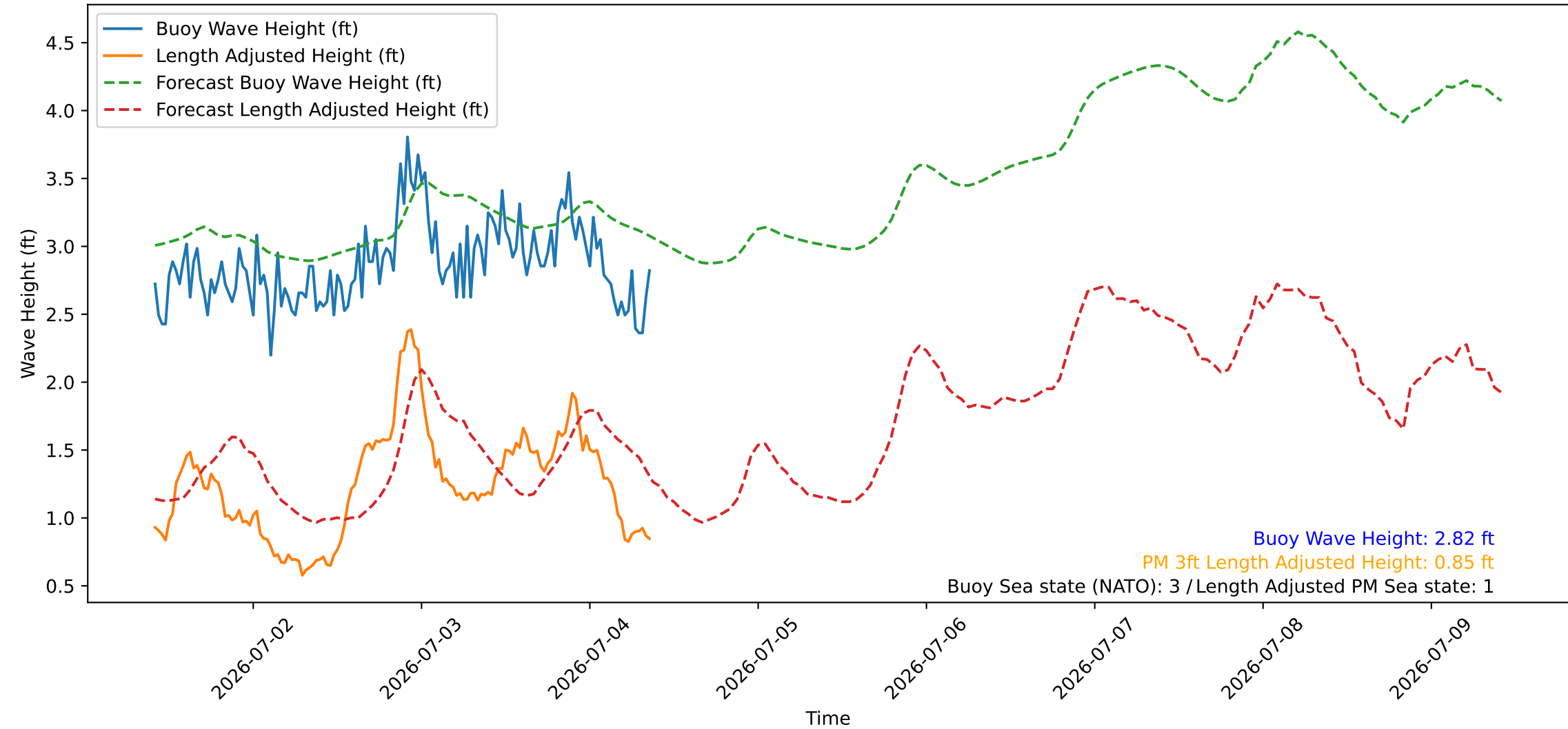
Wave Heights over Time for Red Beach at 2026-07-04 09:30:46
