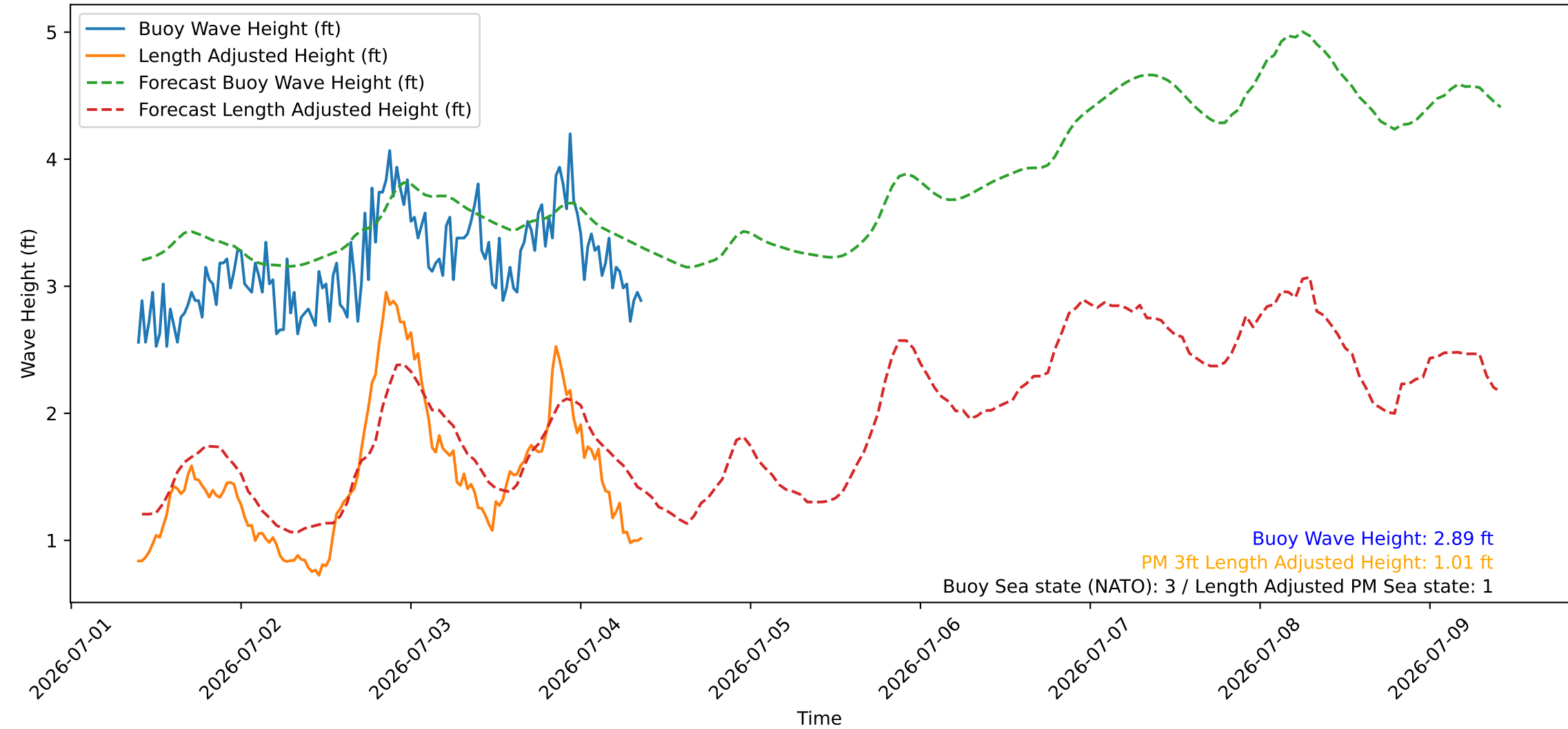
Wave Heights over Time for Green Beach at 2026-07-04 09:31:09
