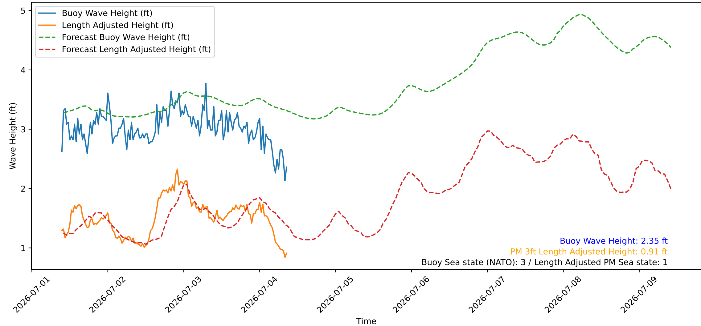
Wave Heights over Time for Oceanside Harbor at 2026-07-04 09:30:27
