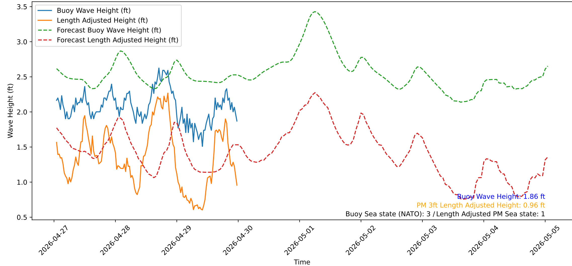
Wave Heights over Time for Red Beach at 2026-04-30 00:30:50
