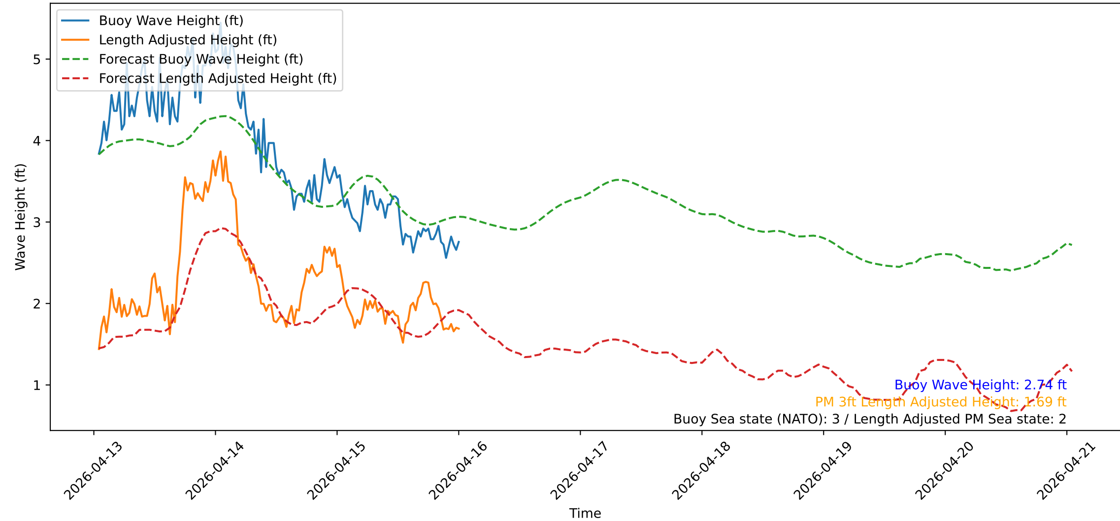
Wave Heights over Time for Oceanside Harbor at 2026-04-16 00:50:31
