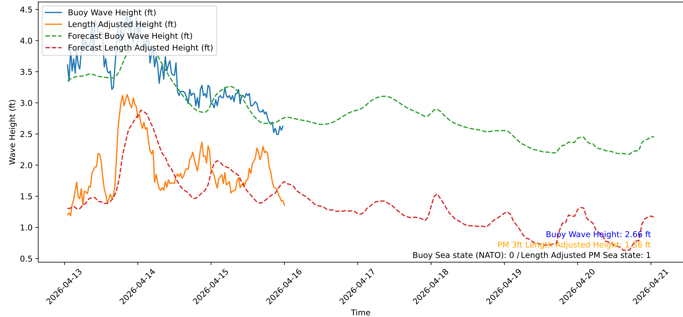
Wave Heights over Time for Red Beach at 2026-04-16 00:50:52
