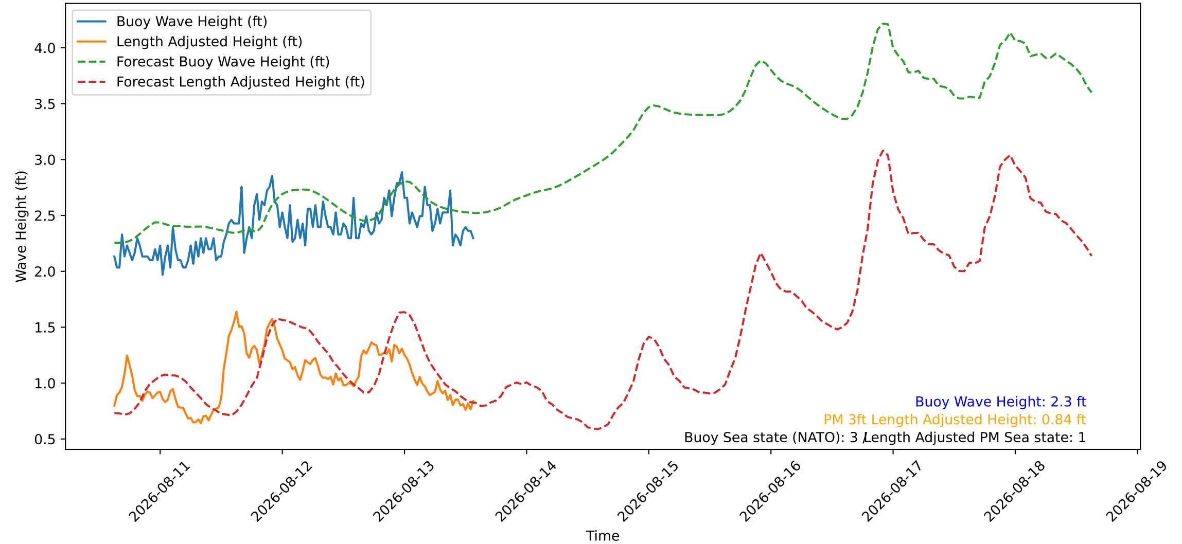
Wave Heights over Time for Red Beach at 2026-08-13 14:30:46
