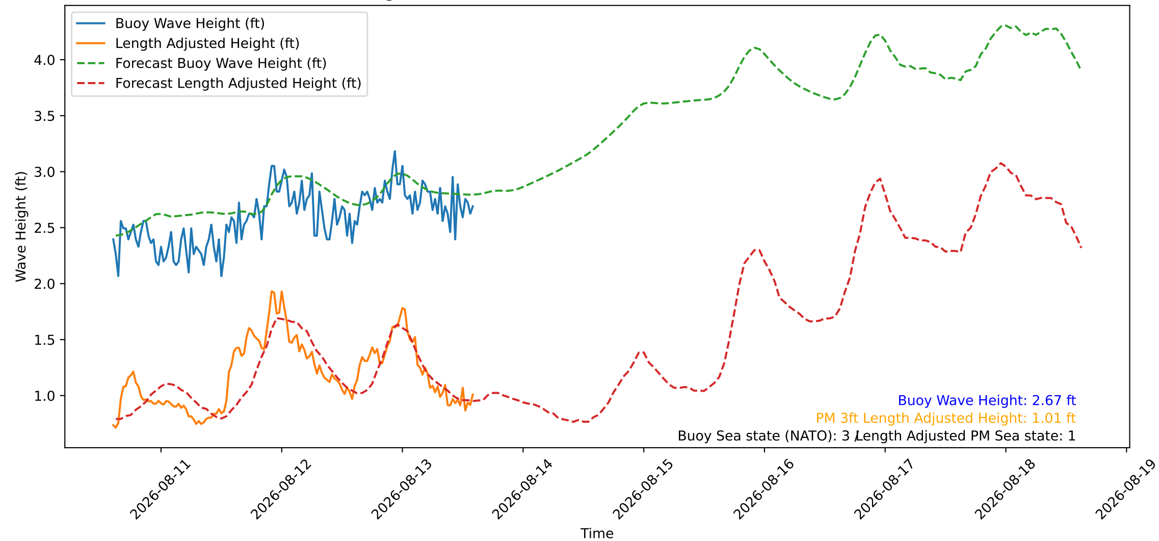
Wave Heights over Time for Oceanside Harbor at 2026-08-13 14:30:27
