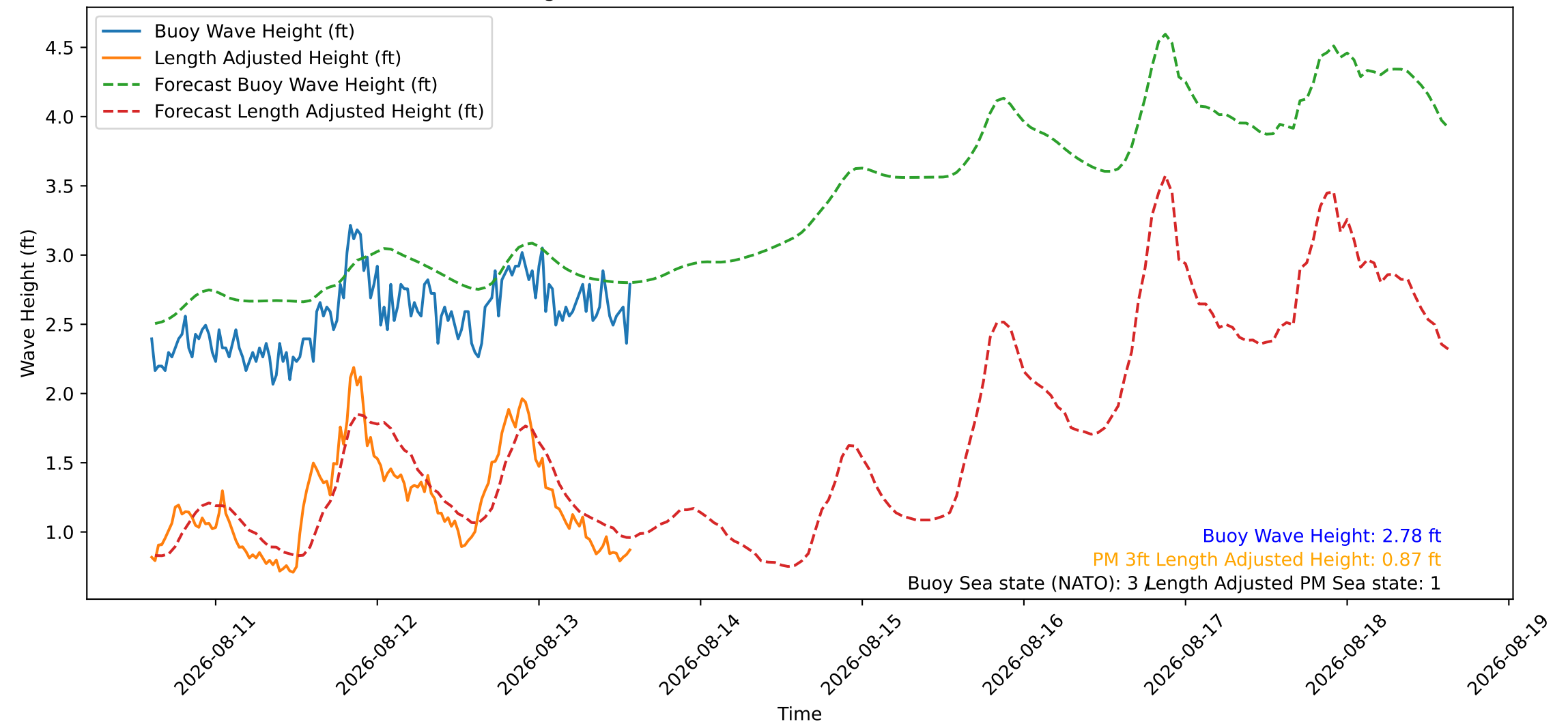
Wave Heights over Time for Green Beach at 2026-08-13 14:31:09
