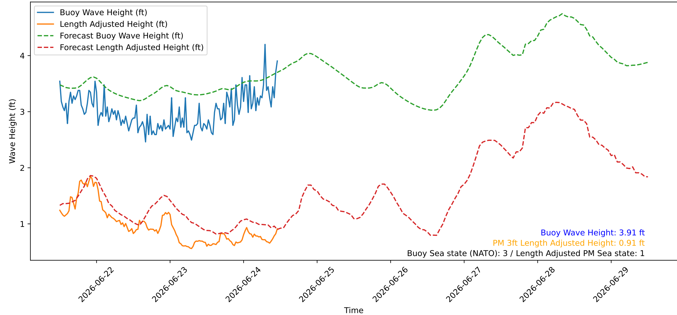
Wave Heights over Time for Green Beach at 2026-06-24 11:51:09
