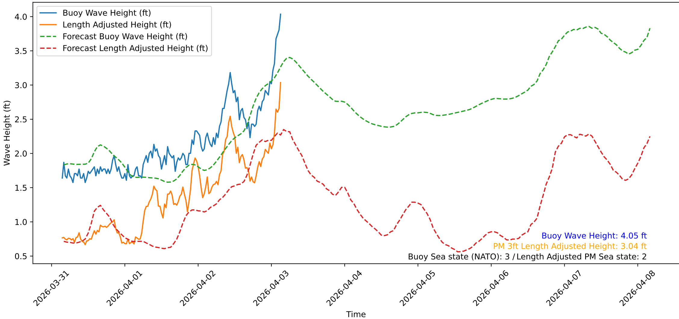
Wave Heights over Time for Oceanside Harbor at 2026-04-03 03:40:31
