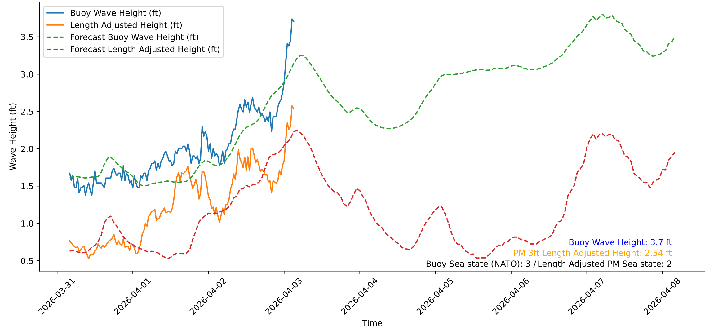
Wave Heights over Time for Red Beach at 2026-04-03 03:40:47
