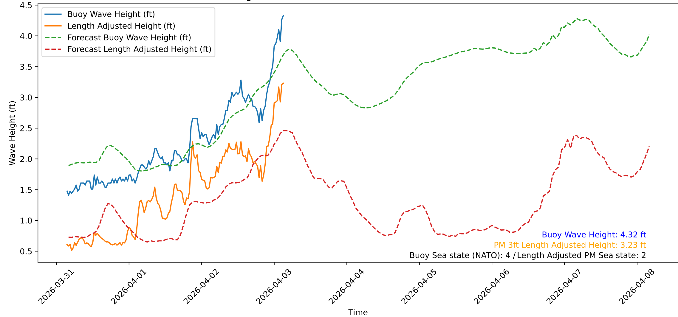
Wave Heights over Time for Green Beach at 2026-04-03 03:41:10
