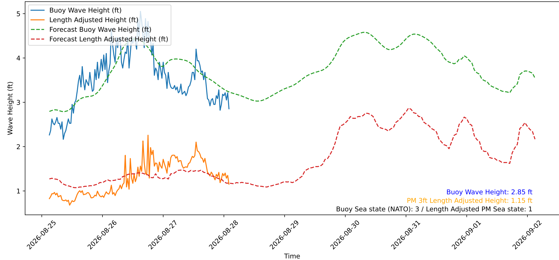
Wave Heights over Time for Red Beach at 2026-08-28 02:40:49
