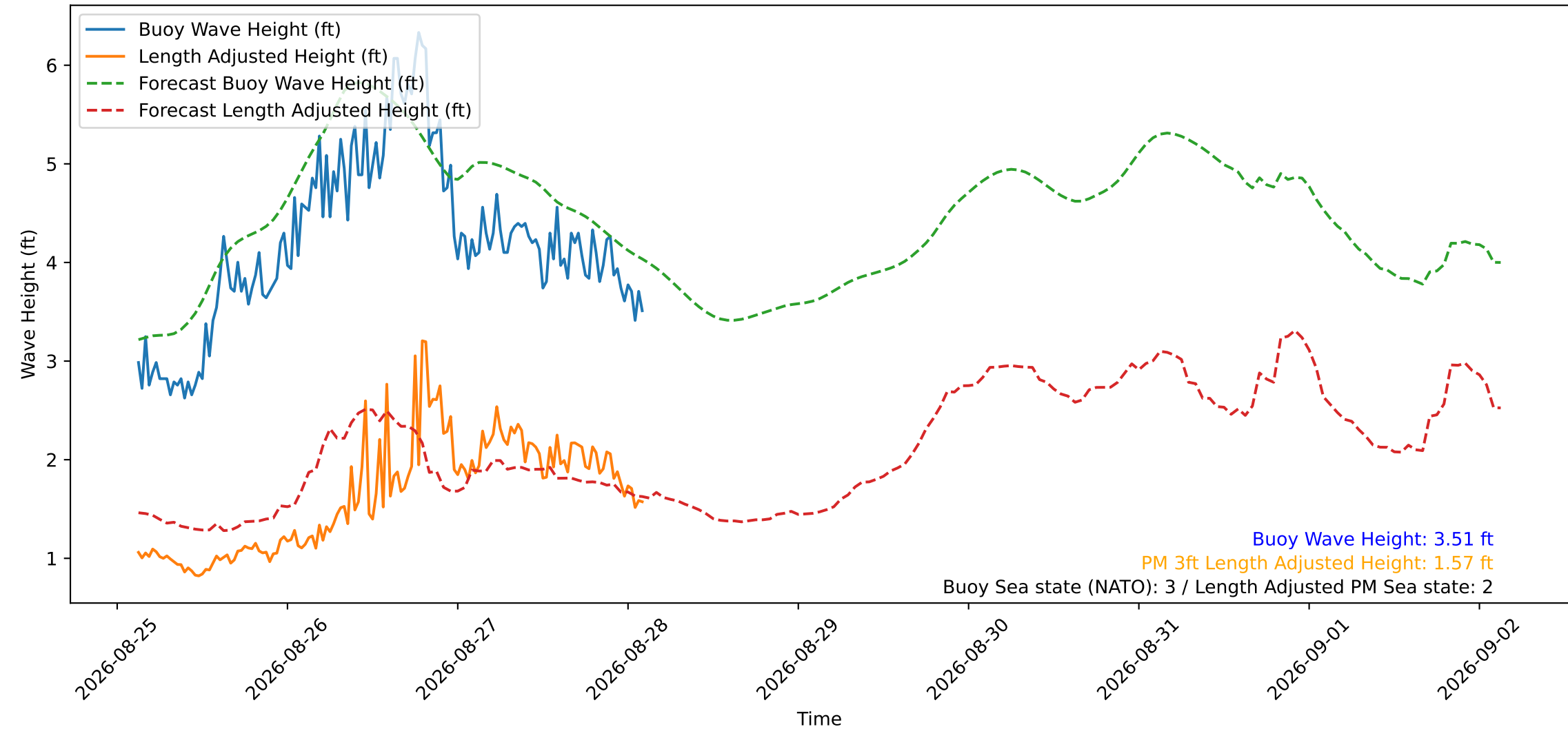
Wave Heights over Time for Green Beach at 2026-08-28 02:41:11
