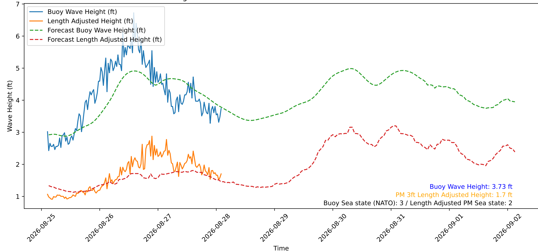
Wave Heights over Time for Oceanside Harbor at 2026-08-28 02:40:29
