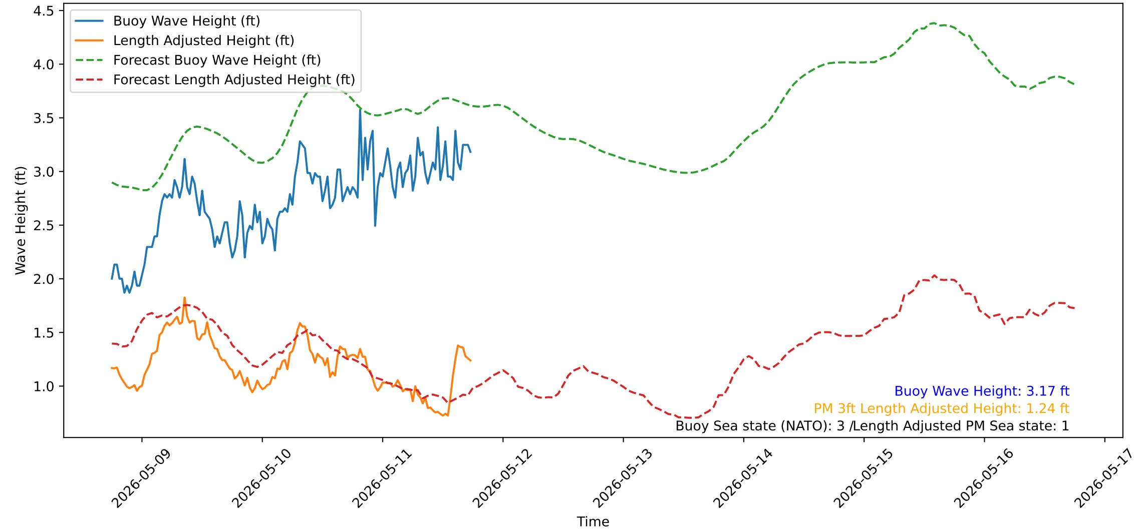
Wave Heights over Time for Oceanside Harbor at 2026-05-11 18:10:31
