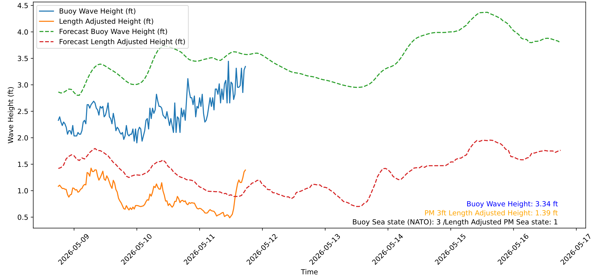
Wave Heights over Time for Green Beach at 2026-05-11 18:11:12
