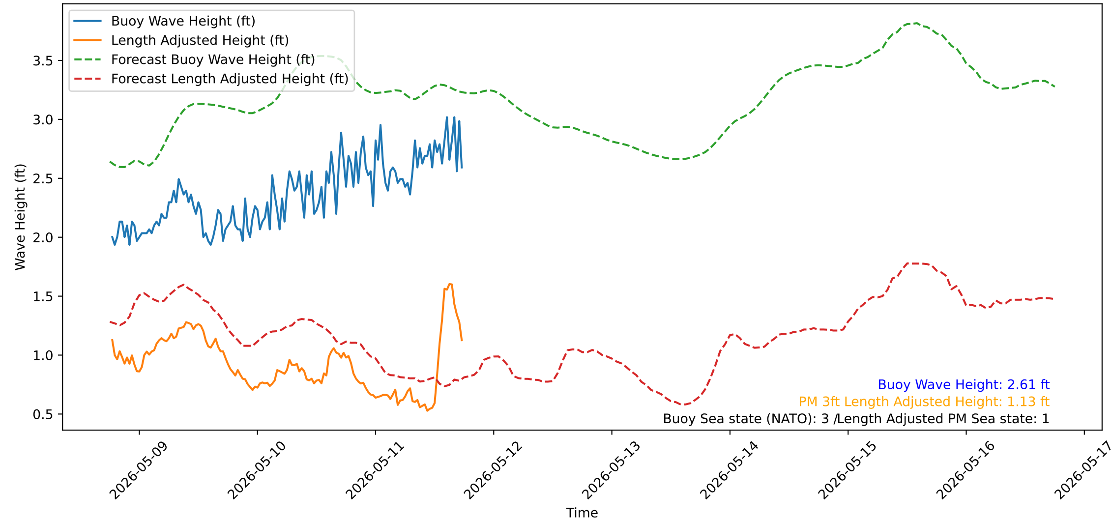
Wave Heights over Time for Red Beach at 2026-05-11 18:10:50
