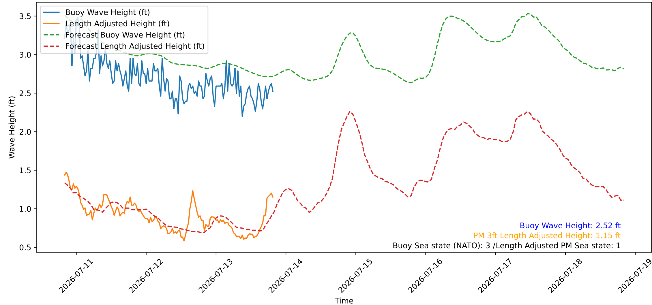
Wave Heights over Time for Green Beach at 2026-07-13 20:11:07
