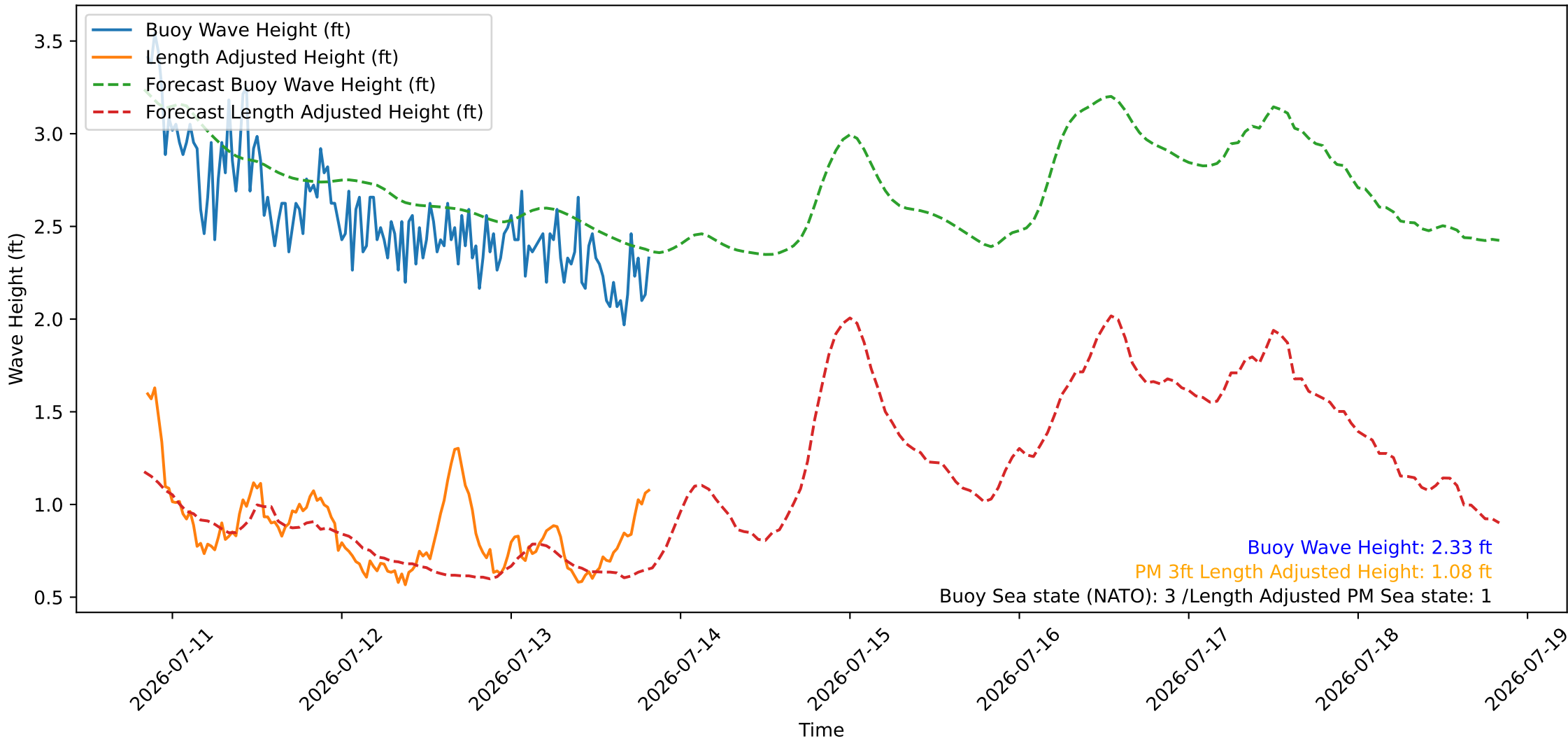
Wave Heights over Time for Red Beach at 2026-07-13 20:10:45
