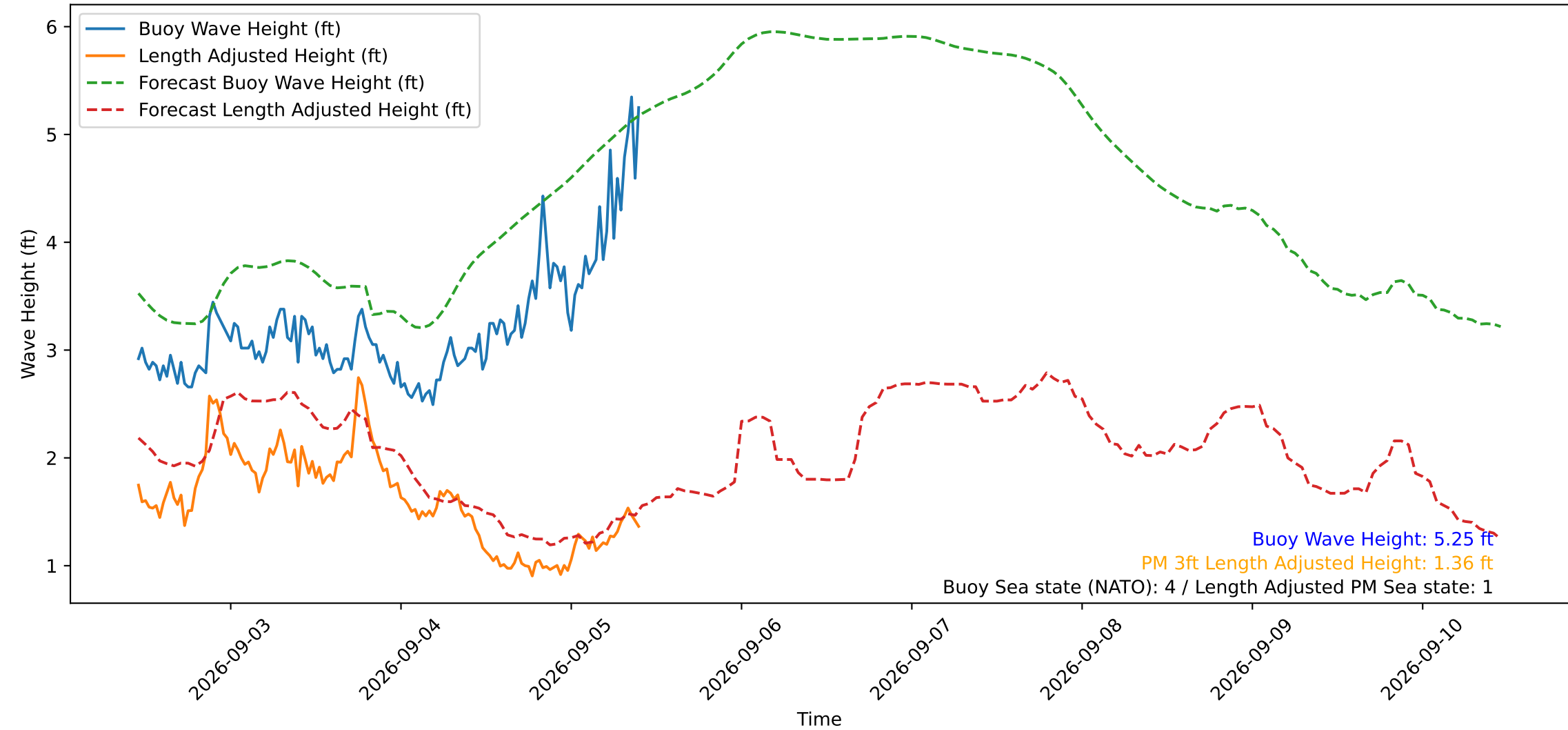
Wave Heights over Time for Green Beach at 2026-09-05 10:31:12
