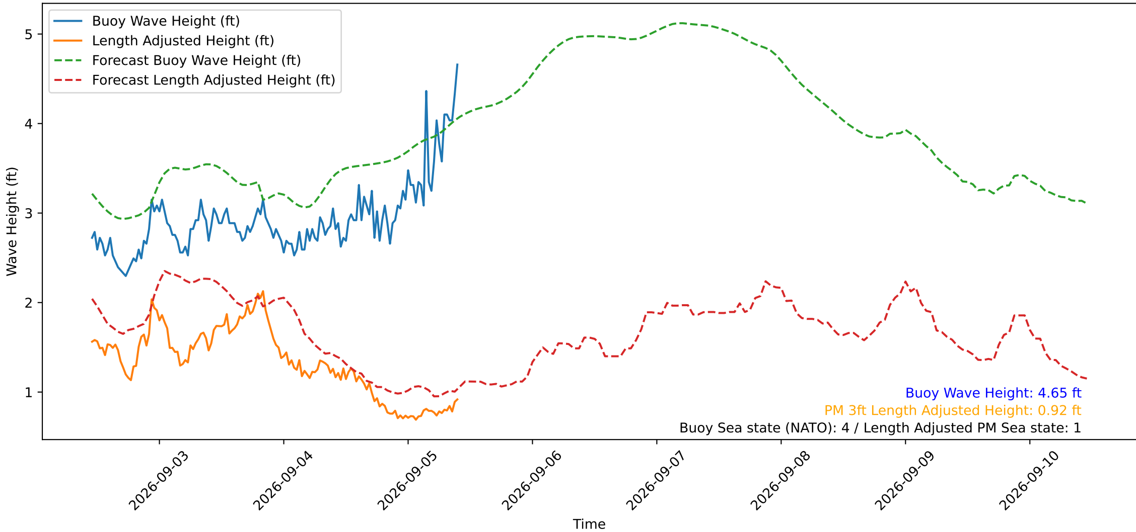
Wave Heights over Time for Red Beach at 2026-09-05 10:30:50
