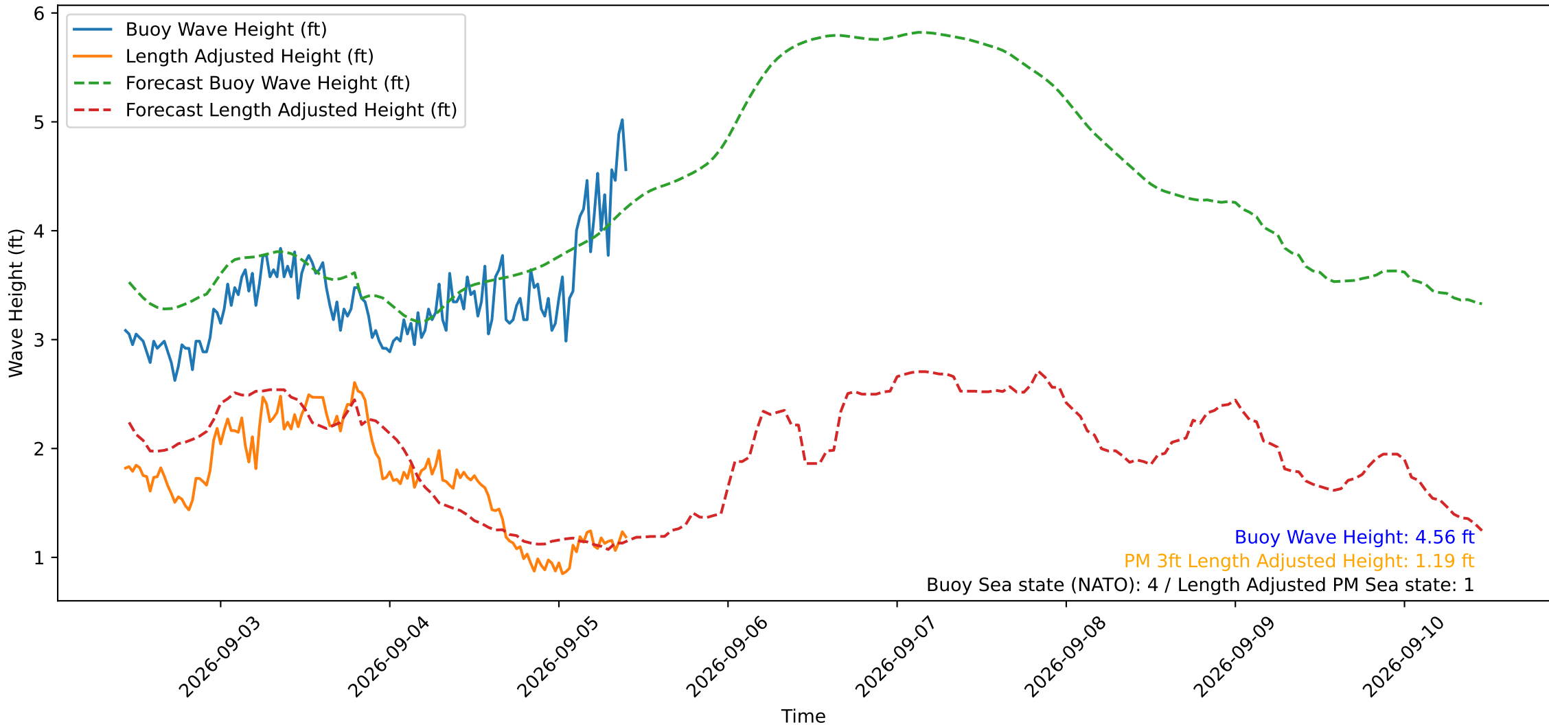
Wave Heights over Time for Oceanside Harbor at 2026-09-05 10:30:30
