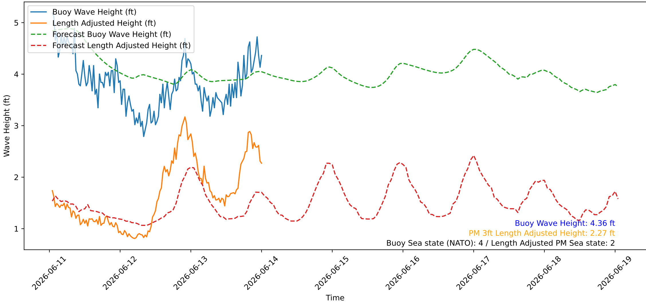
Wave Heights over Time for Oceanside Harbor at 2026-06-14 01:00:27
