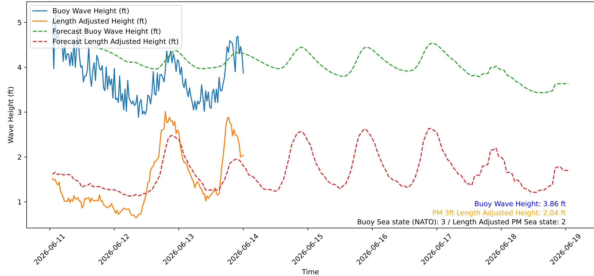
Wave Heights over Time for Green Beach at 2026-06-14 01:01:09
