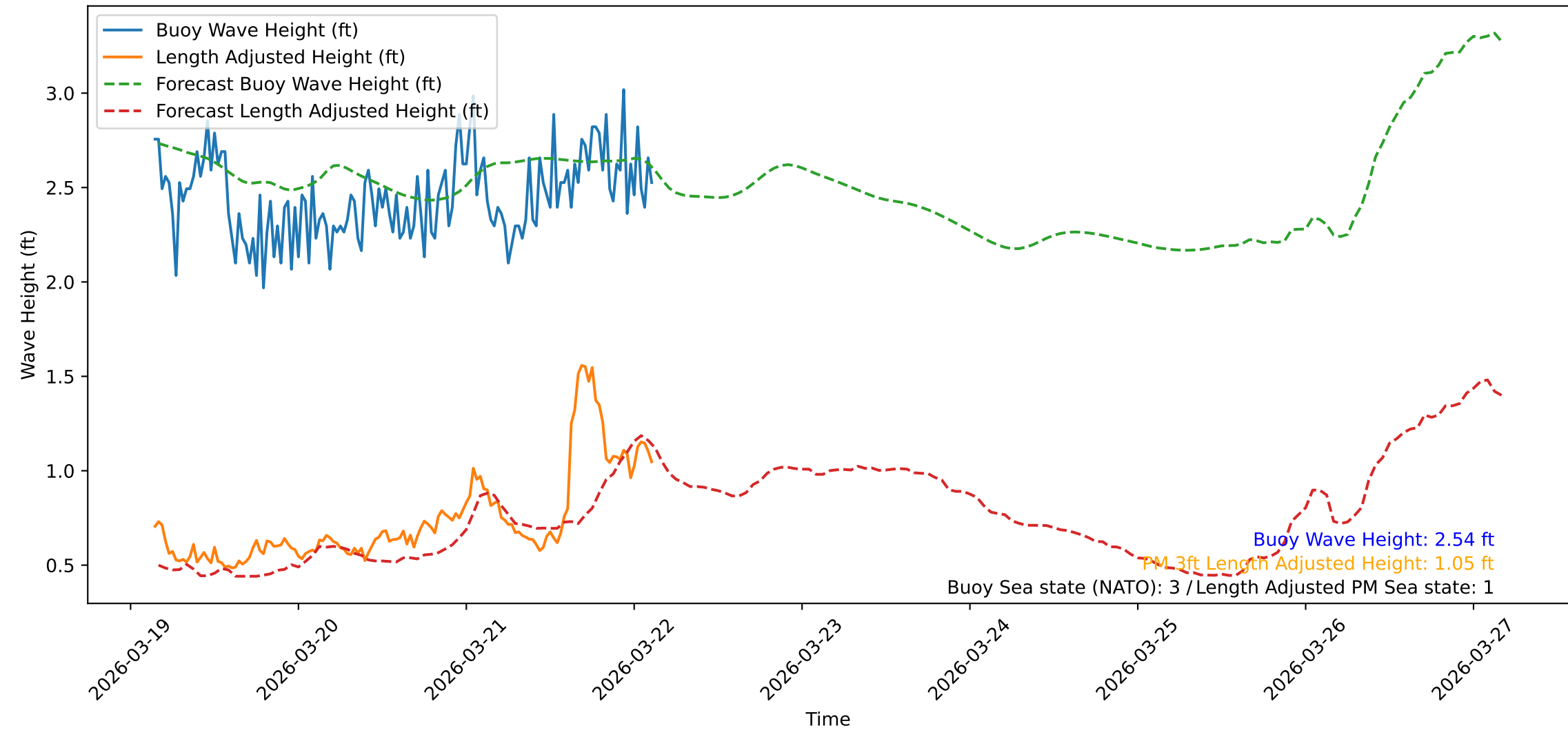
Wave Heights over Time for Oceanside Harbor at 2026-03-22 03:30:31
