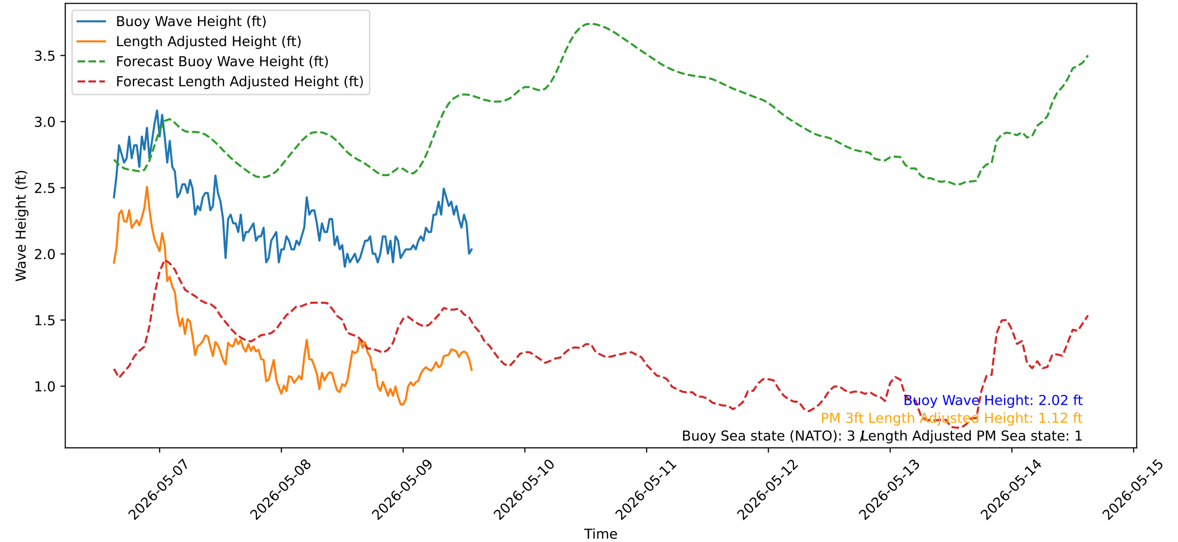
Wave Heights over Time for Red Beach at 2026-05-09 14:30:50
