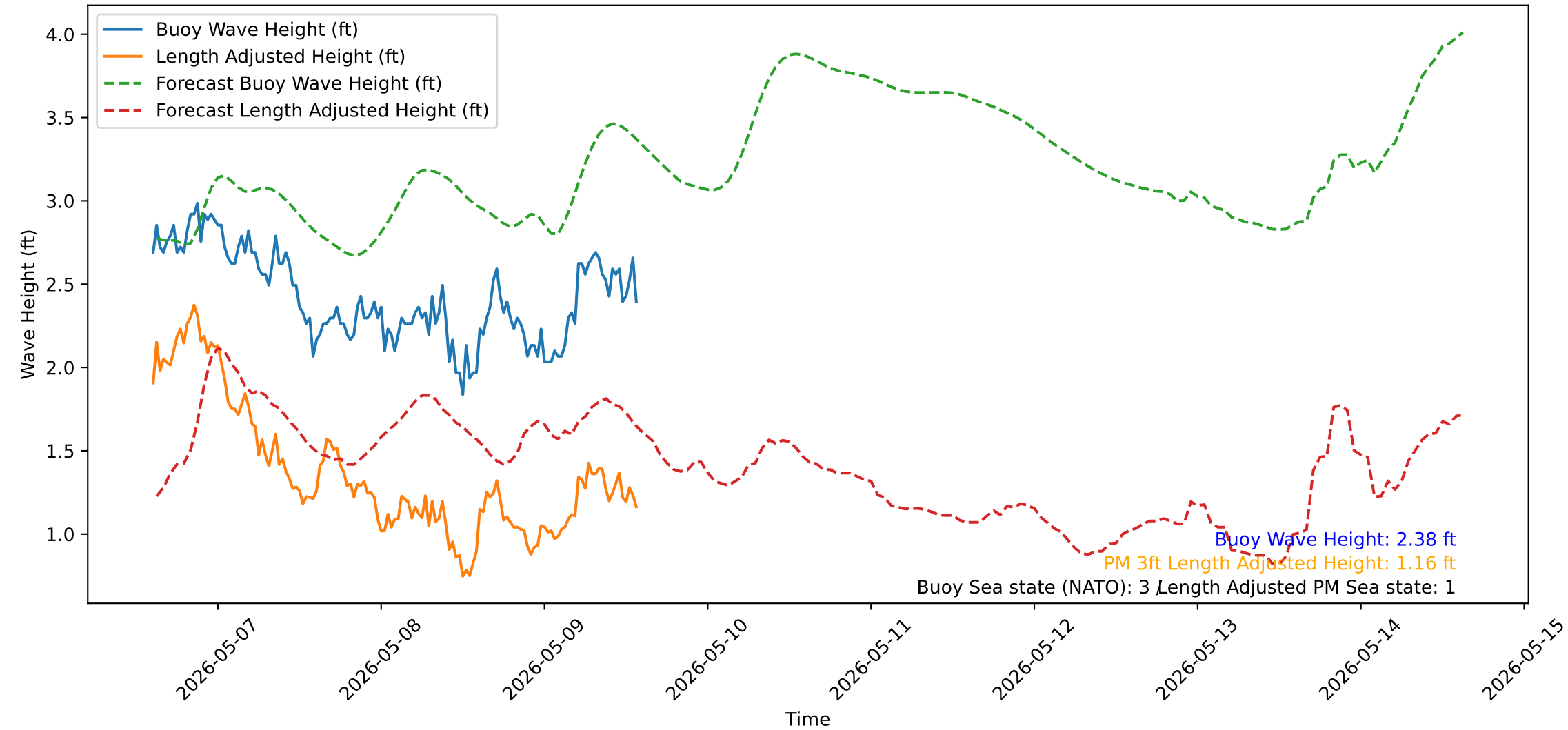
Wave Heights over Time for Green Beach at 2026-05-09 14:31:13
