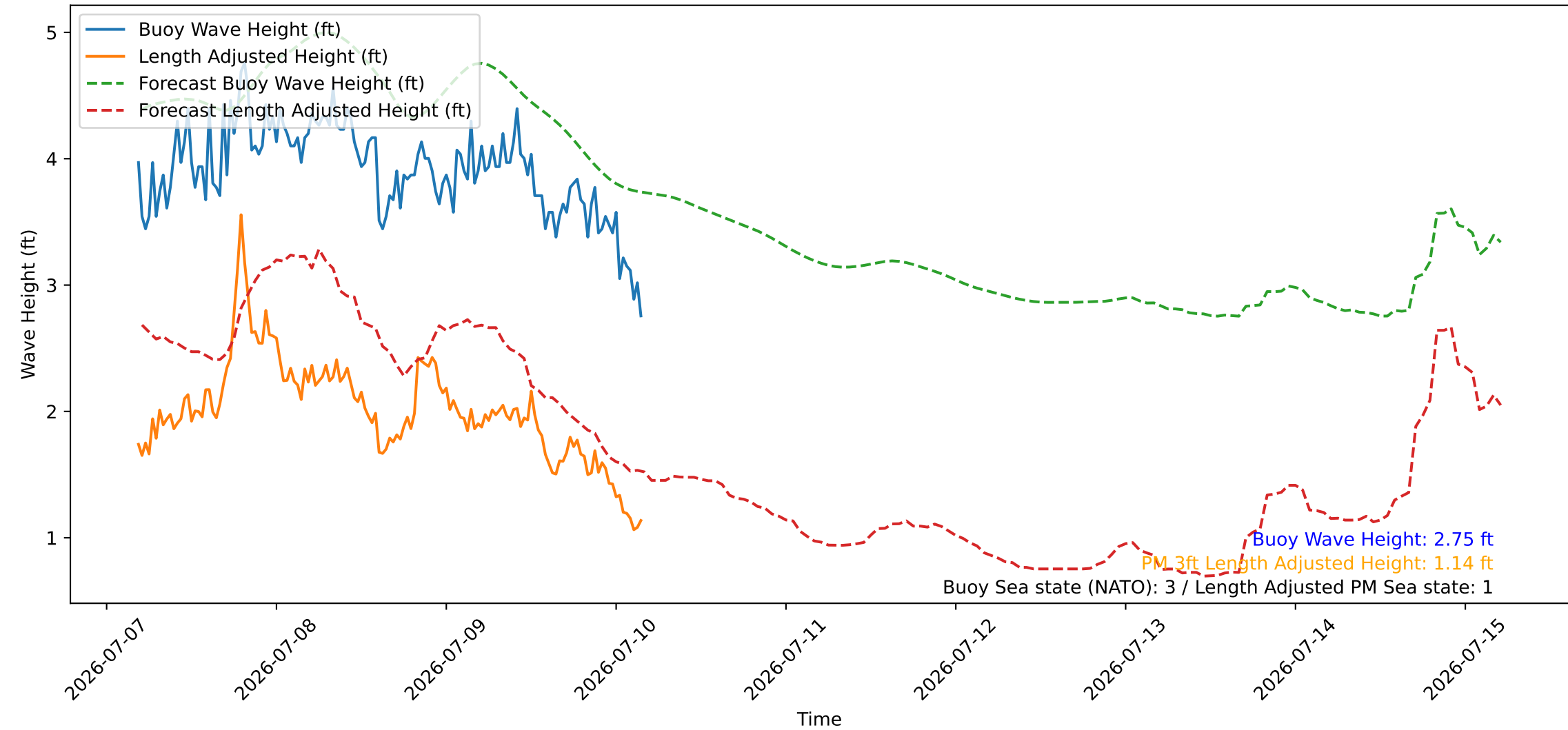
Wave Heights over Time for Green Beach at 2026-07-10 04:31:08
