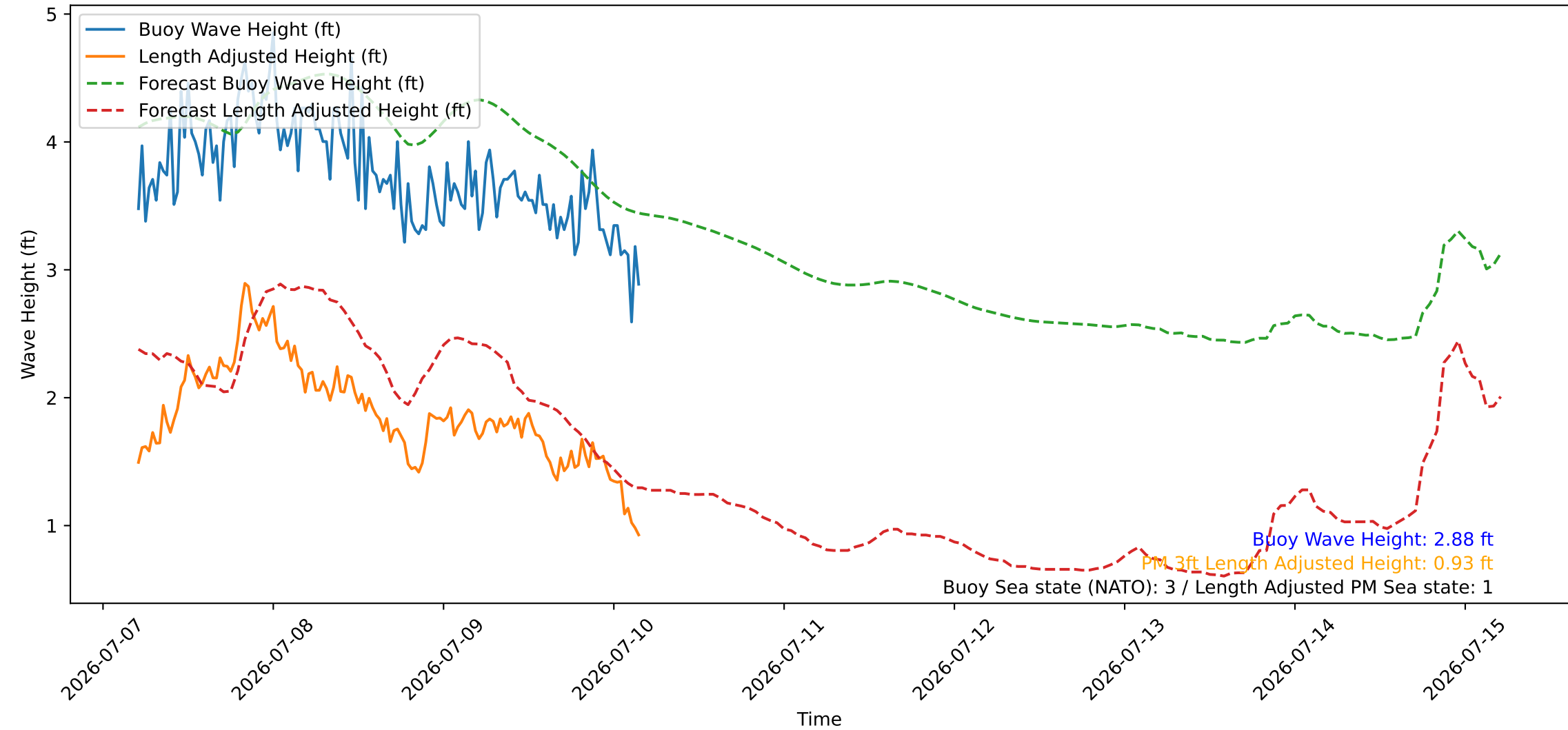
Wave Heights over Time for Red Beach at 2026-07-10 04:30:46
